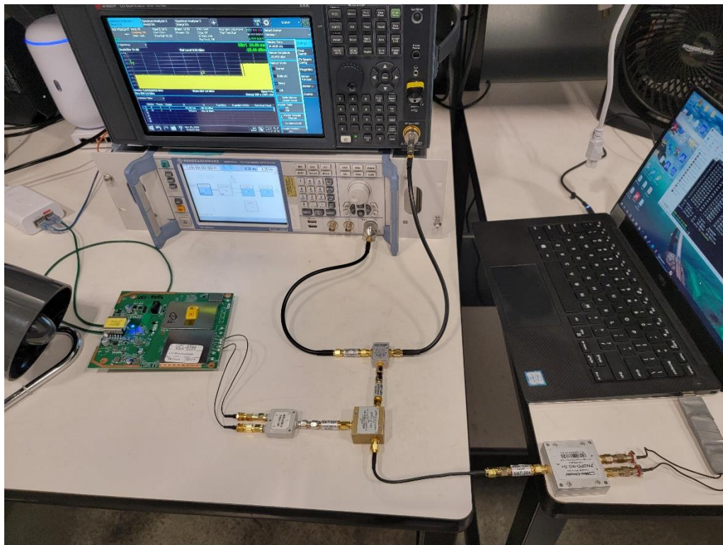
Photograph 5: View Test Set Up DFS
