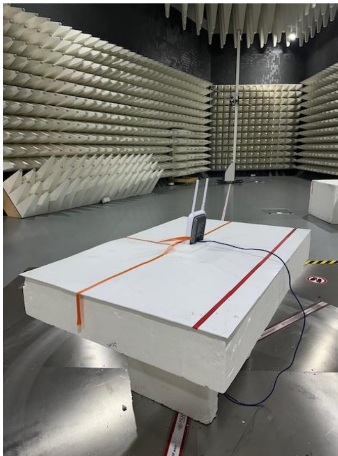
Photograph 1: View Test Set Up Radiated Emissions 30 – 1000 MHz
