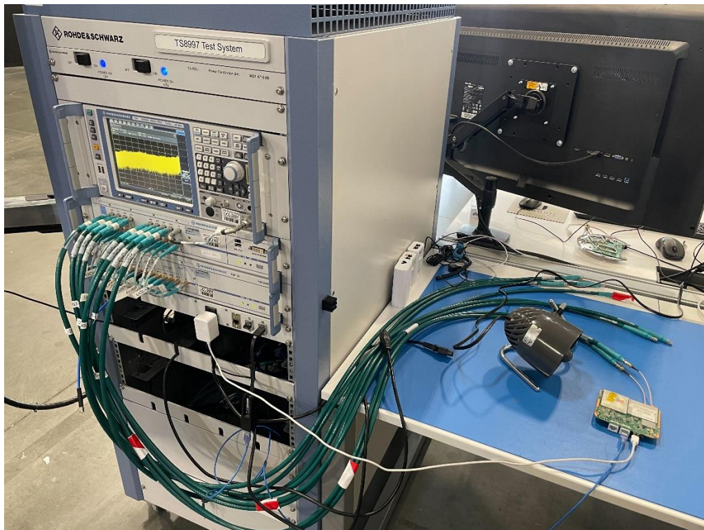
Photograph 4: View Test Set Up RF Conducted
