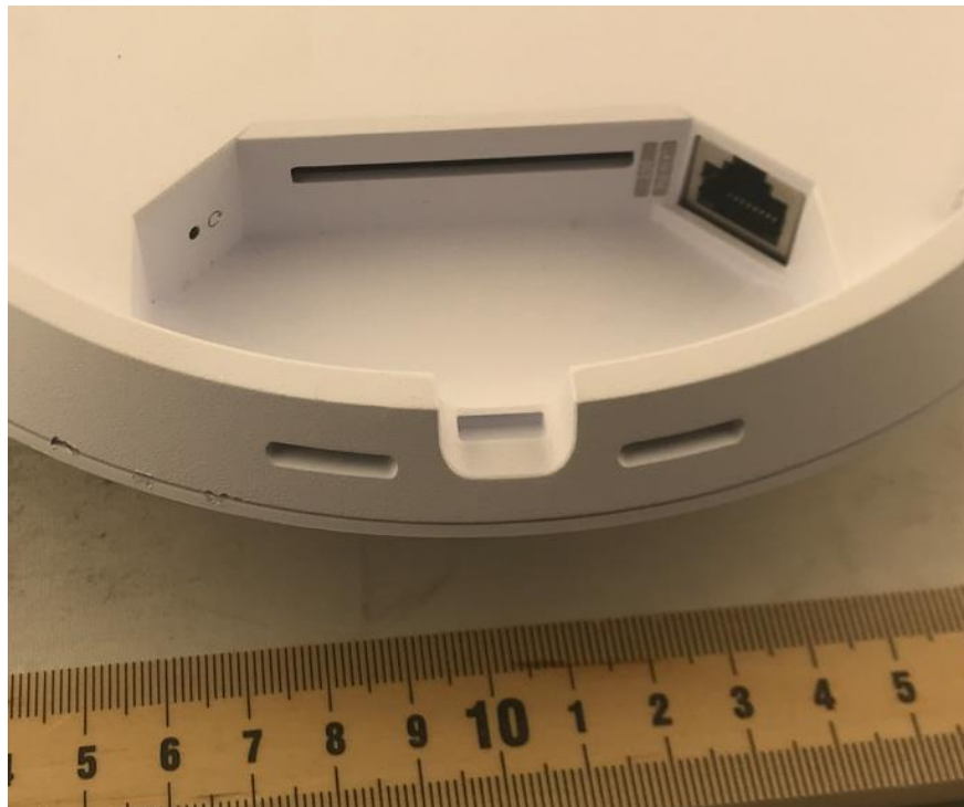
Photograph 8: PoE/LAN port on DUT
