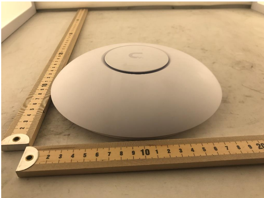
Photograph 4: Right View of DUT
