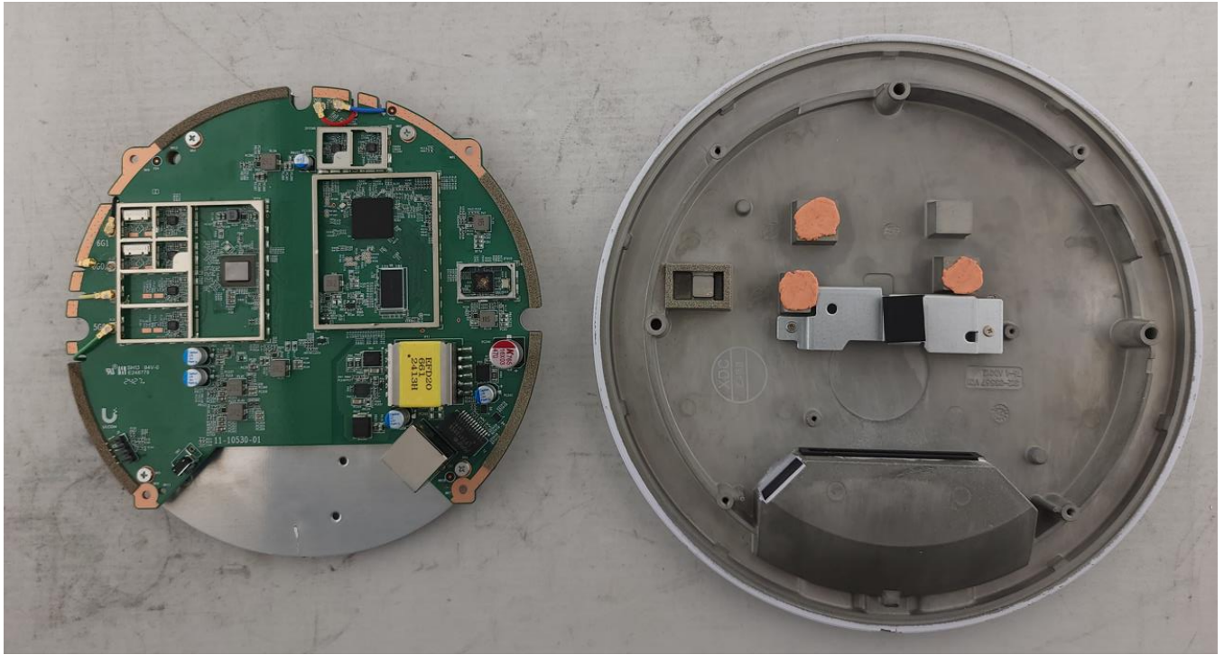
Photograph 3: Bottom Base Internal View of DUT with PCB Off
