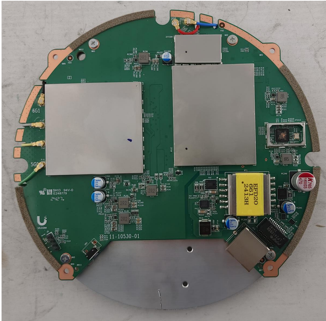
Photograph 4: Top View of the PCB with Cans On
