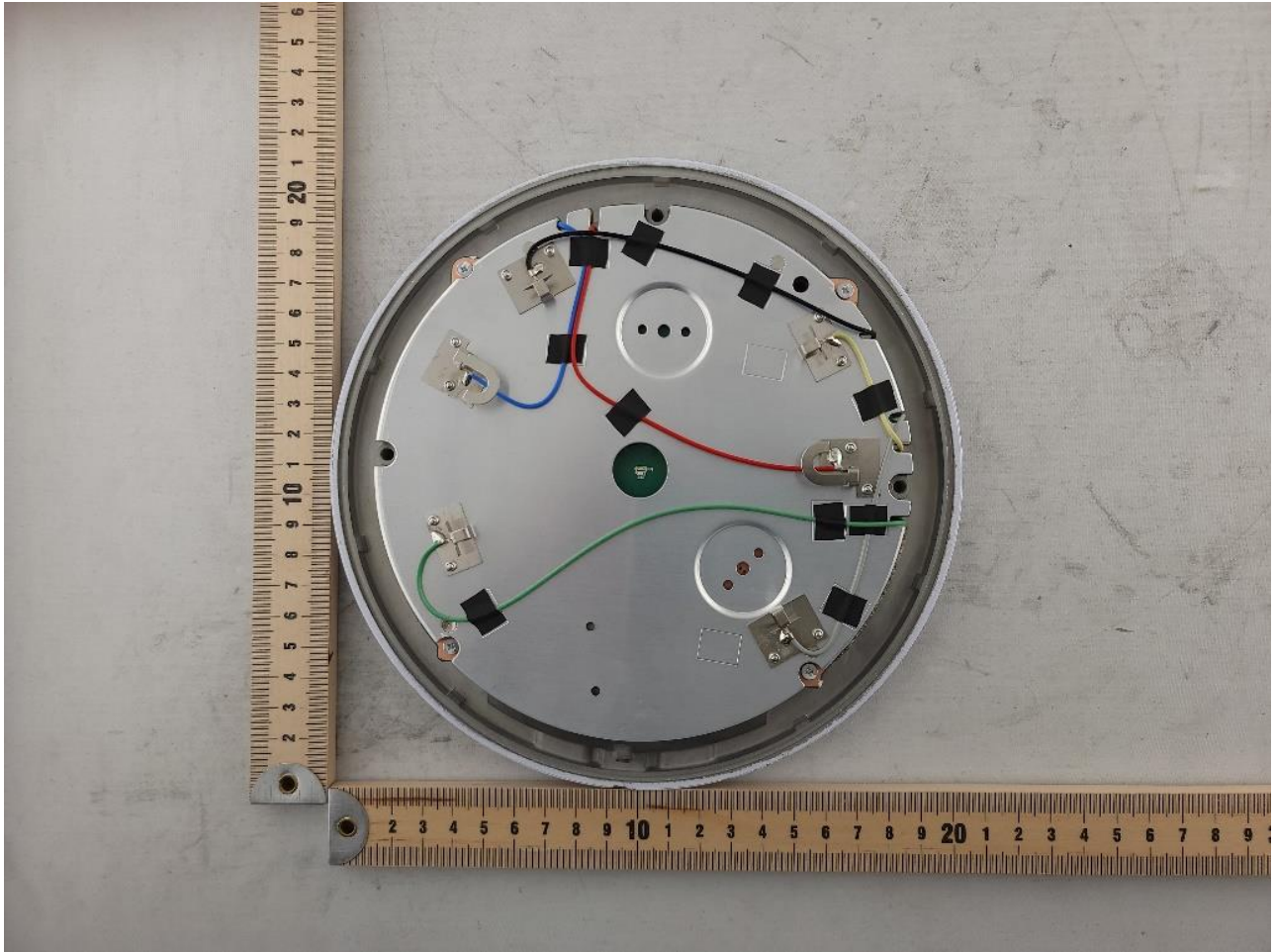
Photograph 2: Internal View of DUT Antenna Board
