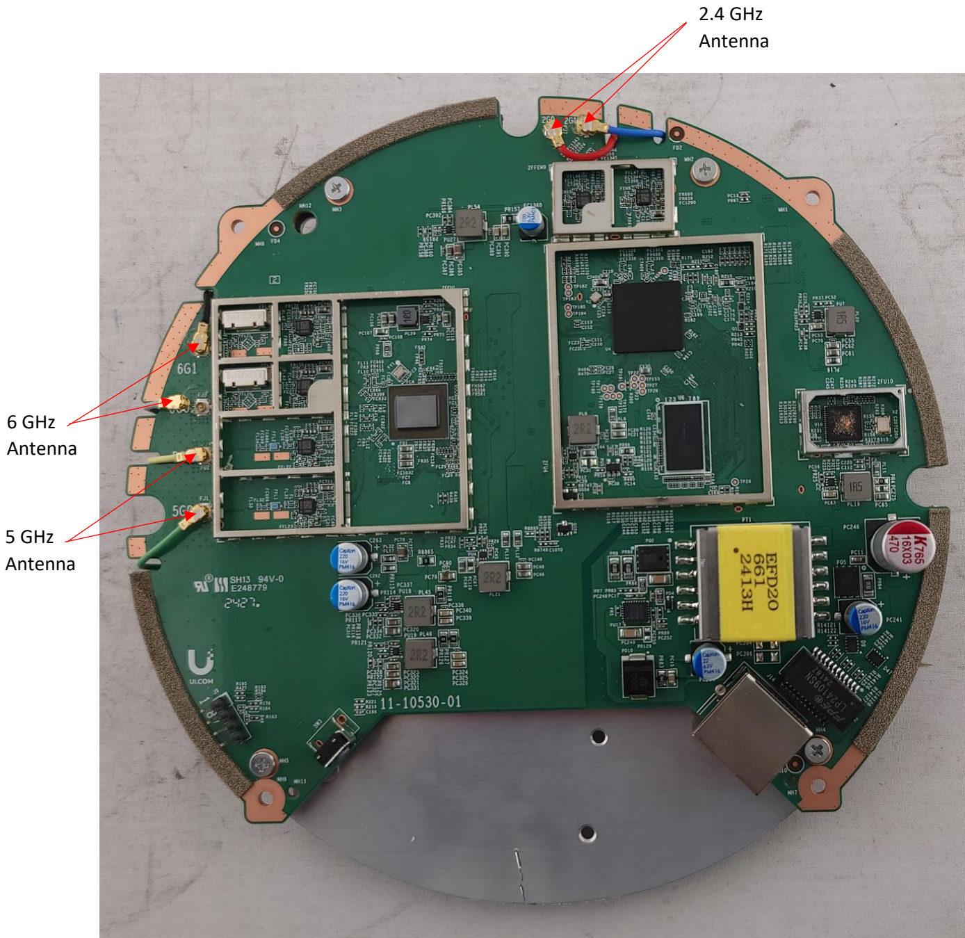
Photograph 1: Top View of the PCB with Cans Off
