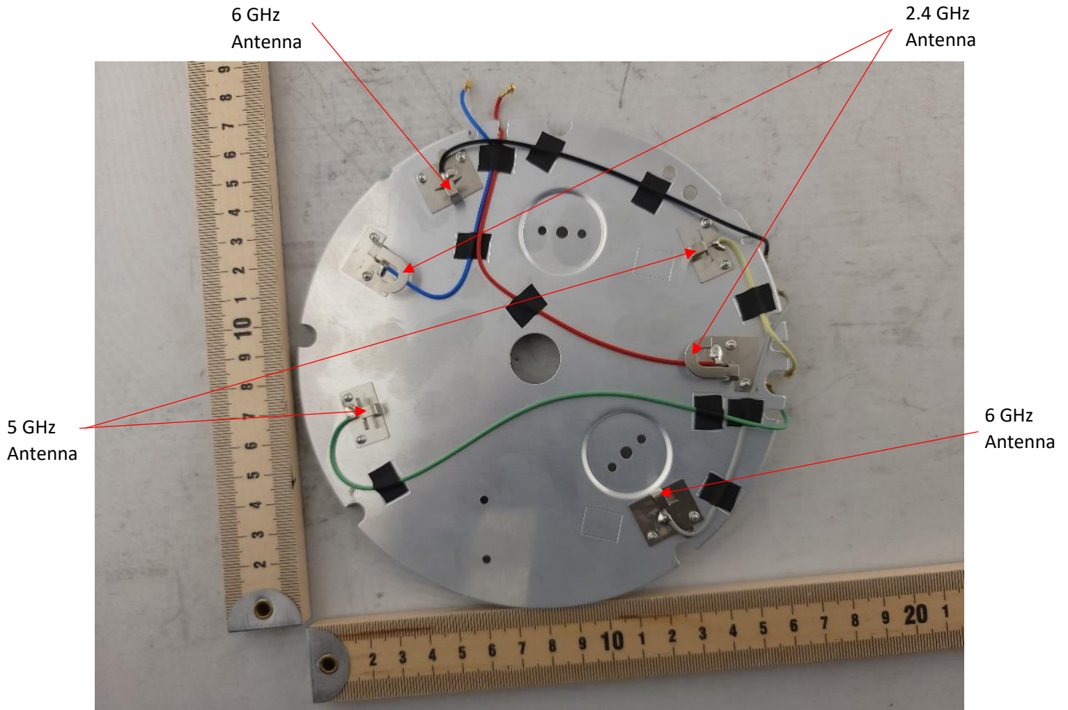
Photograph 3: Top View of the Antenna Configuration
