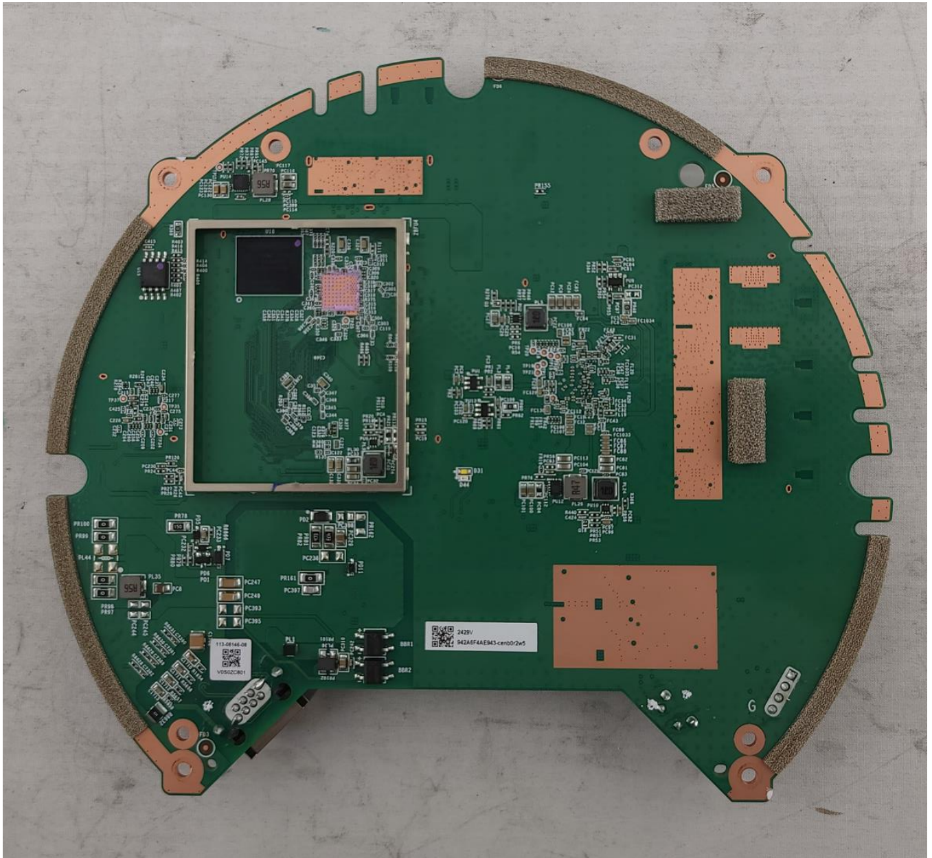
Photograph 2: Bottom View of the PCB Can Off
