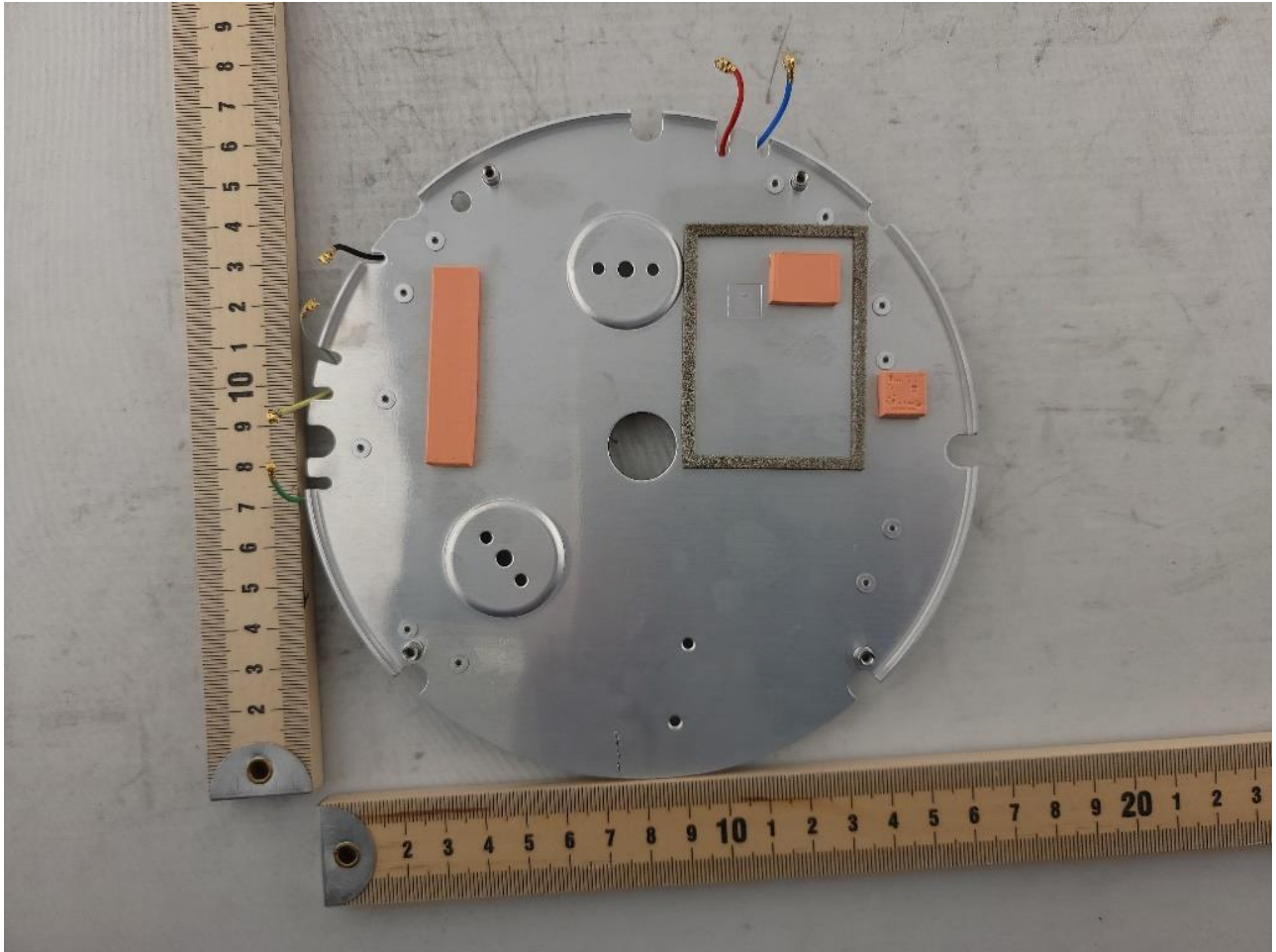
Photograph 4: Bottom View of the Antenna Configuration
