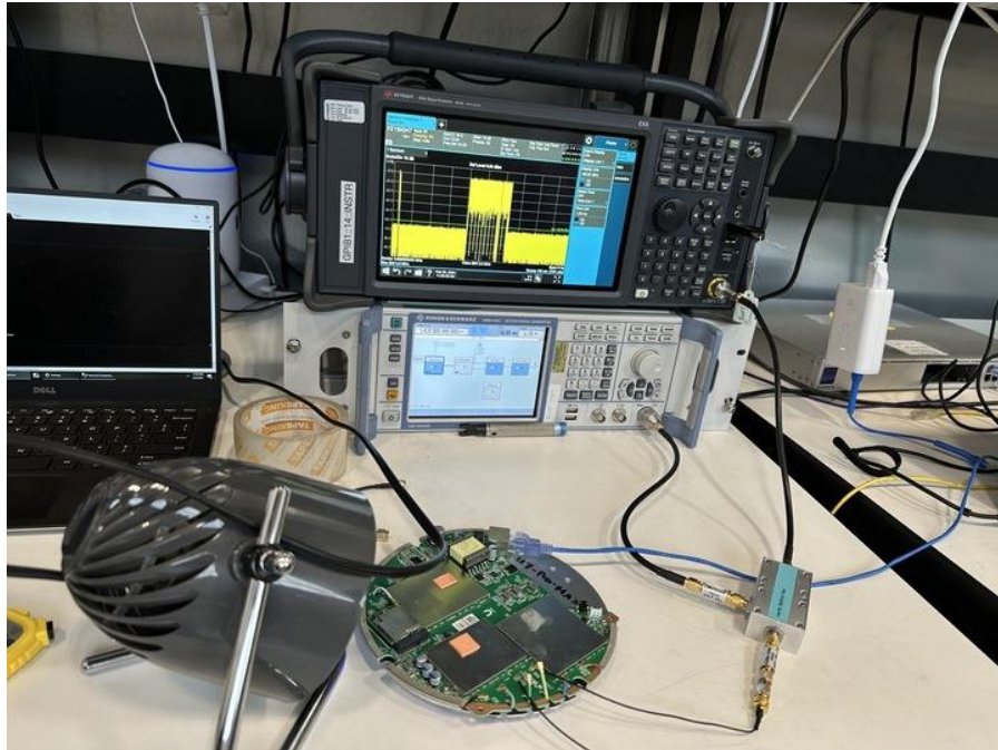
Photograph 7: View Test Set Up DFS
