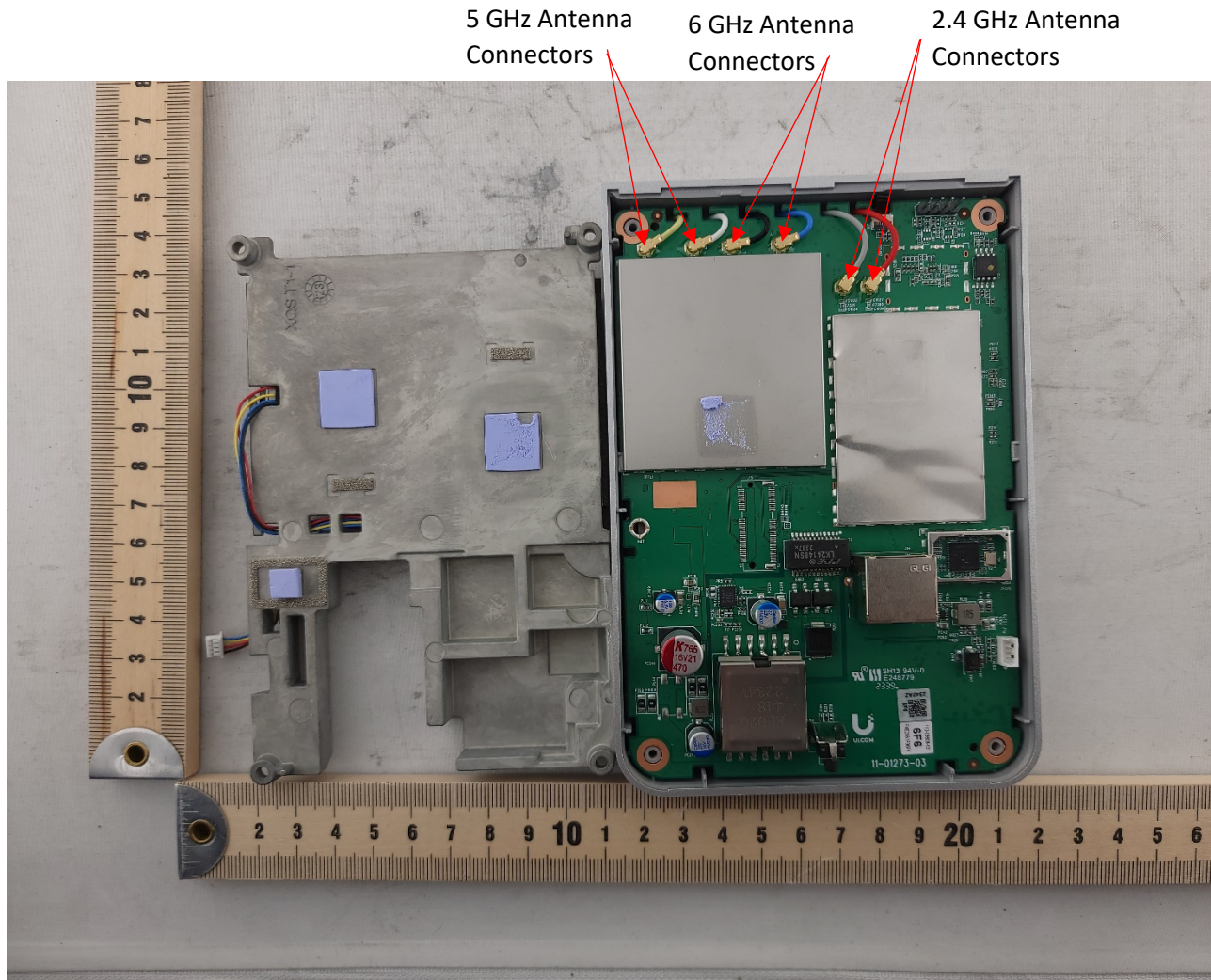
Photograph 2: Internal View with Fan Mount Removed
