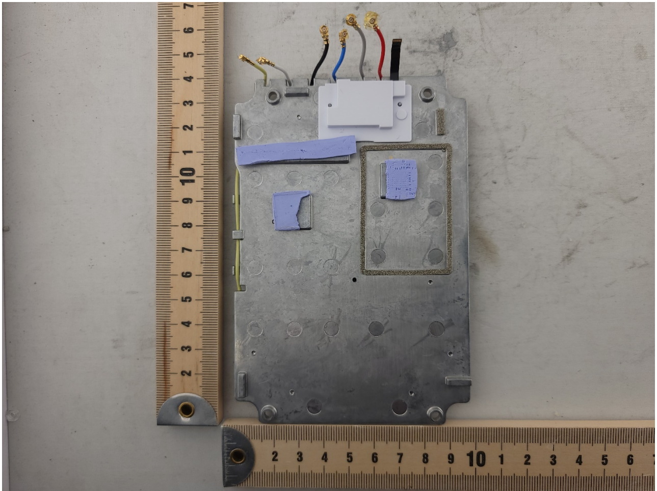
Photograph 6: Back View of Antenna Board
