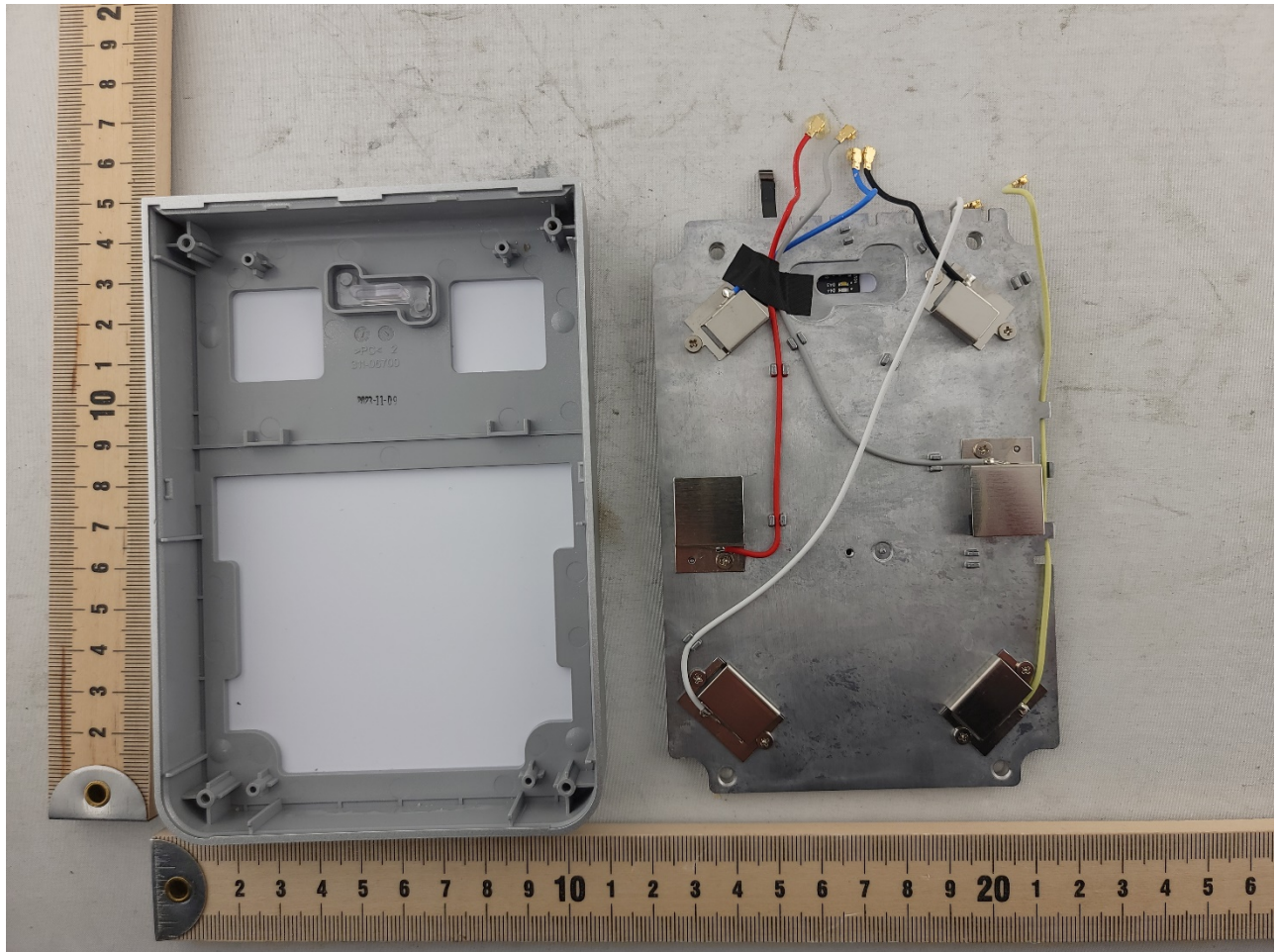
Photograph 4: Internal View with Antenna Board Removed
