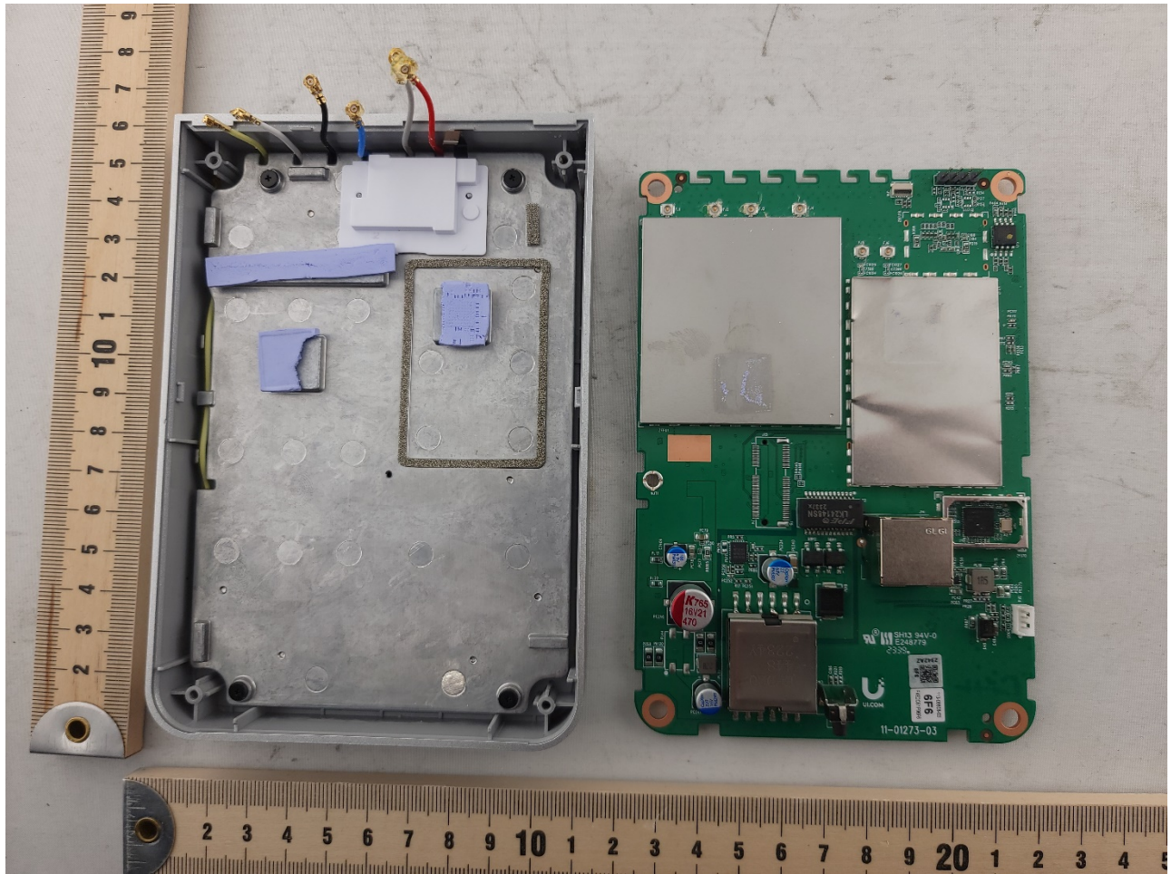
Photograph 3: Internal View with Main PCB Removed
