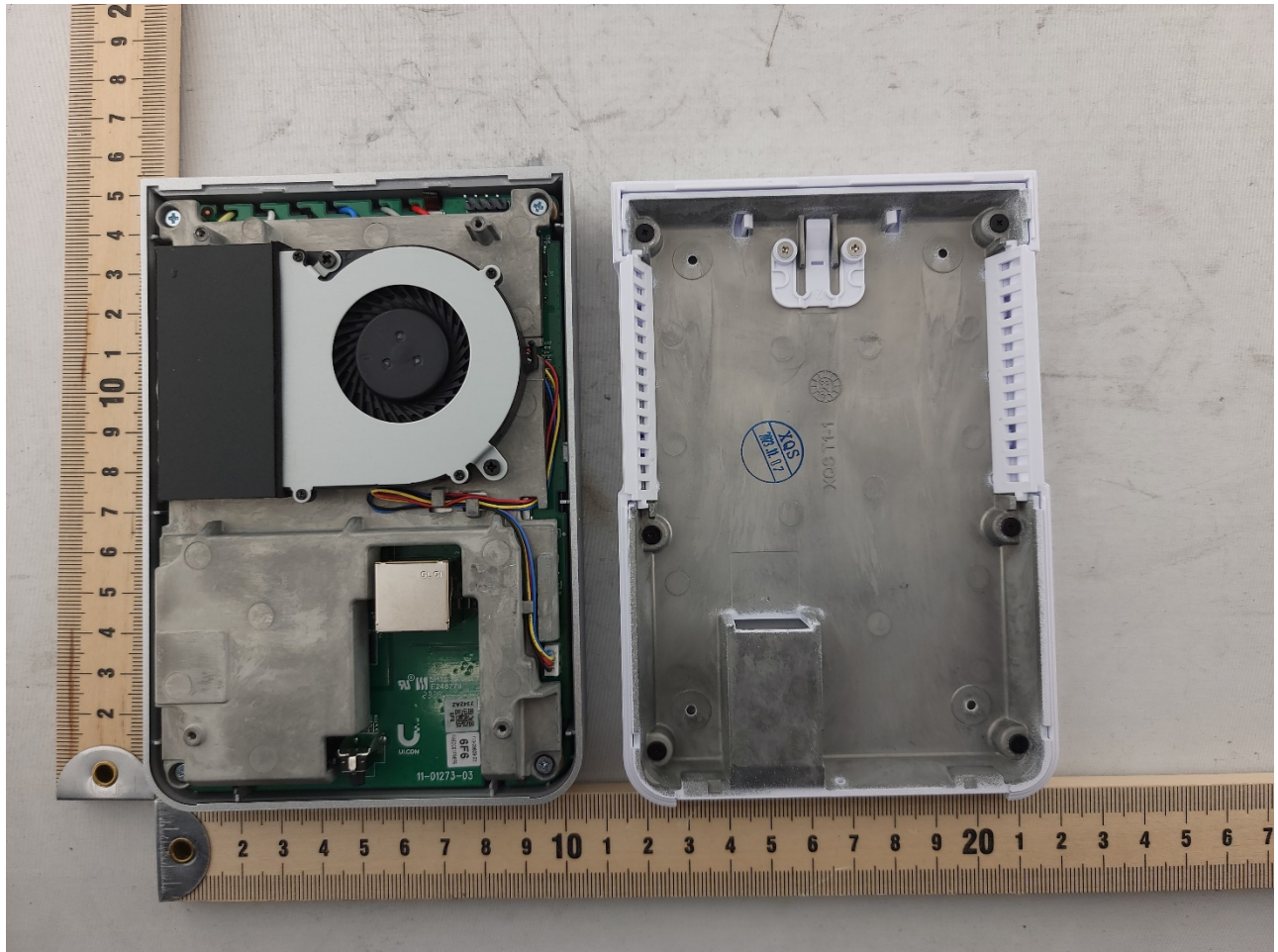
Photograph 1: Internal View with Back Cover Off
