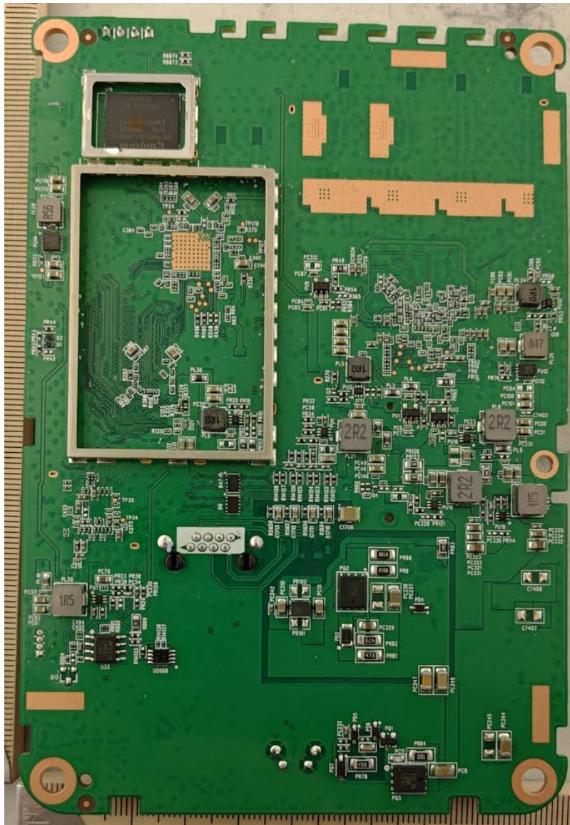
Photograph 3: Close Up of Bottom Main PCB
