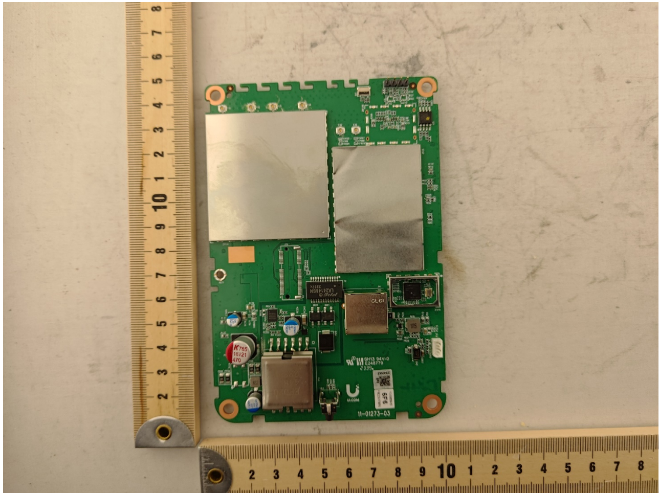
Photograph 1: Front Main PCB with RF Cans On
