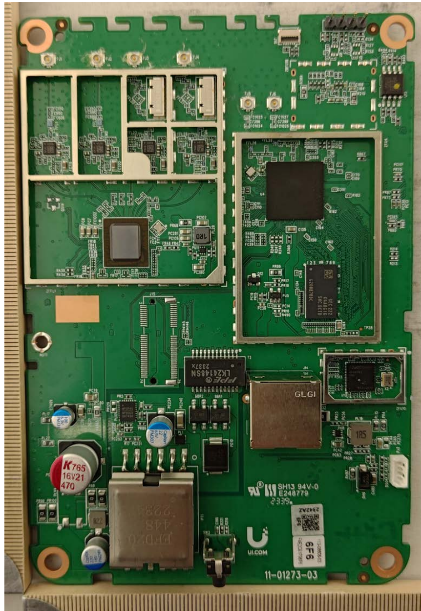
Photograph 2: Close Up of Front Main PCB
