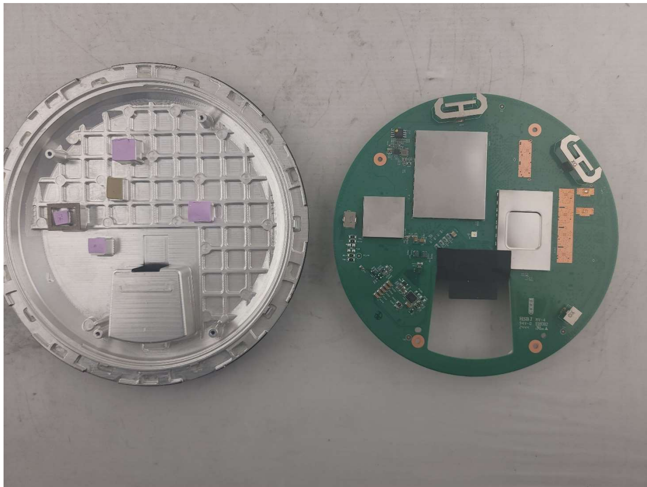
Photograph 3: Internal View of DUT PCB Out of Back Enclosure
