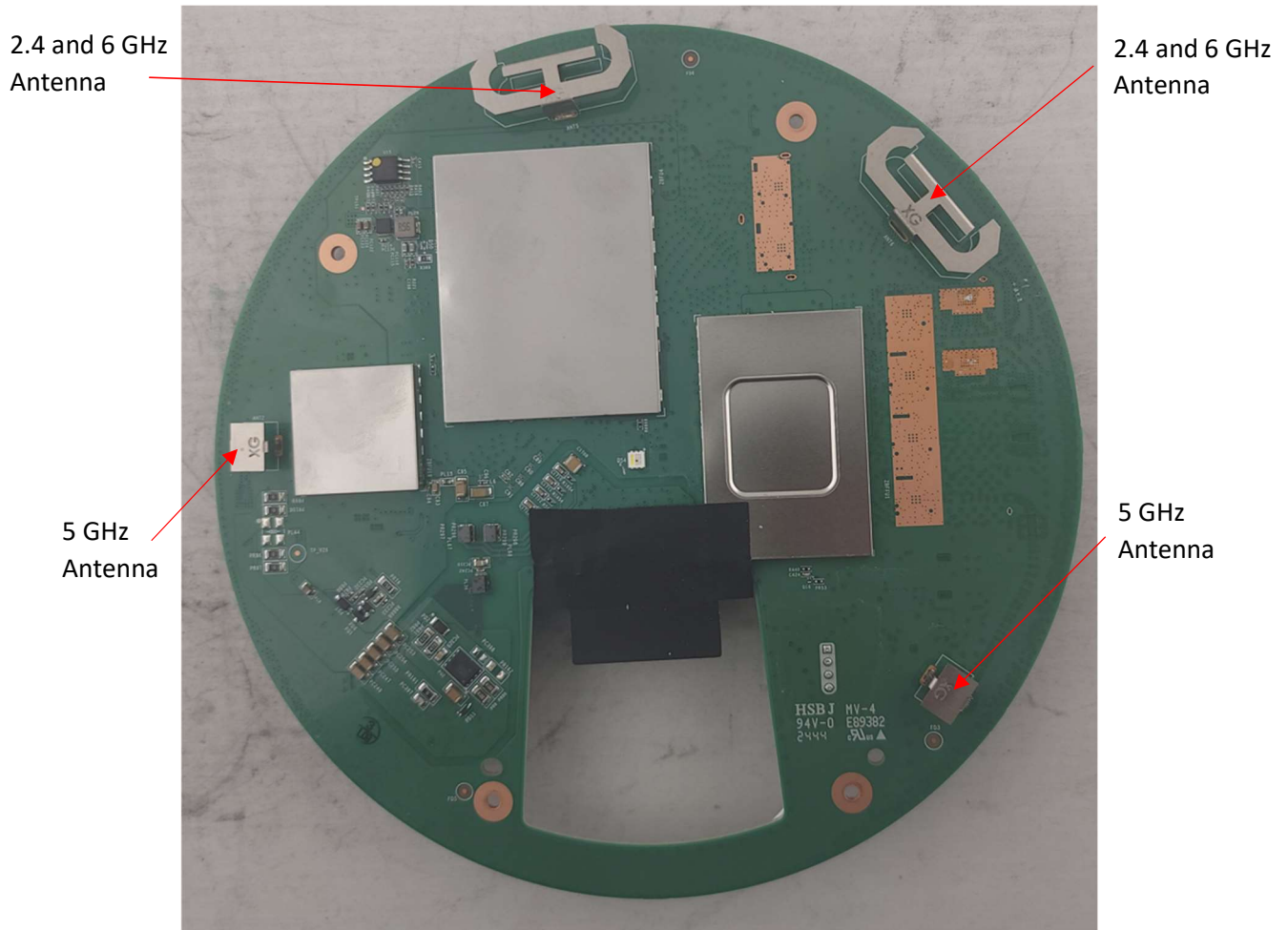
Photograph 5: Front Side of PCB with Cans On
