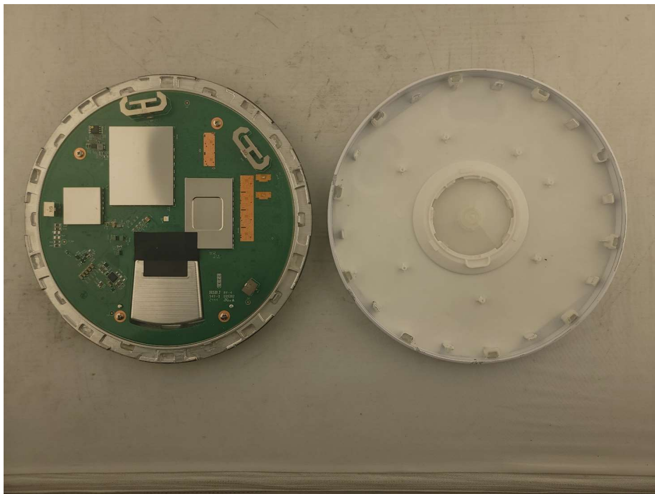
Photograph 1: Internal View of DUT with Front Cover Off
