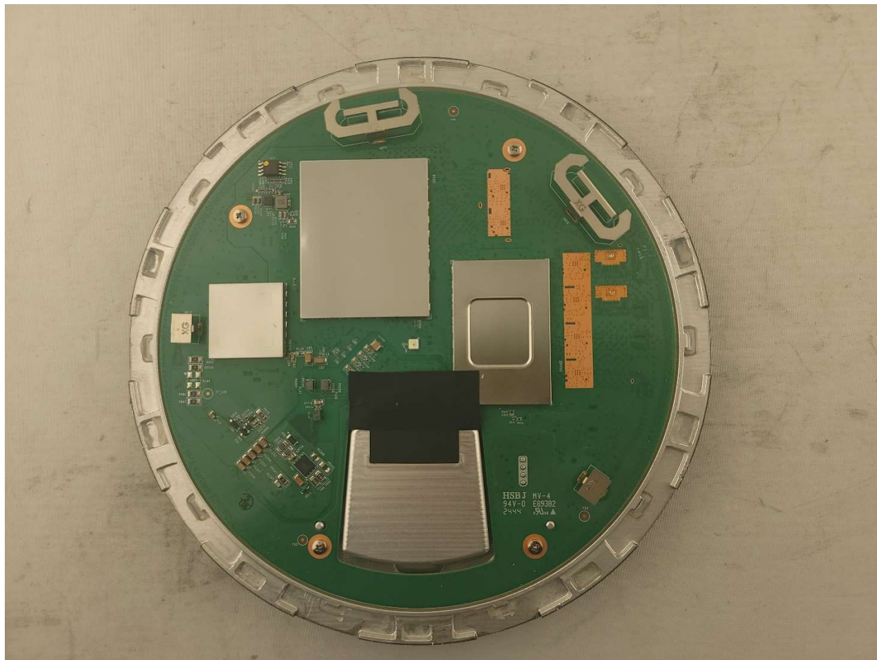
Photograph 2: Internal View of DUT PCB in Back Enclosure
