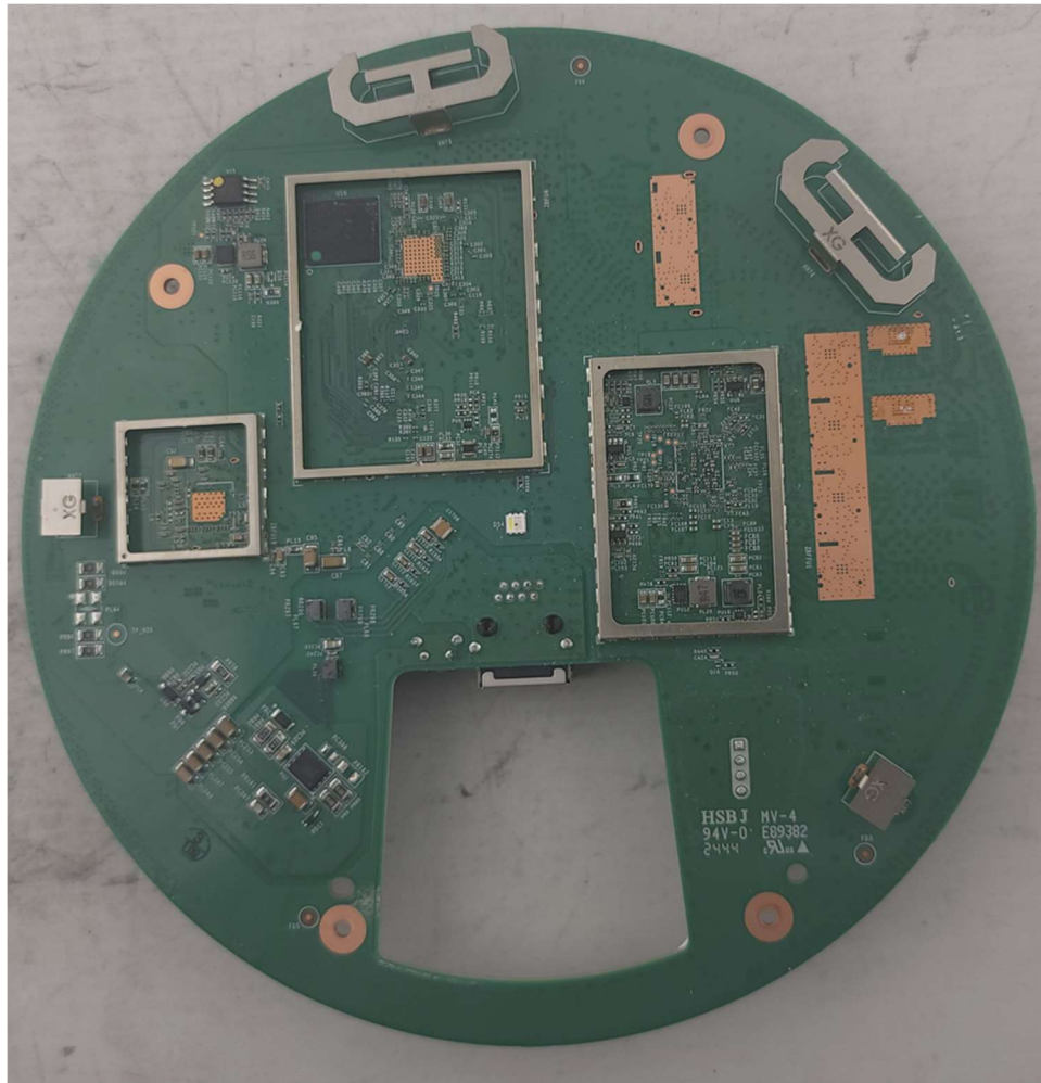
Photograph 1: Front Side of PCB with Cans Off
