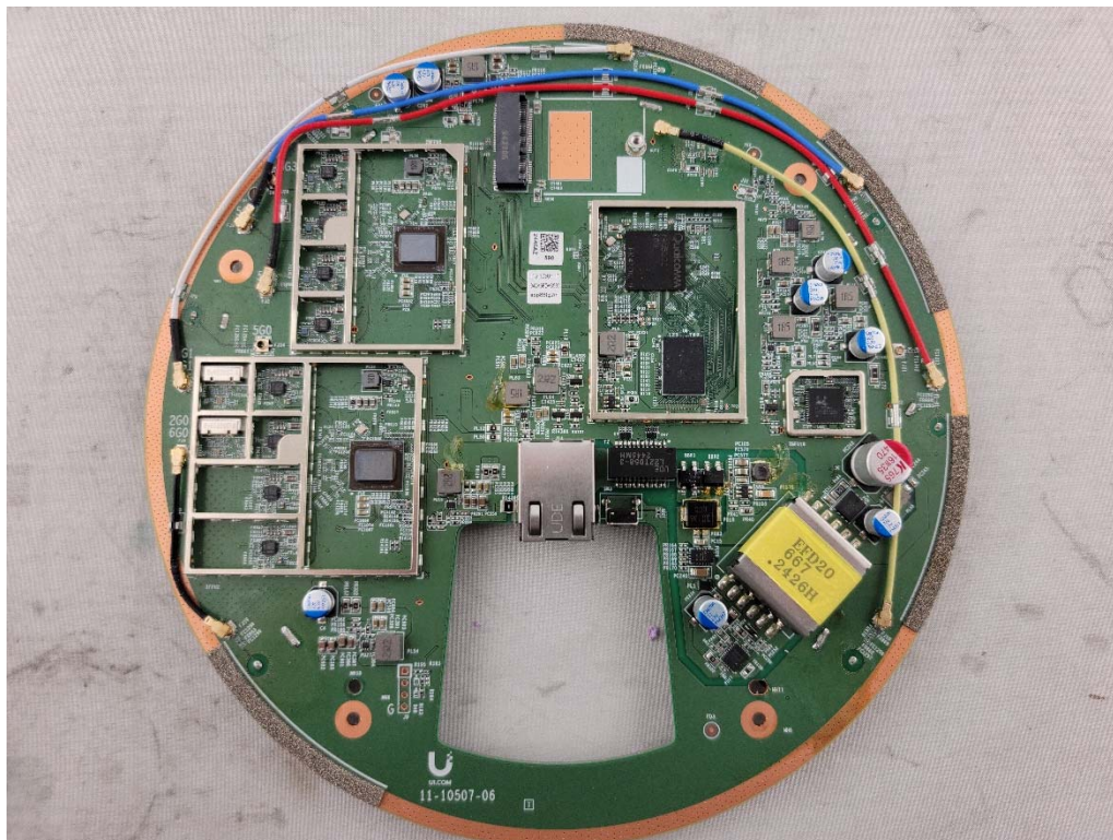
Photograph 6: Bottom of PCB w/Cans off
