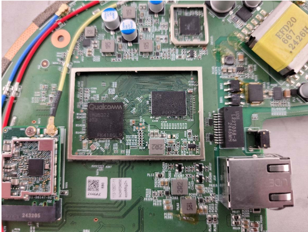
Photograph 10: Bottom of PCB Close Up
