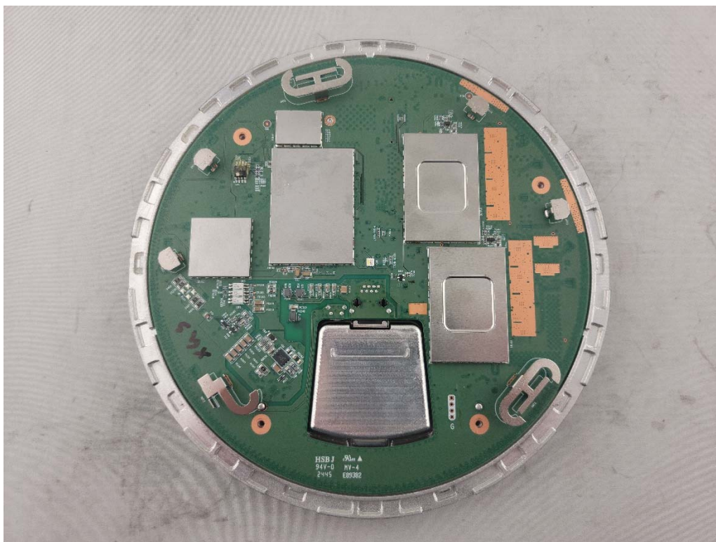
Photograph 1: Front Cover off Showing Top of PCB w/Cans on
