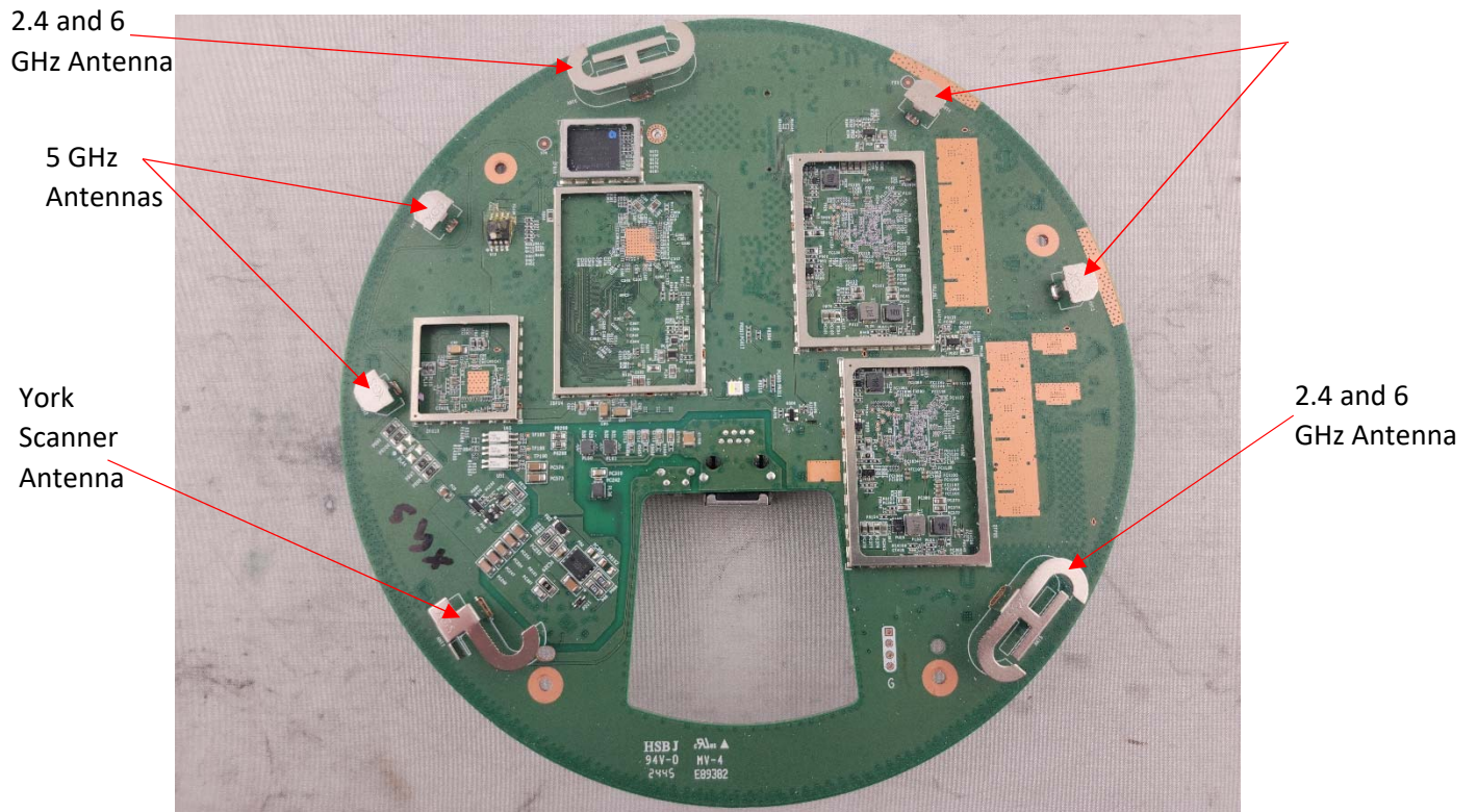
Photograph 2: Top of PCB w/Cans off
