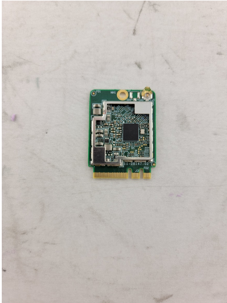
Photograph 1: York PCB
