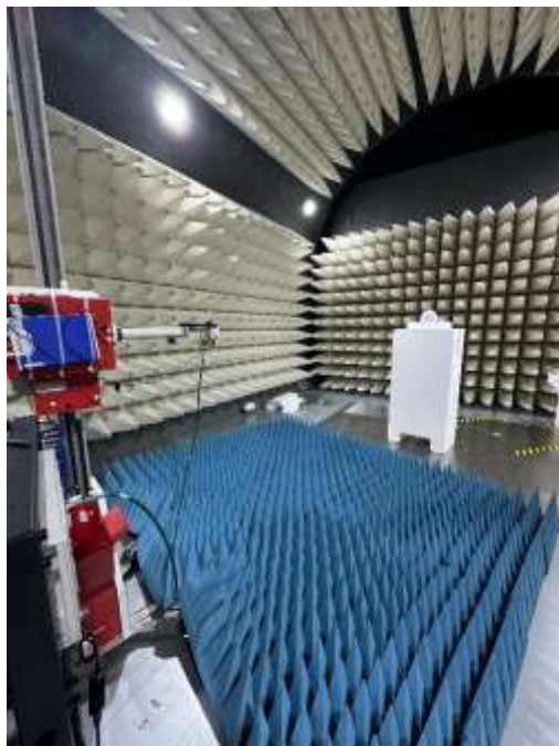
Photograph 3: View Test Set Up Radiated Emissions 17 – 40 GHz
