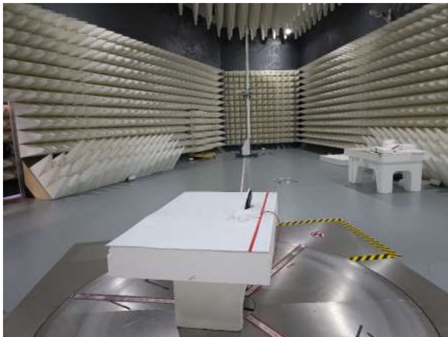
Photograph 1: View Test Set Up Radiated Emissions 30 – 1000 MHz
