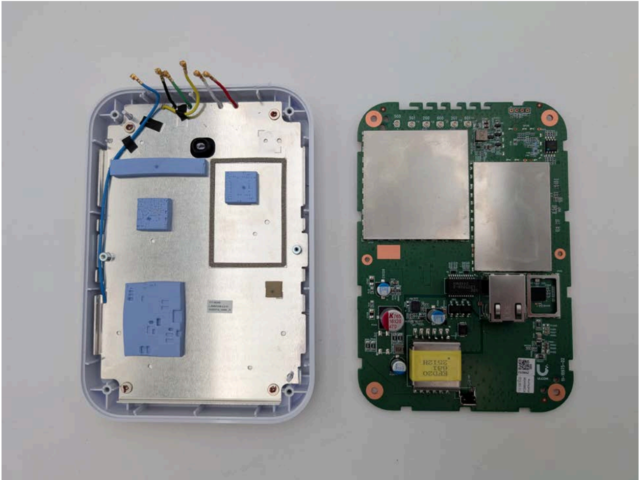
Photograph 2: Internal View PCB Outside of Front Cover
