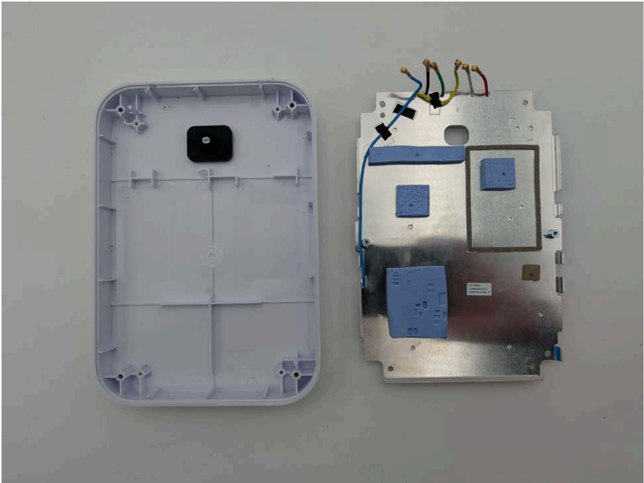
Photograph 1: Internal View Antenna Board Outside Front Cover
