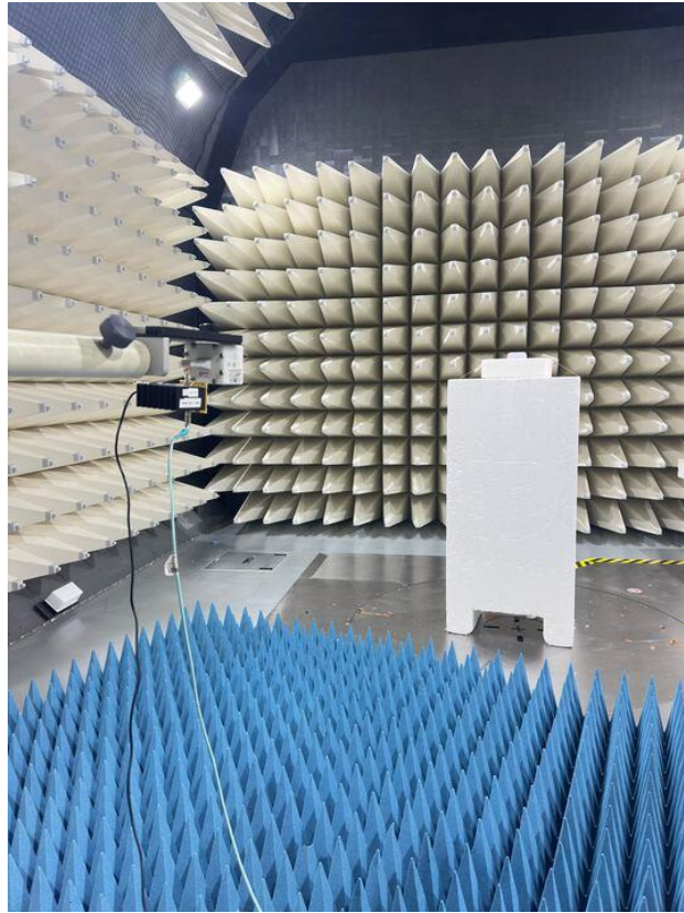
Photograph 3: View Test Set Up Radiated Emissions 17 – 40 GHz
