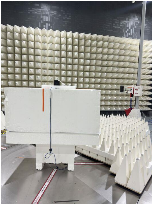
Photograph 1: View Test Set Up Radiated Emissions 30 – 1000 MHz
