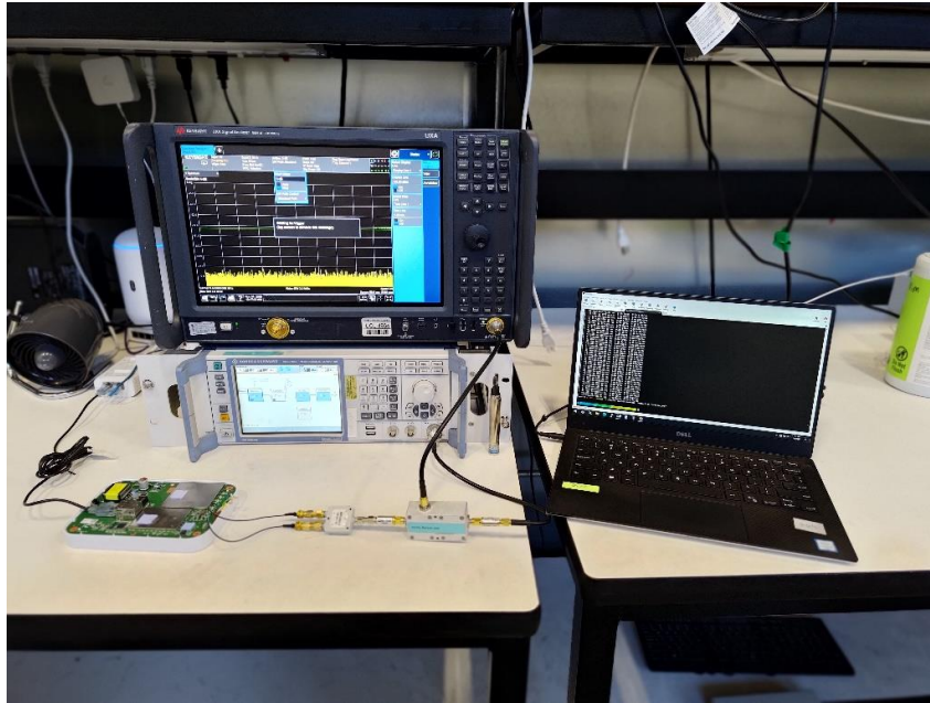
Photograph 5: View Test Set Up DFS
