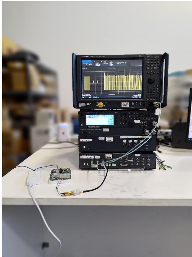
Photograph 6: View Test Set Up CBP
