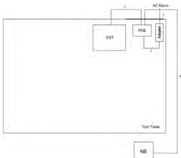
Test Setup Diagram – AC Line Conducted Emission Test - Non-Beamforming
