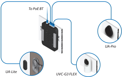
Sample UniFi Access Diagram
