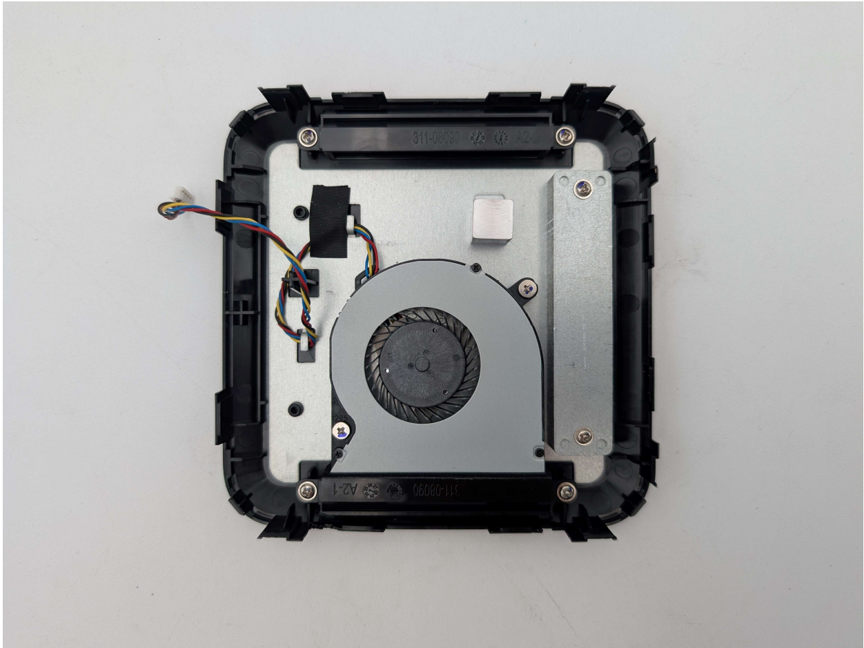
Photograph 6: Bottom Fan Housing
