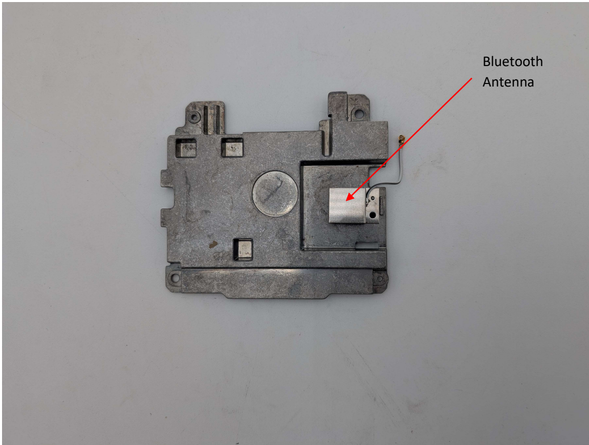
Photograph 5: Top Metal Housing Showing Top Side of Metal Piece
