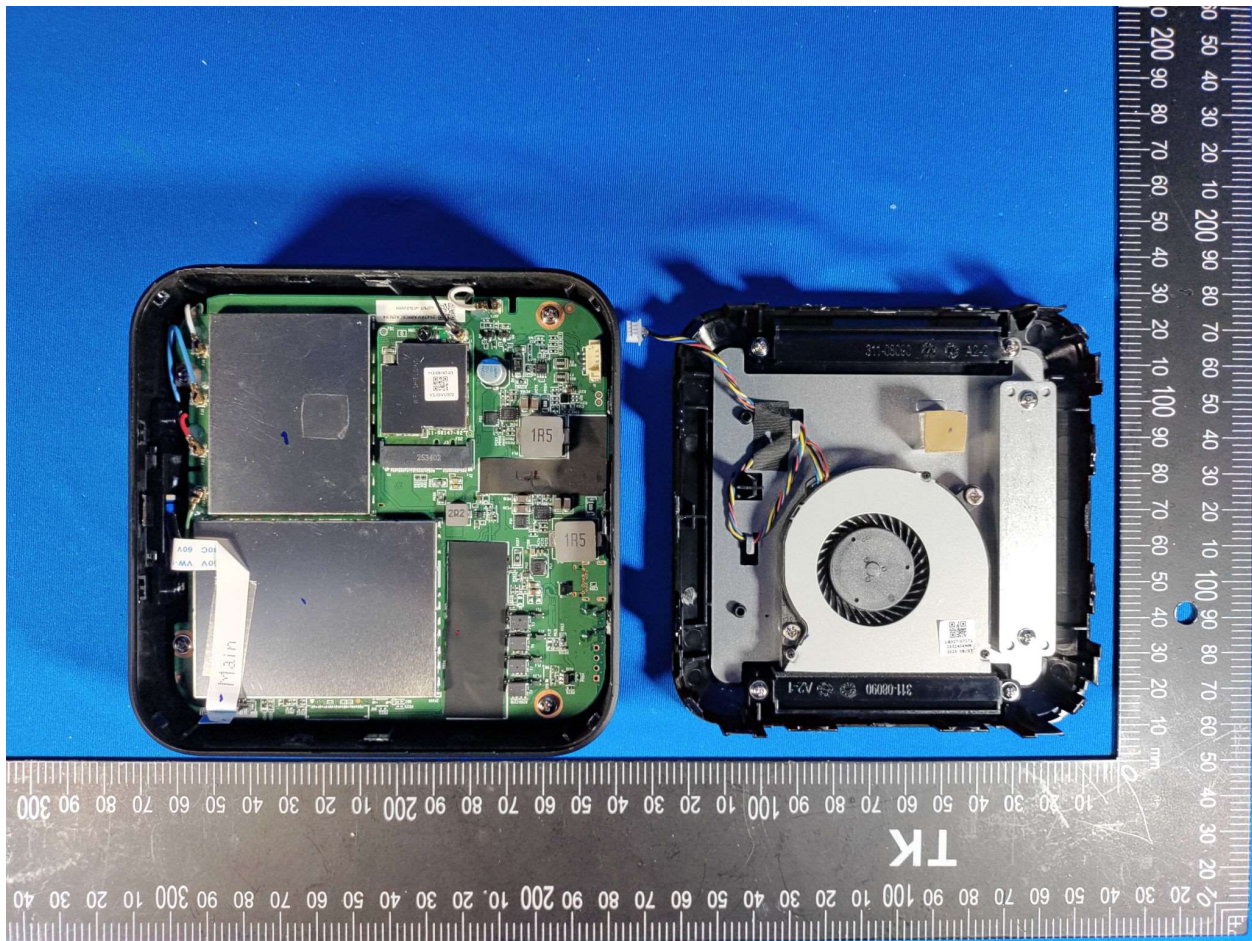
Photograph 1: Internal View of DUT Bottom Removed
