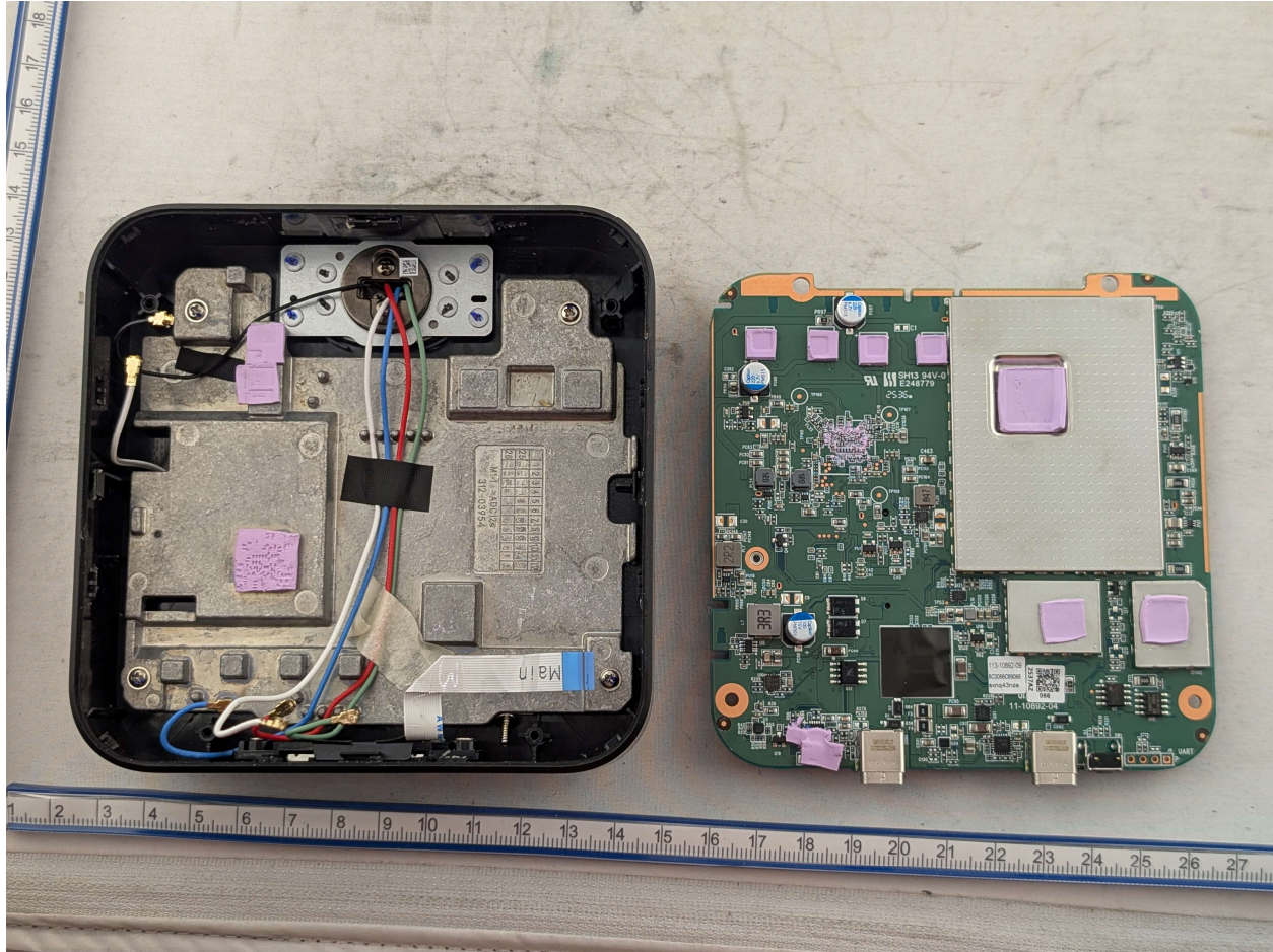
Photograph 2: Internal View of DUT PCB Removed
