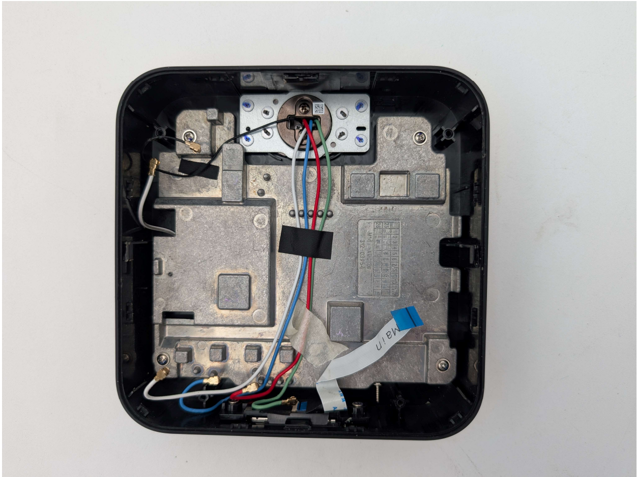
Photograph 3: Top Metal Housing Showing Back of Metal Piece
