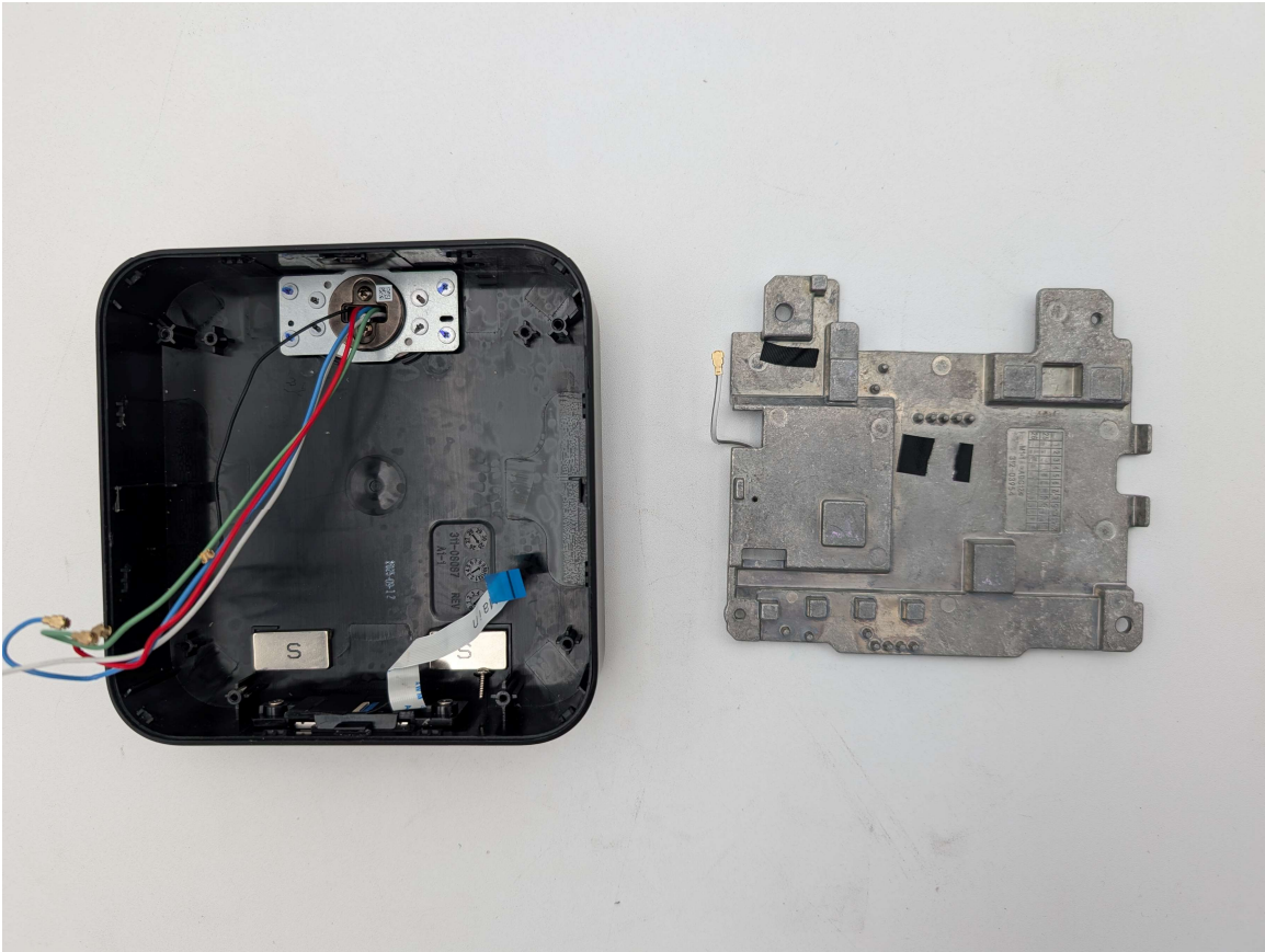
Photograph 4: Top Metal Removed From Top Housing
