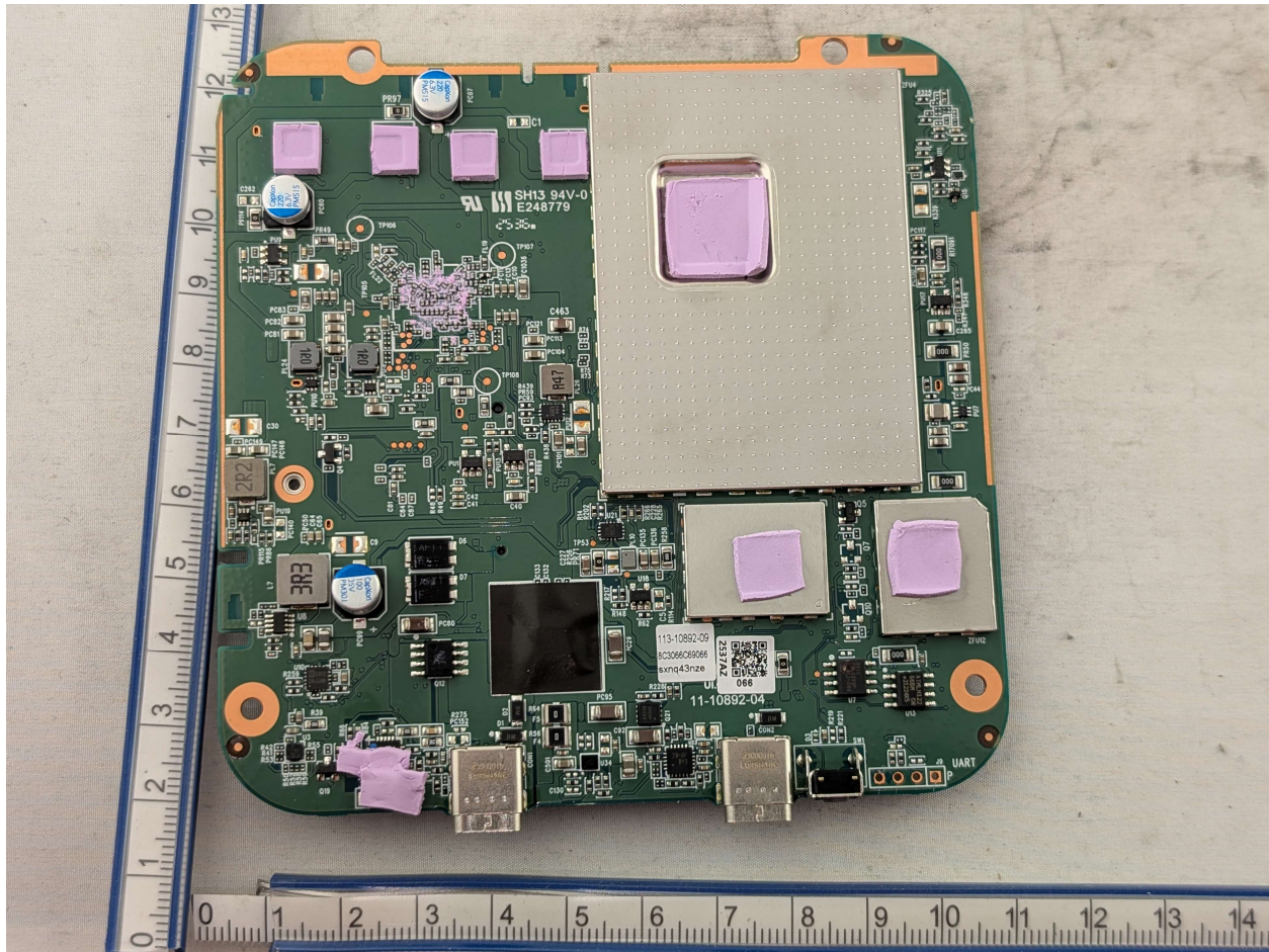
Photograph 2: Internal View of DUT Main PCB Top w/Cans
