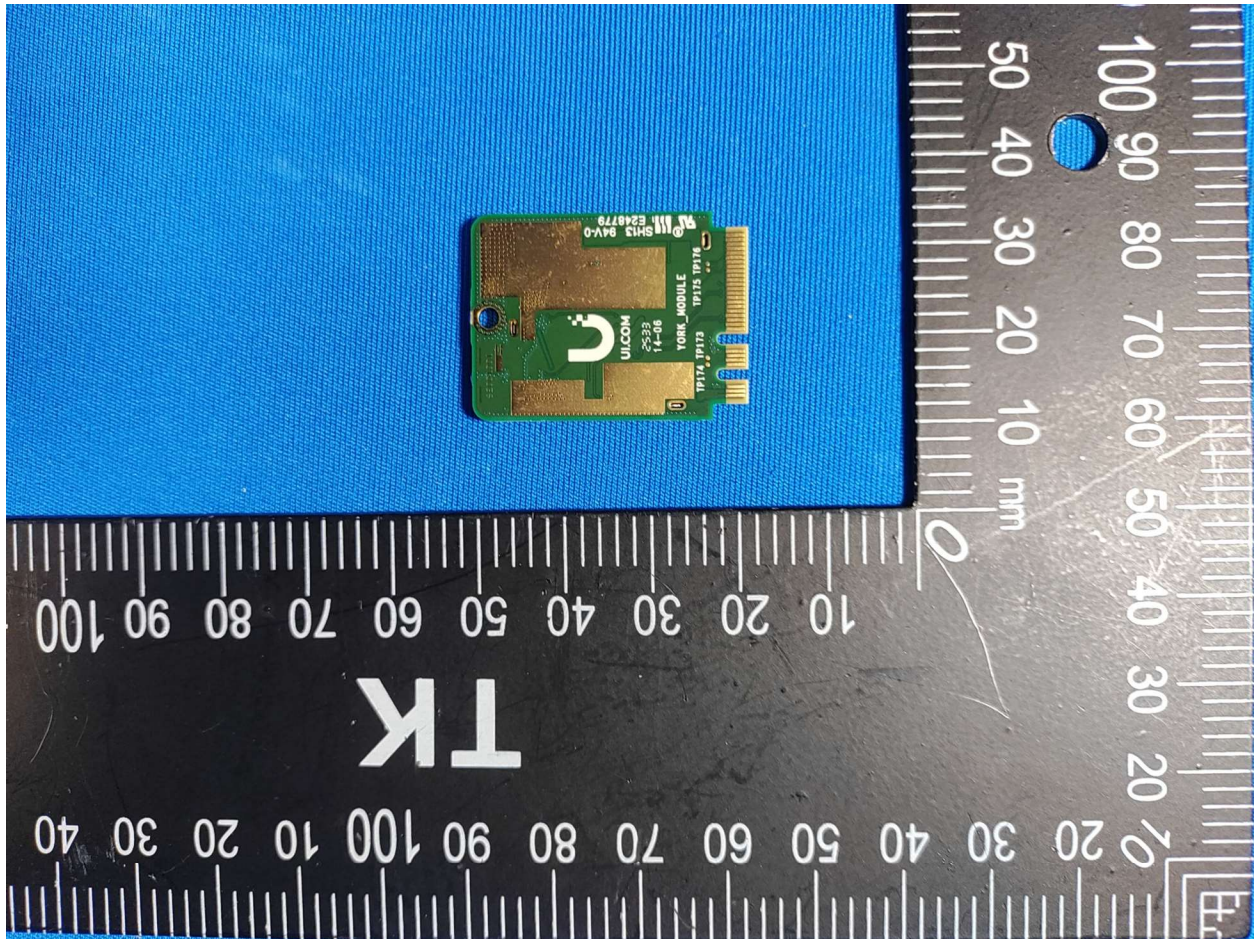
Photograph 7: Top Side Of PCB York Scanning PCB
