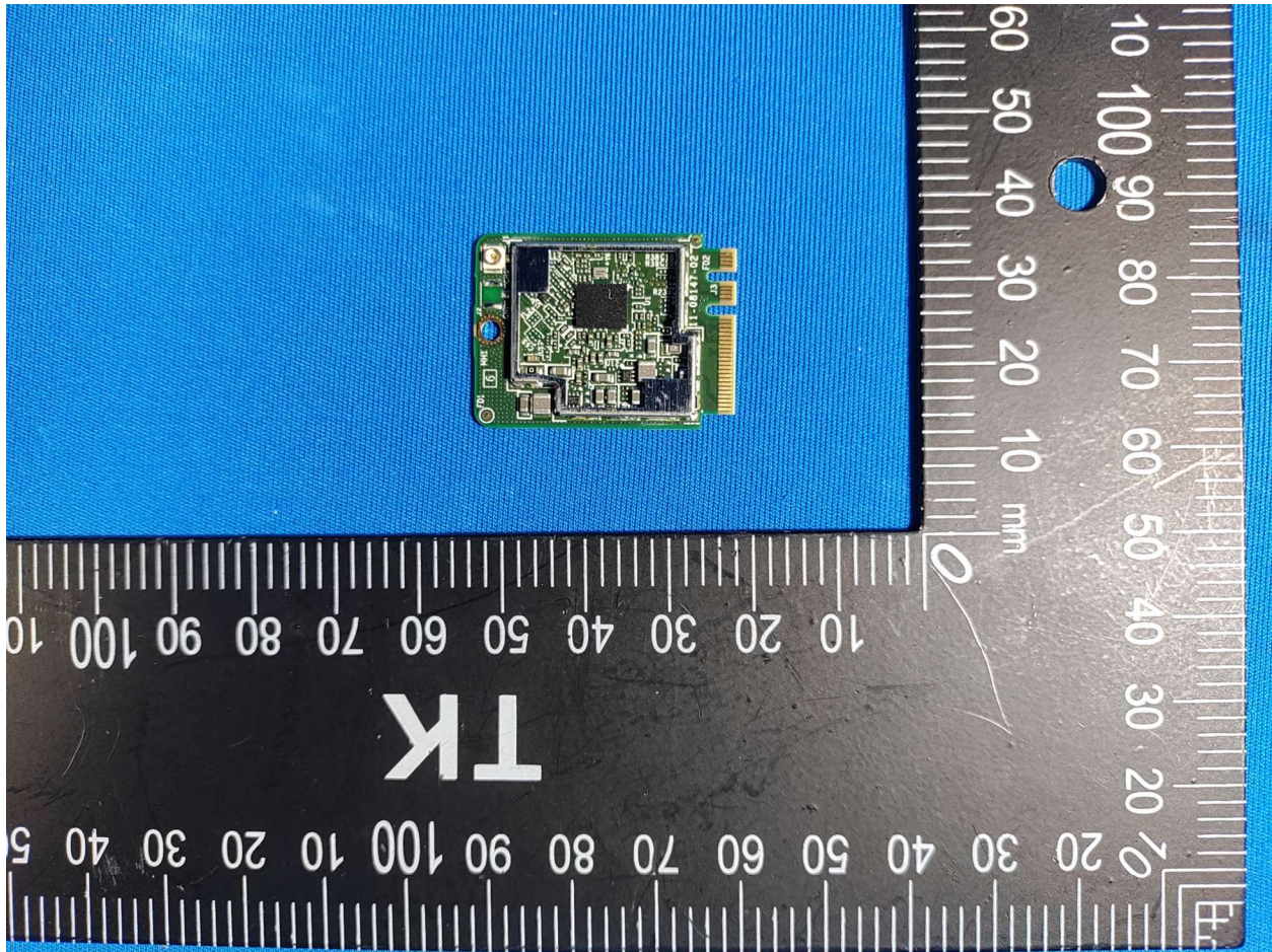
Photograph 6: Internal View of DUT York Scanning PCB
