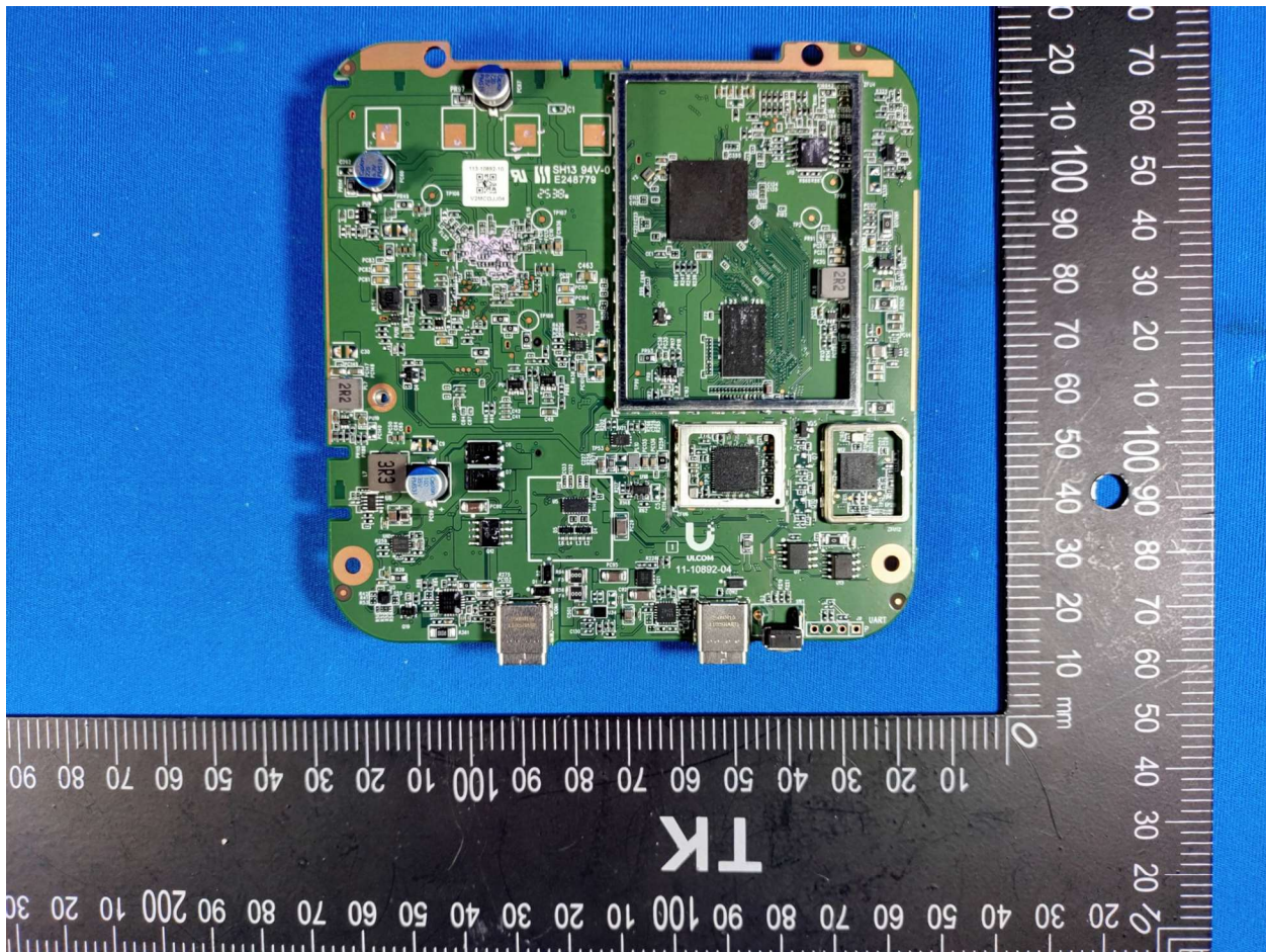
Photograph 4: Internal View of DUT Main PCB Top w/o Cans
