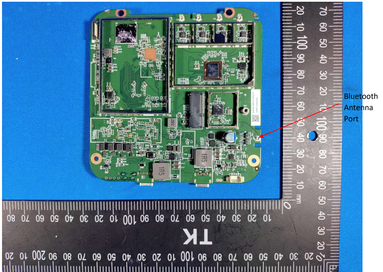
Photograph 5: Internal View of DUT Main PCB Bottom w/o Cans
