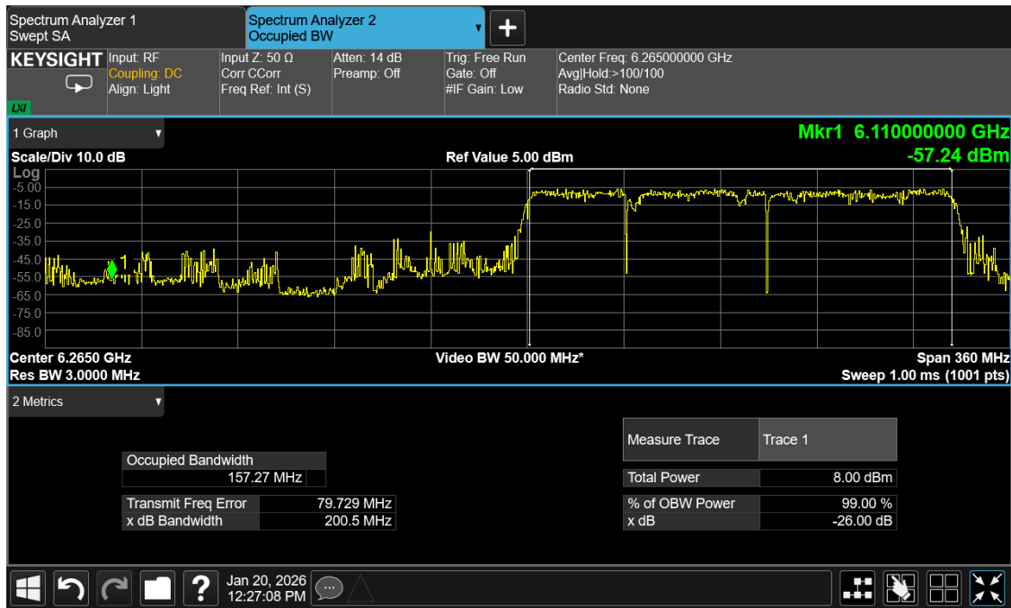
Plot 9: EUT 320MHz Bandwidth Reduction
