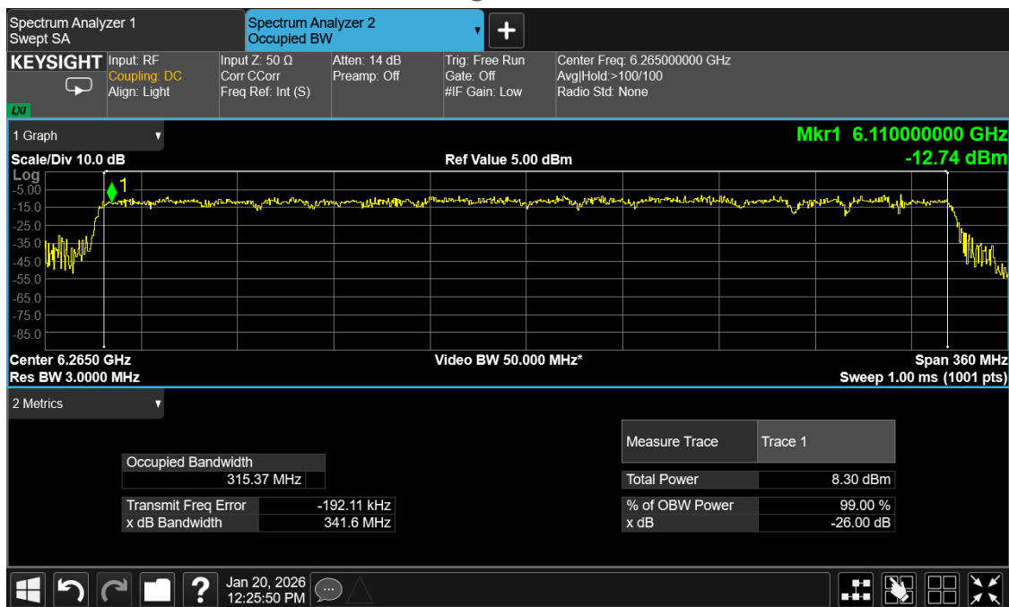
Plot 8: EUT 320MHz Bandwidth
