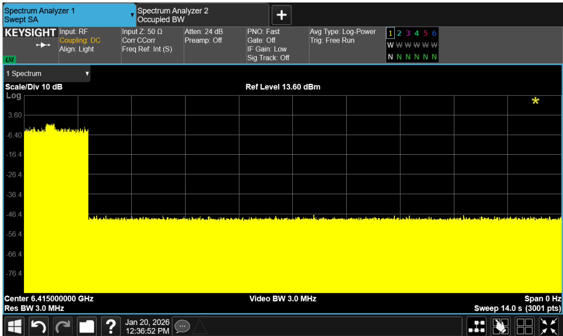
Plot 12: AWGN Signal Detection 320MHz
