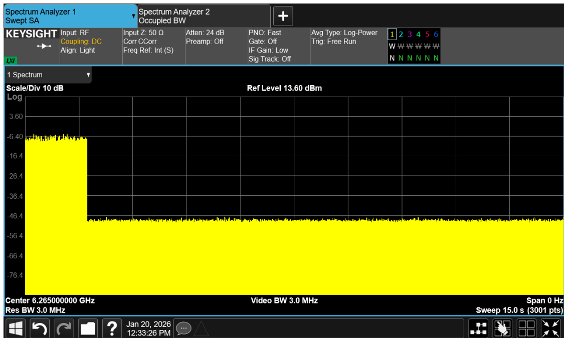
Plot 10: AWGN Signal Detection 320MHz
