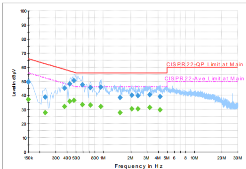
ENV216 Auto Test FCC Power Bar - L
