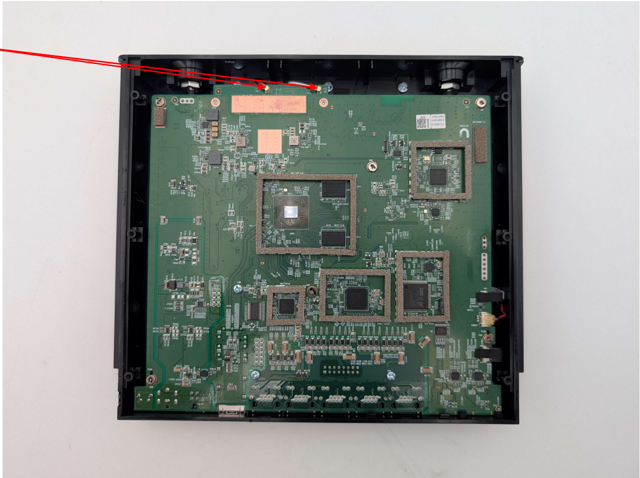
Photograph 2: Main PCB Bottom Inside Top Cover
