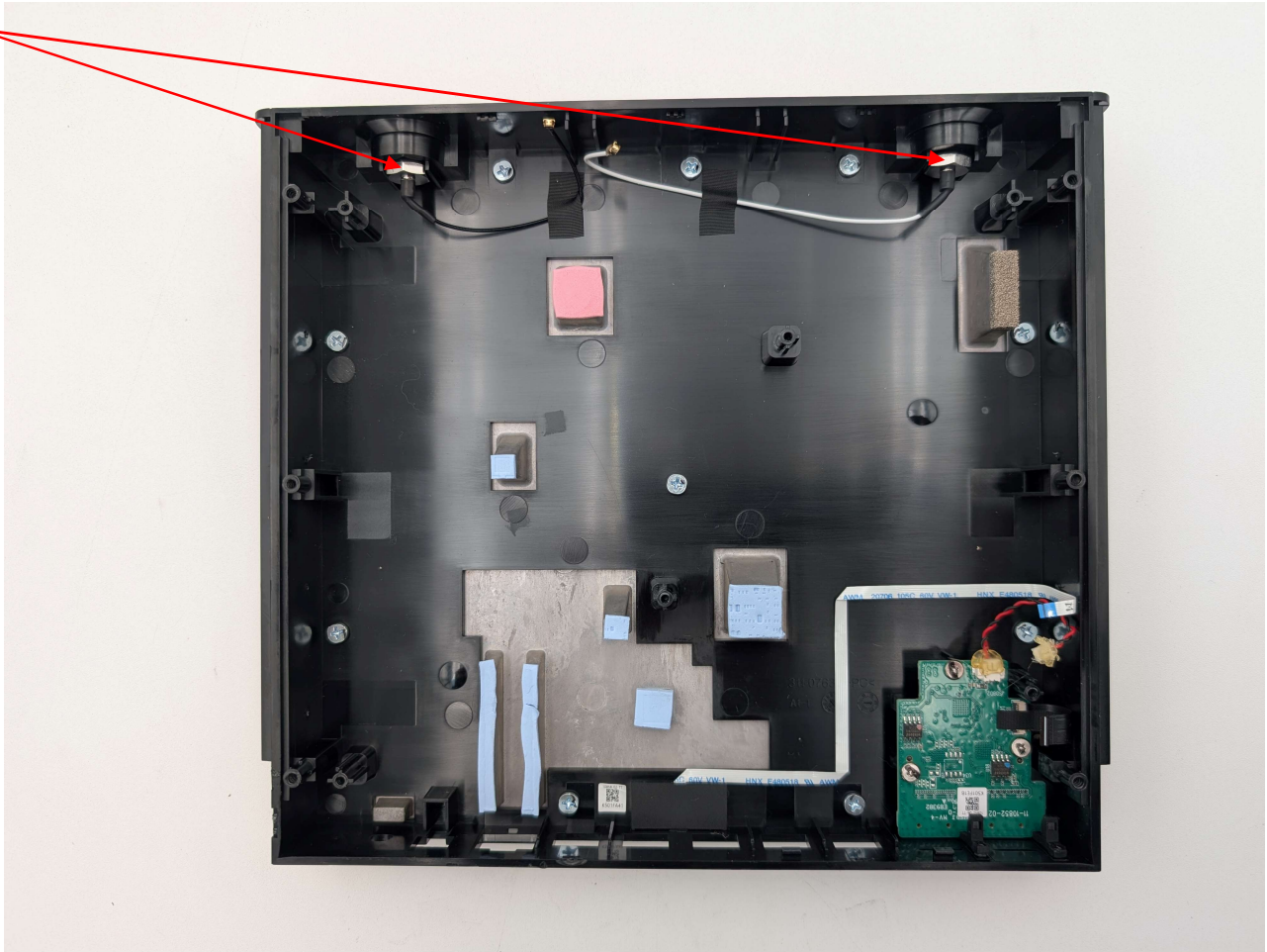
Photograph 6: Top of EUT Main PCB Removed
