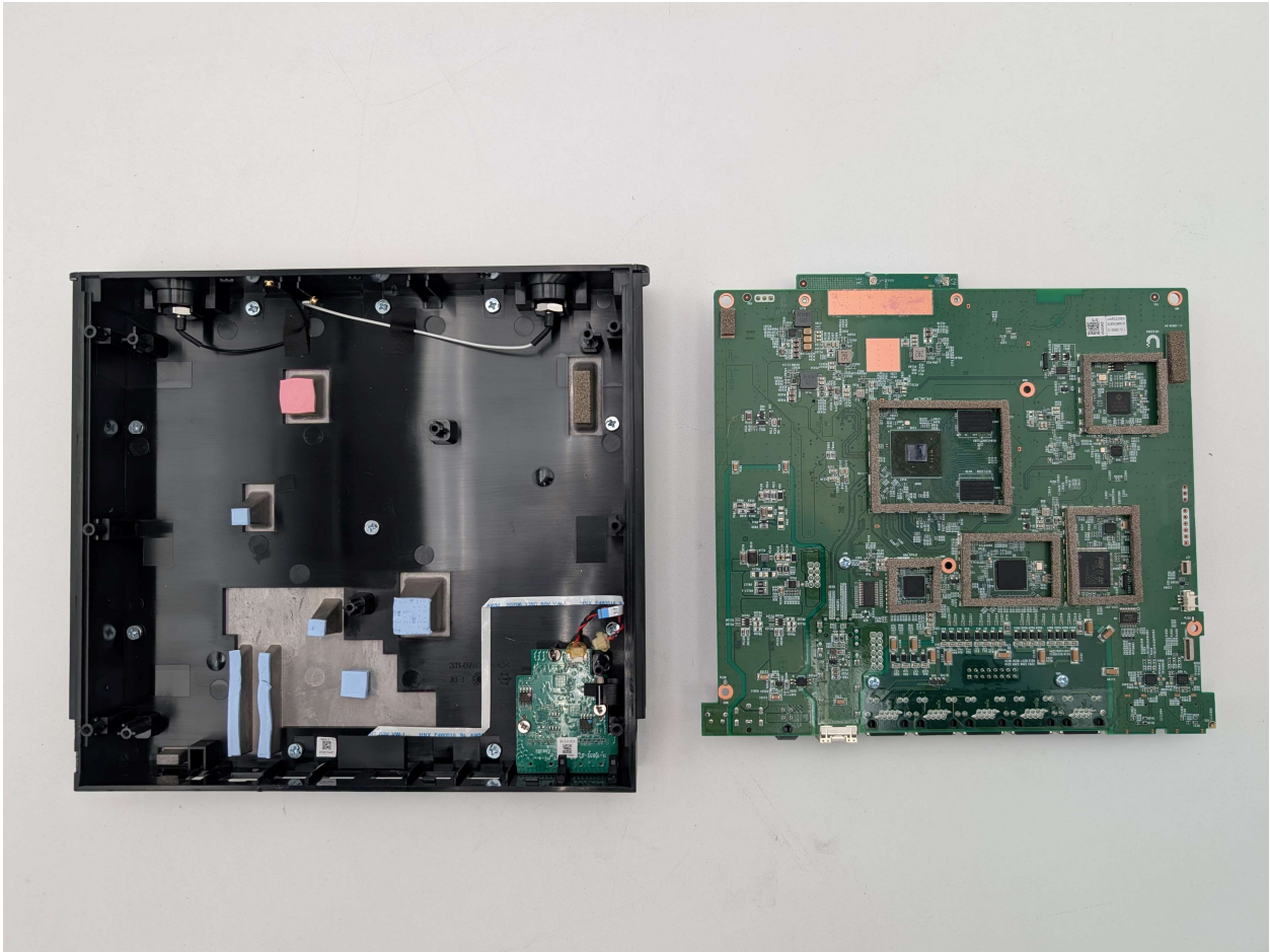
Photograph 3: Main PCB Removed Showing Top Cover
