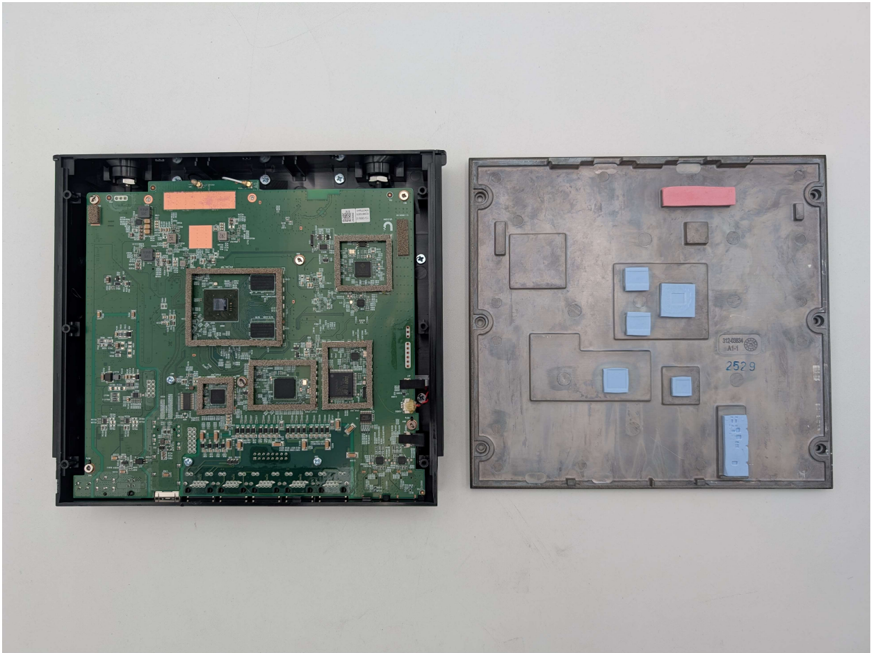
Photograph 1: Back Cover Off Showing Bottom of Main PCB
