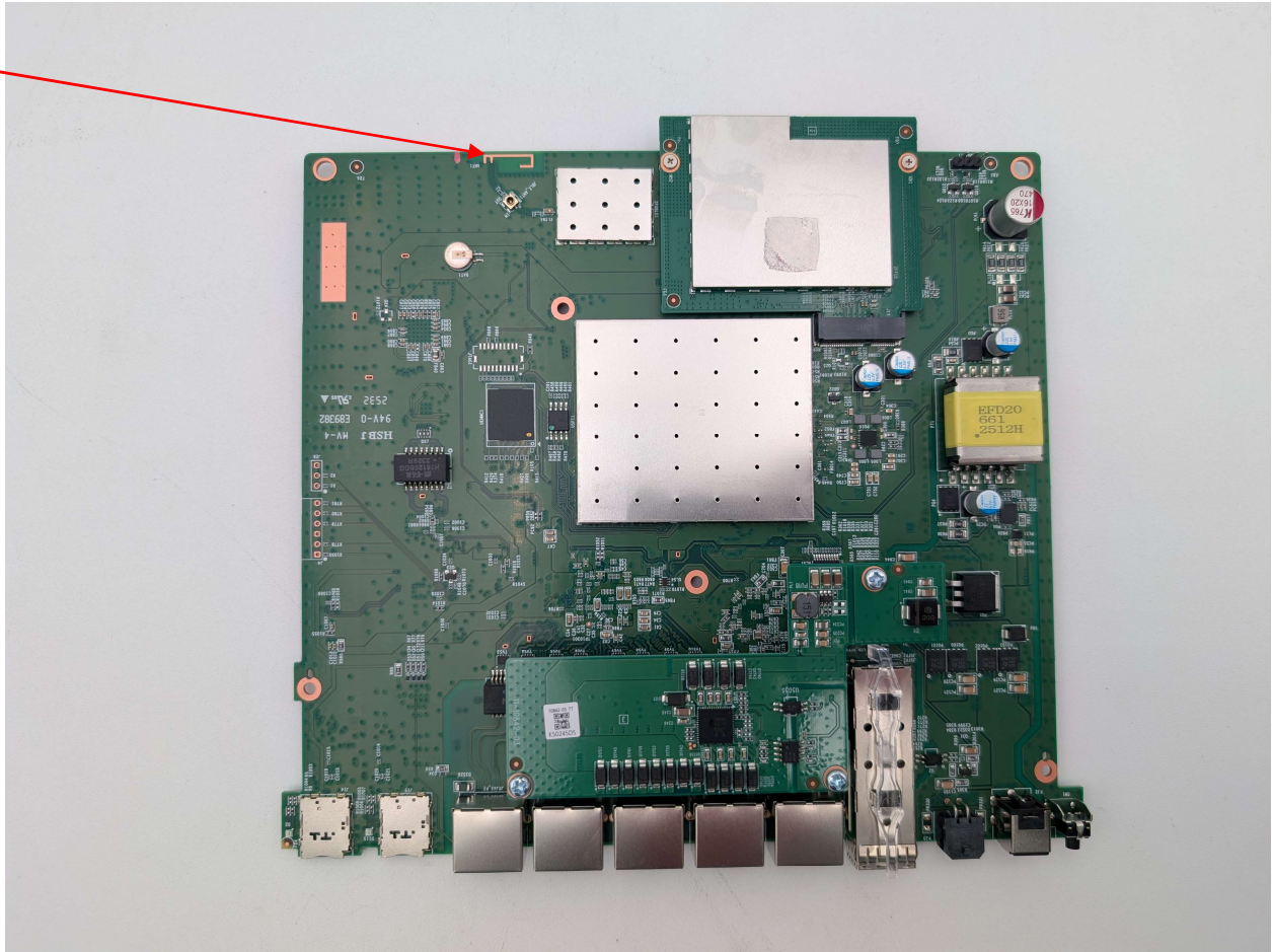
Photograph 5: Main PCB Top w/Cans
