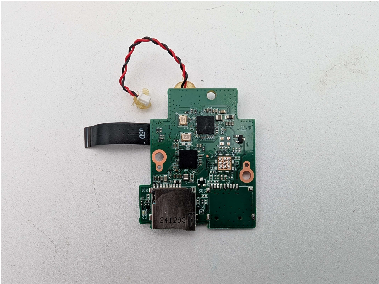
Photograph 1: SD PCB Top
