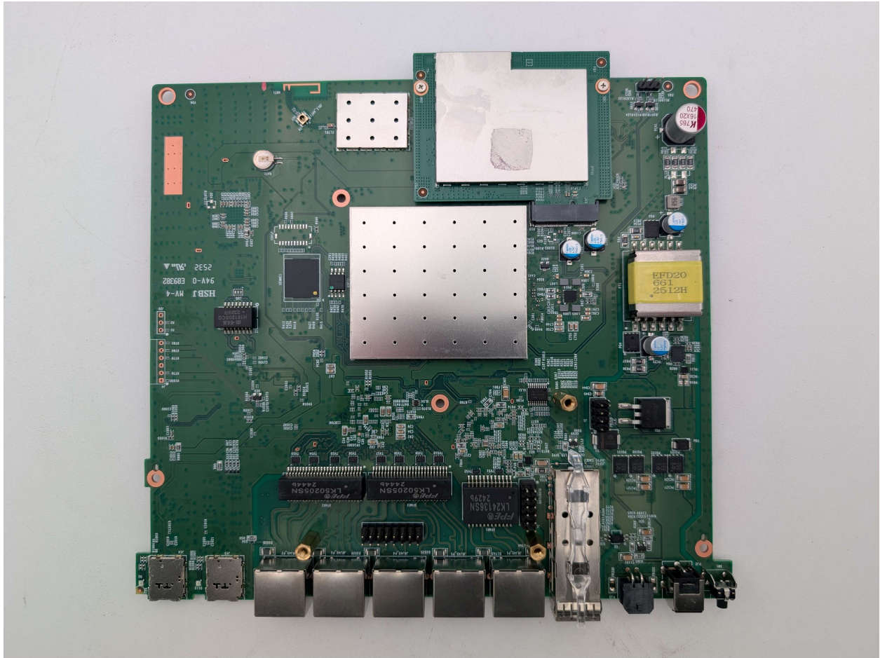
Photograph 4: Main PCB w/POE Power PCB Removed
