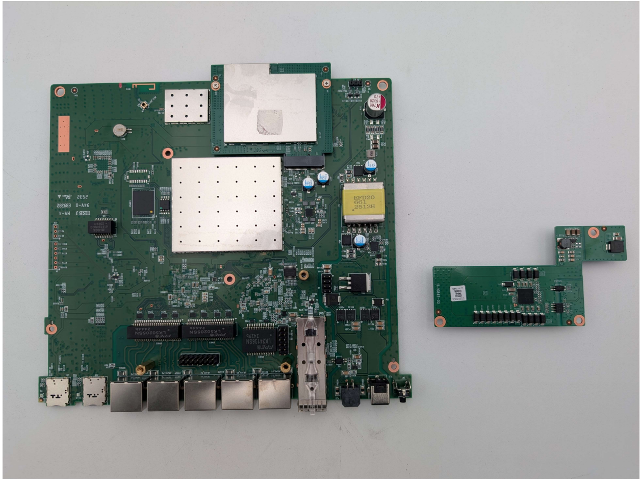
Photograph 3: POE Power PCB Off Main PCB
