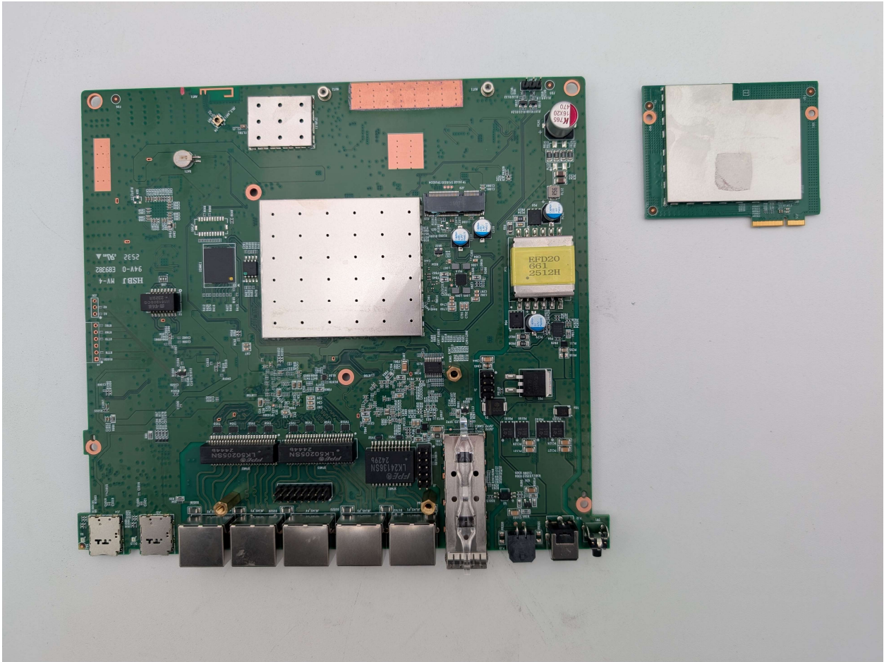
Photograph 1: RF PCB Off Main PCB
