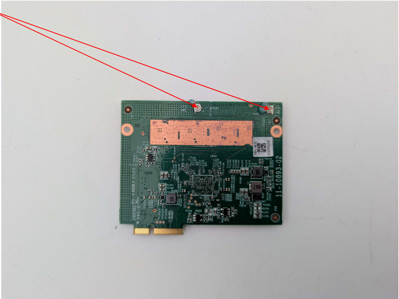
Photograph 6: RF PCB Bottom
