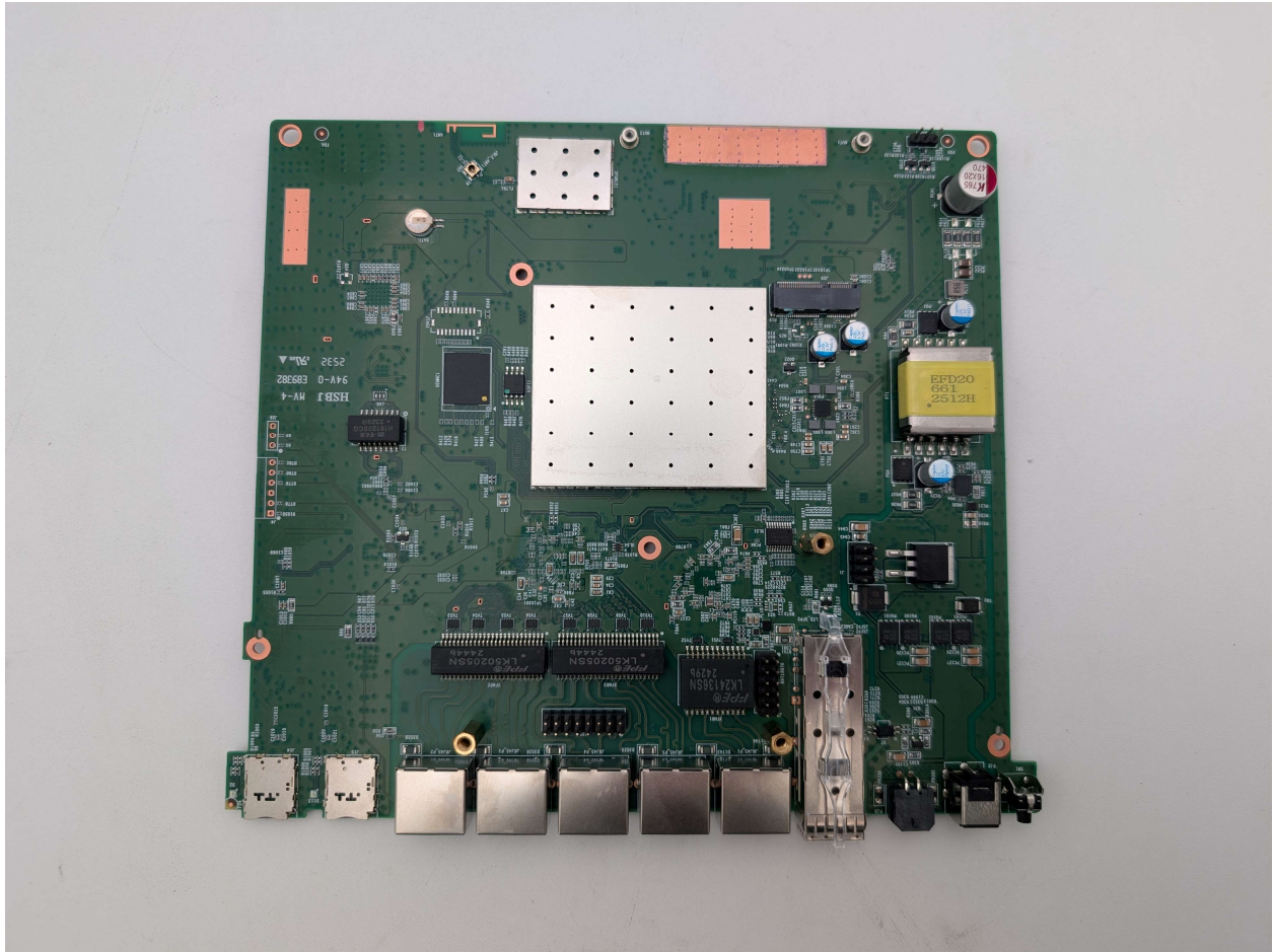
Photograph 2: Main PCB w/RF PCB Removed
