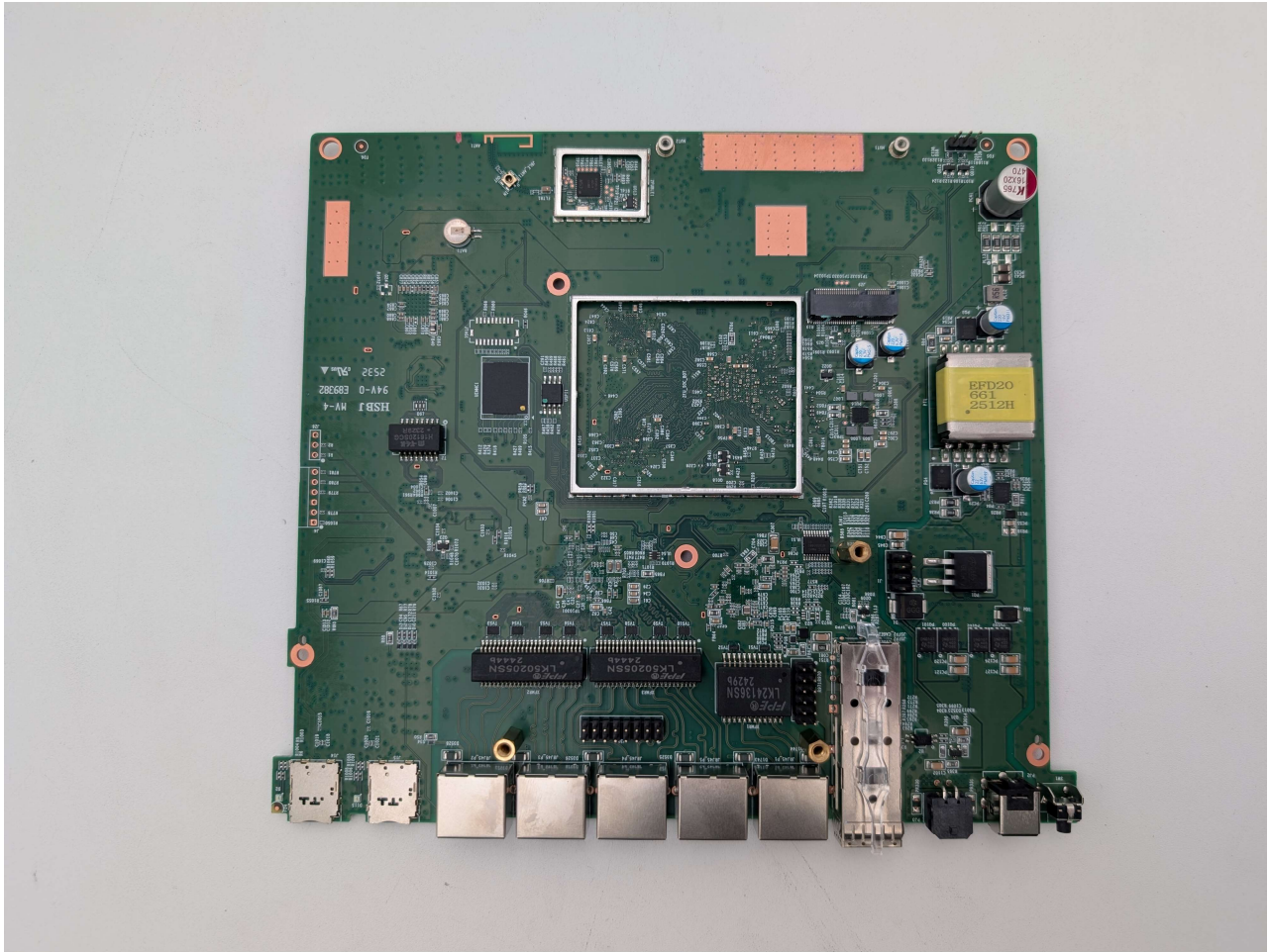
Photograph 3: Main PCB w/o Cans
