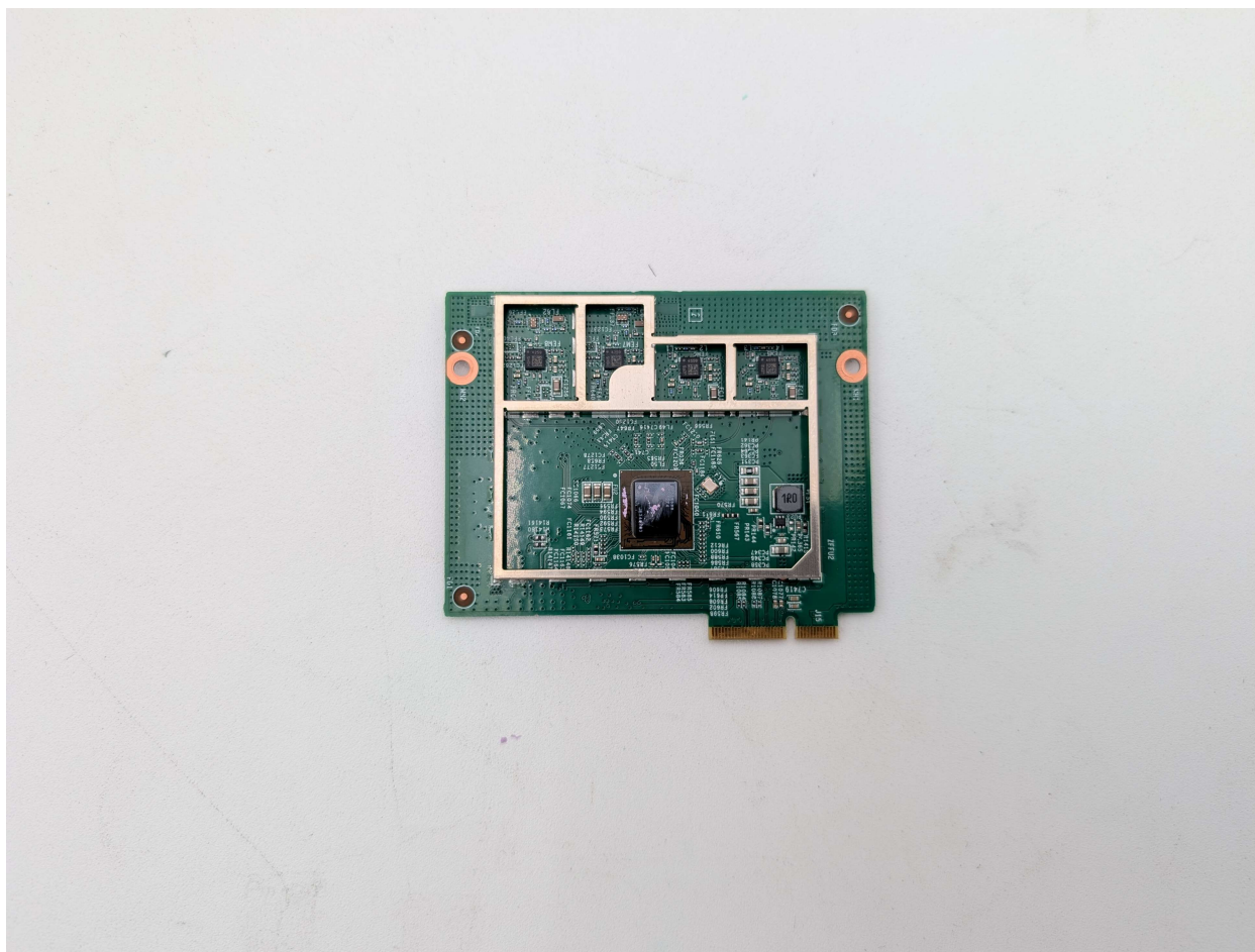
Photograph 5: RF PCB Top w/o Can
