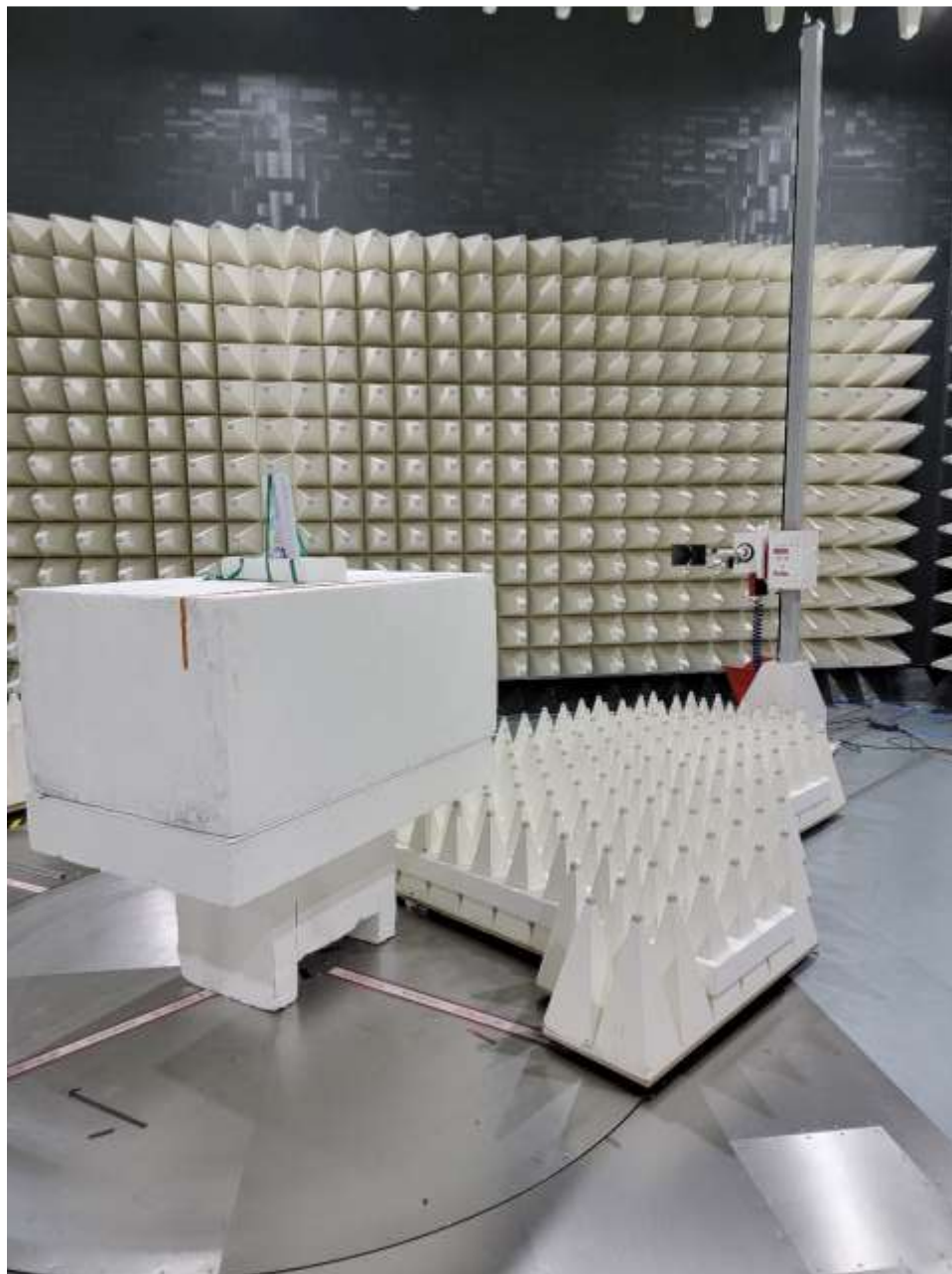
Photograph 2: View Test Set Up Radiated Emissions 1 – 17 GHz
