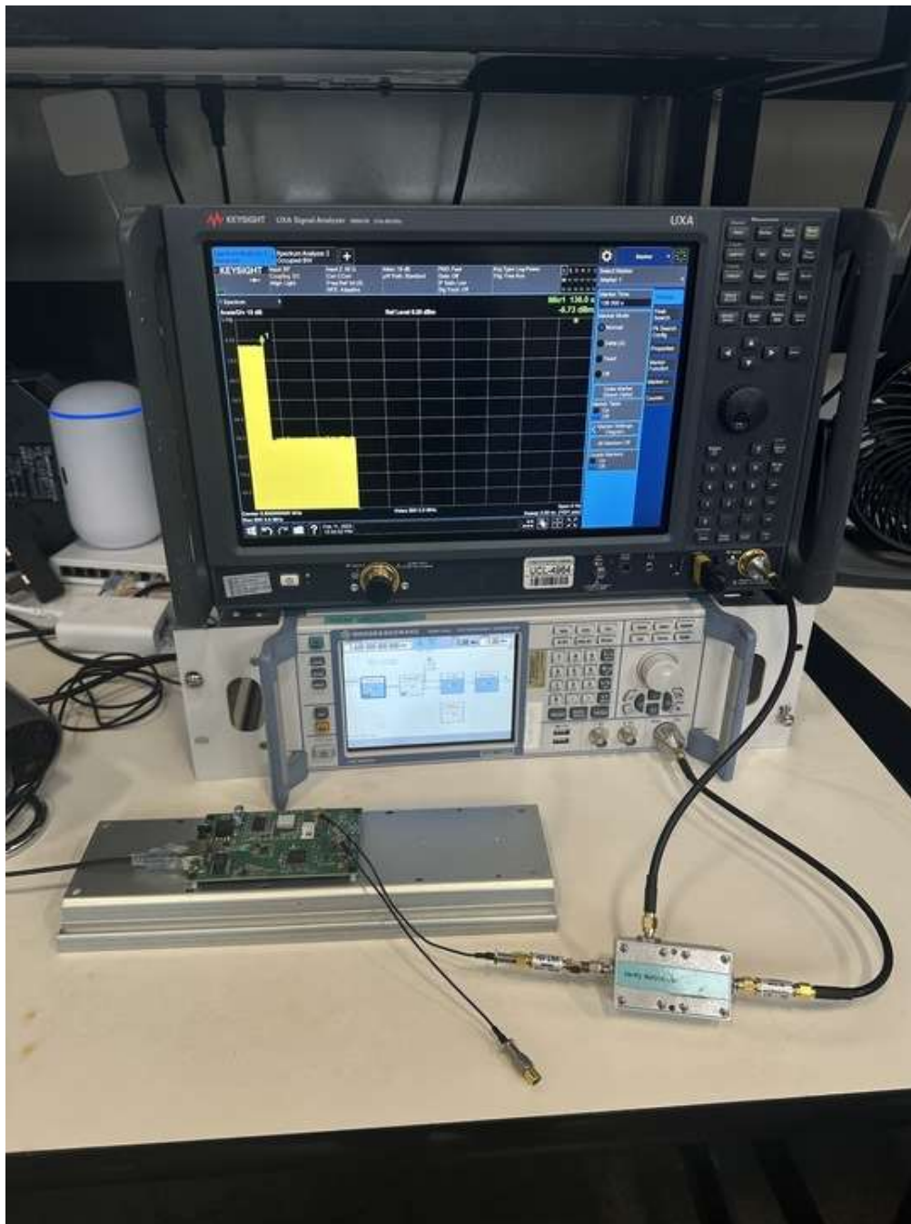
Photograph 5: View Test Set Up DFS
