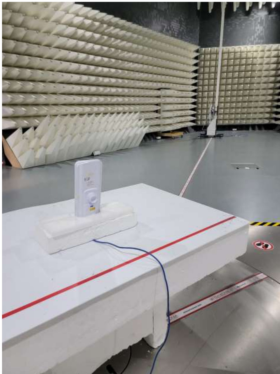
Photograph 1: View Test Set Up Radiated Emissions 30 – 1000 MHz
