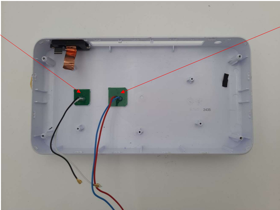
Photograph 9: Top Cover
