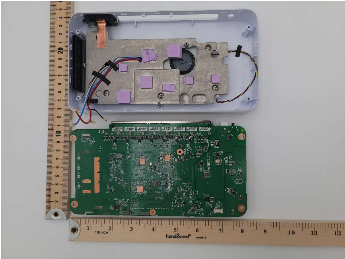
Photograph 3: PCB Bottom Outside of Top Cover
