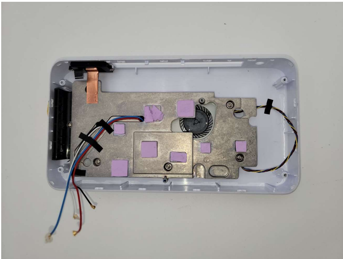
Photograph 5: Top Cover w/Fan
