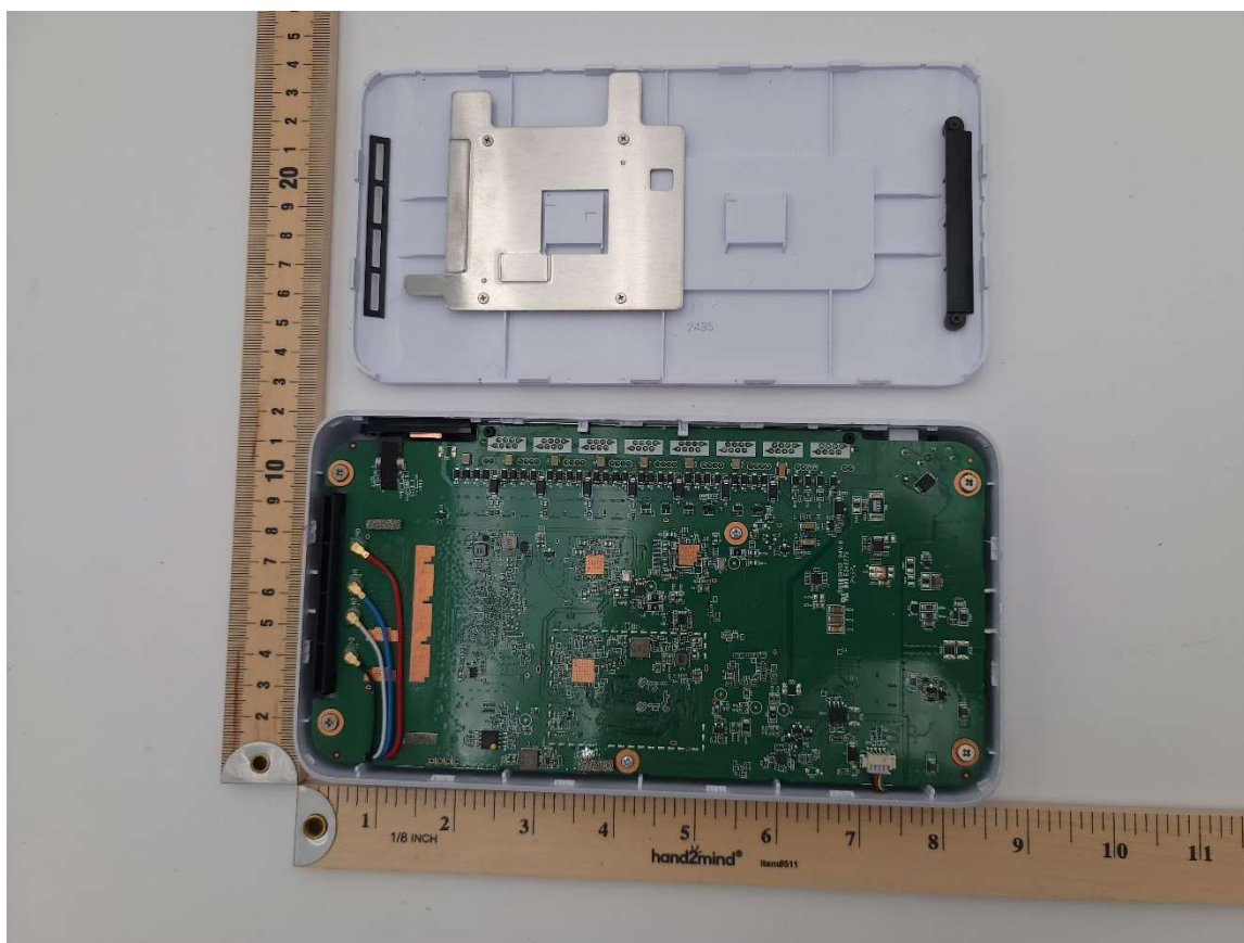
Photograph 1: Bottom Cover Removed Showing PCB Board
