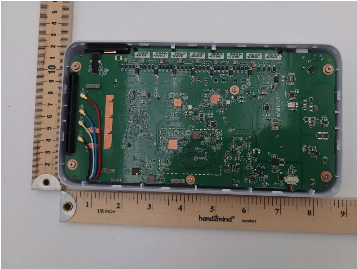
Photograph 2: PCB Bottom In Top Cover
