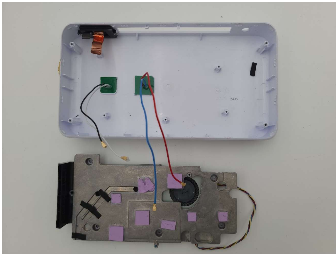
Photograph 6: Top Cover w/Fan Removed
