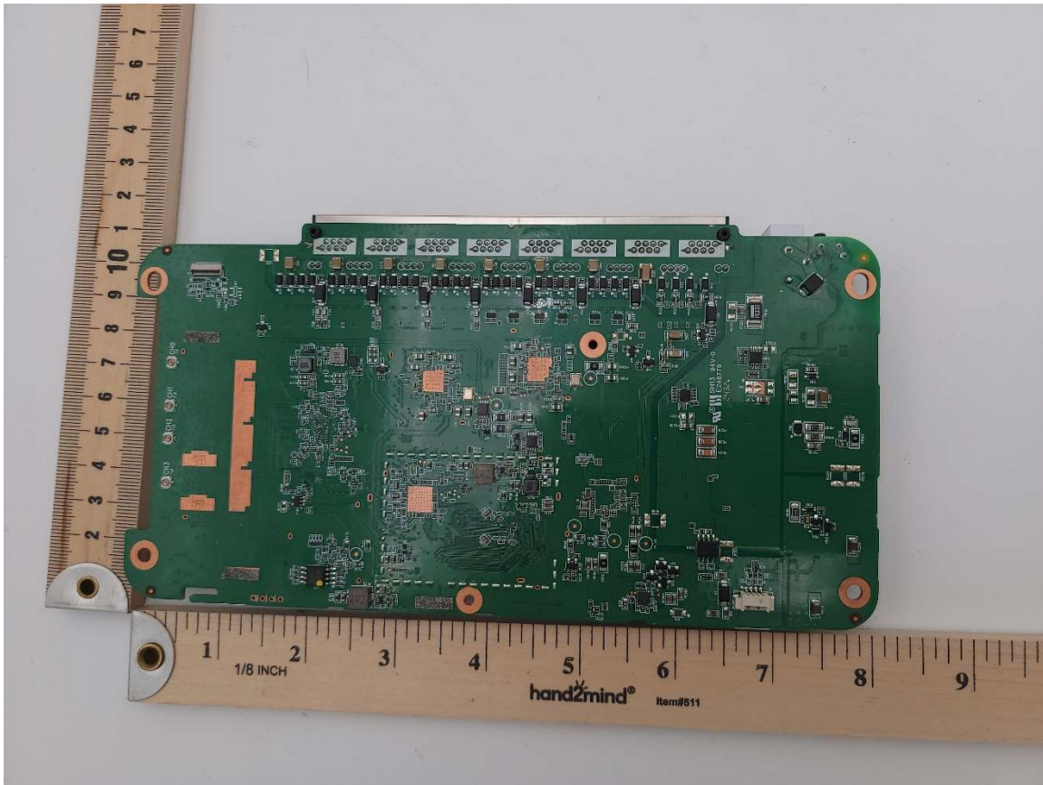
Photograph 4: Bottom Side of PCB
