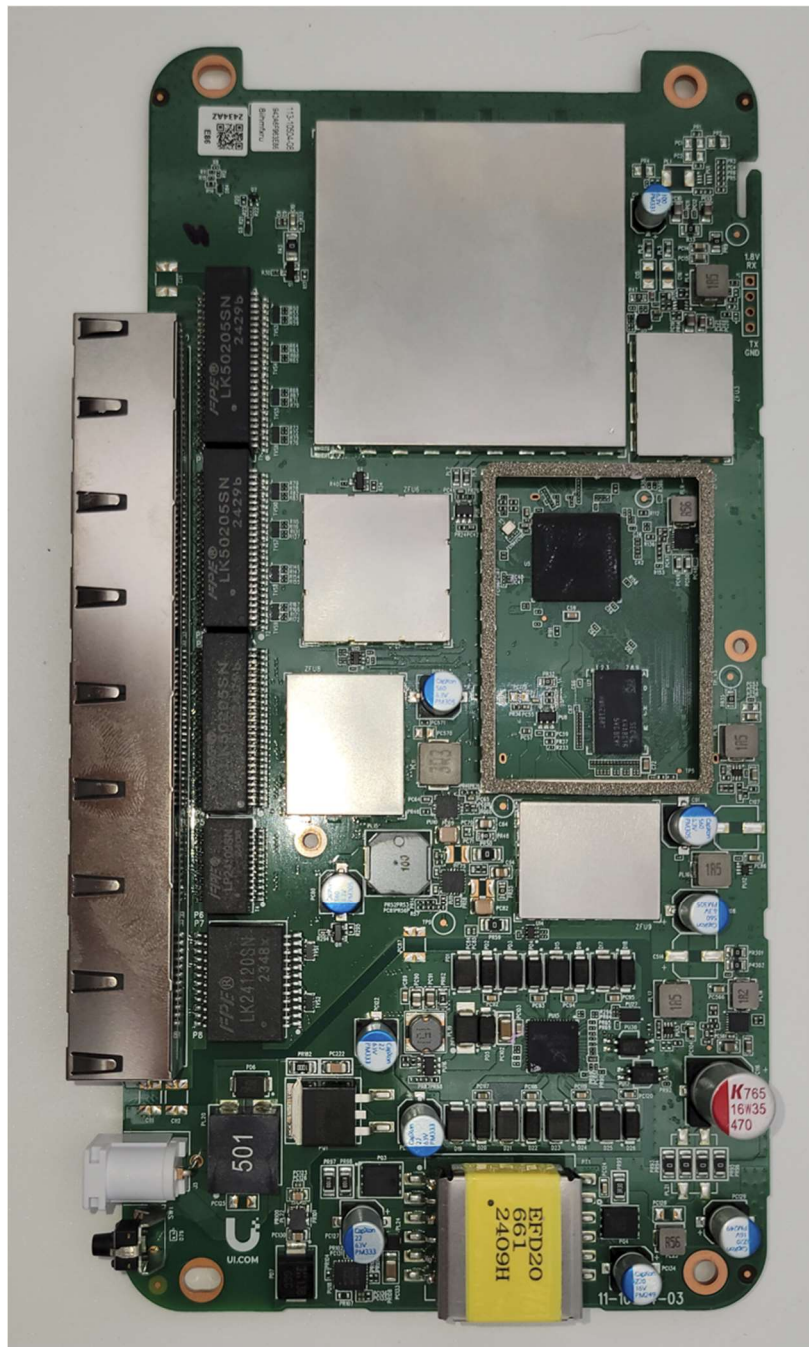
Photograph 1: Top Side Of PCB w/Cans
