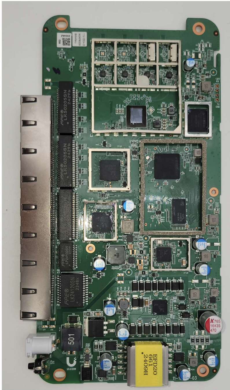
Photograph 2: Top Side PCB w/o Cans
