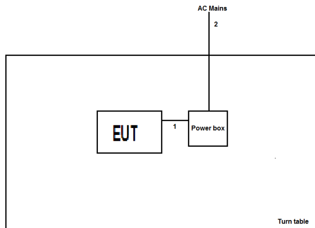
Test Setup Diagram - Radiated Test
