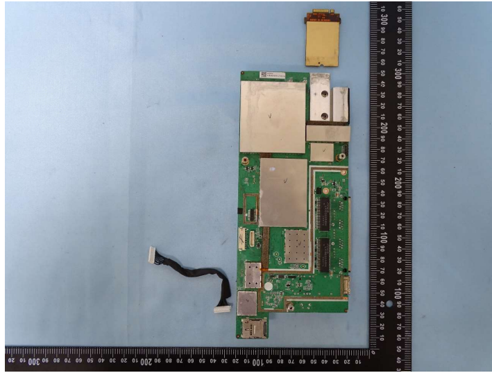
Photograph 29: Front of Main PCB
