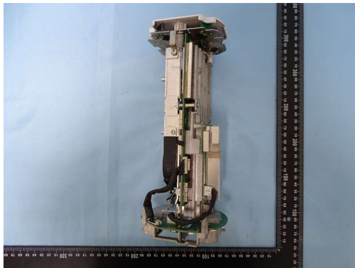
Photograph 5: Disassembled DUT
