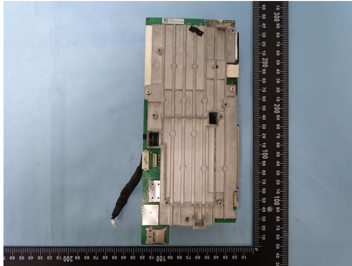
Photograph 27: Front of Main PCB w/Heat Sink
