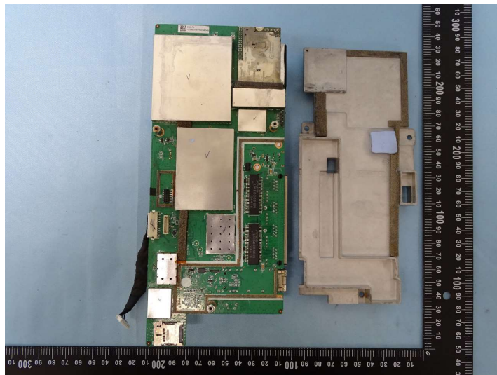
Photograph 28: Front of Main PCB Heat Sink Removed
