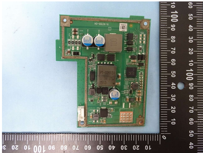
Photograph 8: Power Board PCB
