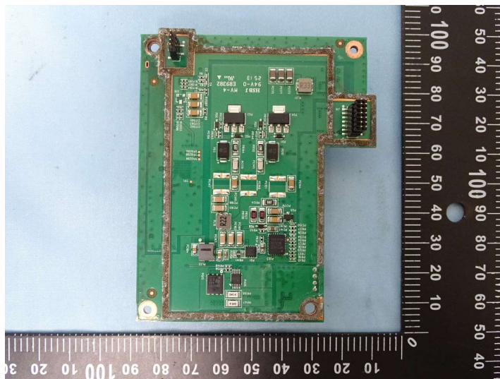
Photograph 12: Power Board PCB
