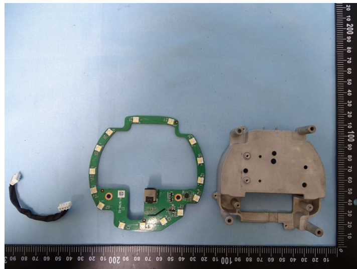
Photograph 18: LED PCB Disassembled
