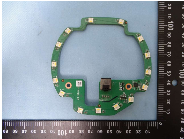
Photograph 19: LED PCB
