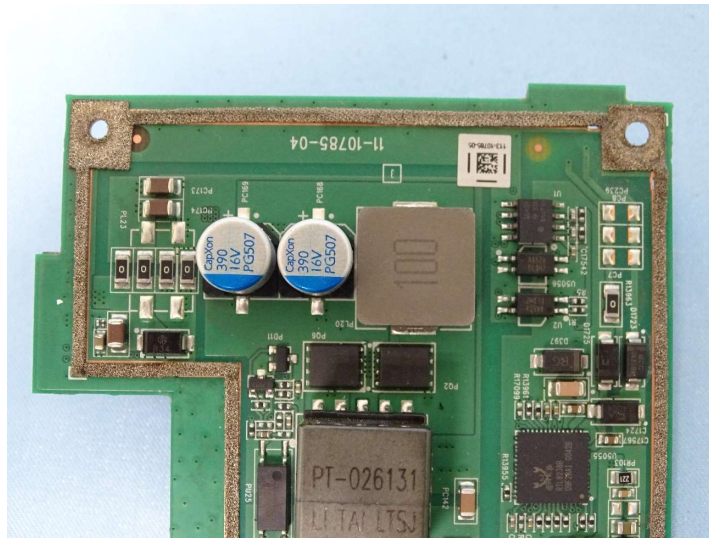
Photograph 9: Power Board PCB
