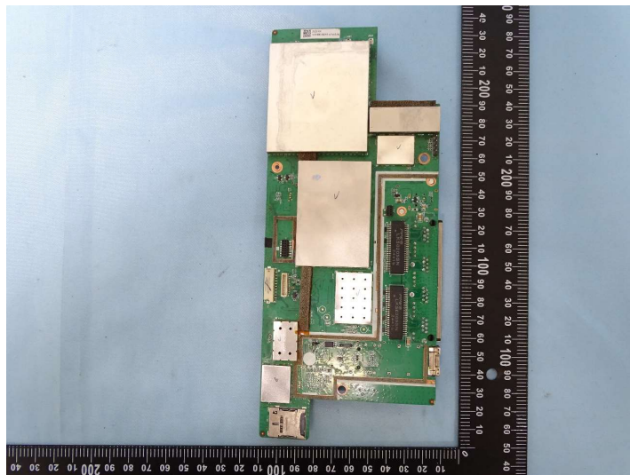
Photograph 31: Front of Main PCB
