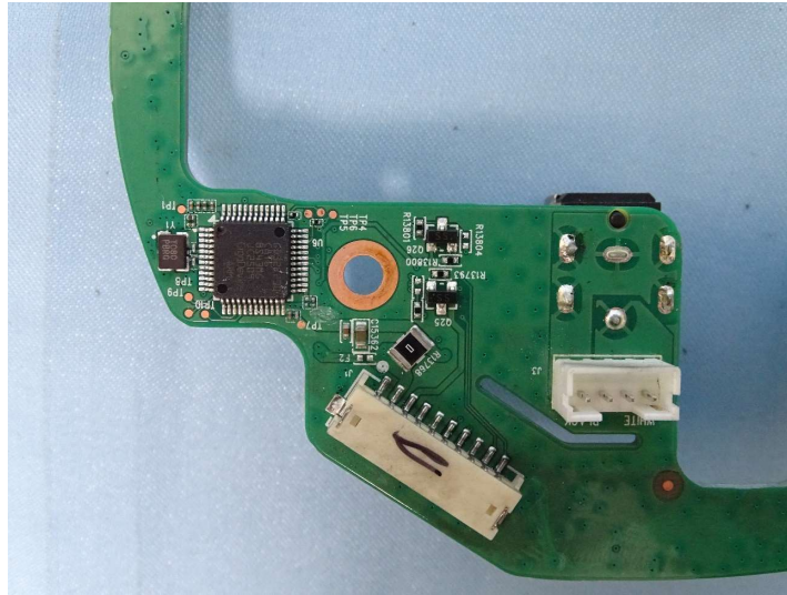
Photograph 25: LED PCB
