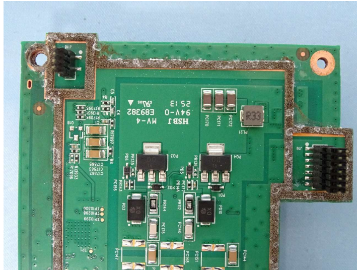
Photograph 13: Power Board PCB
