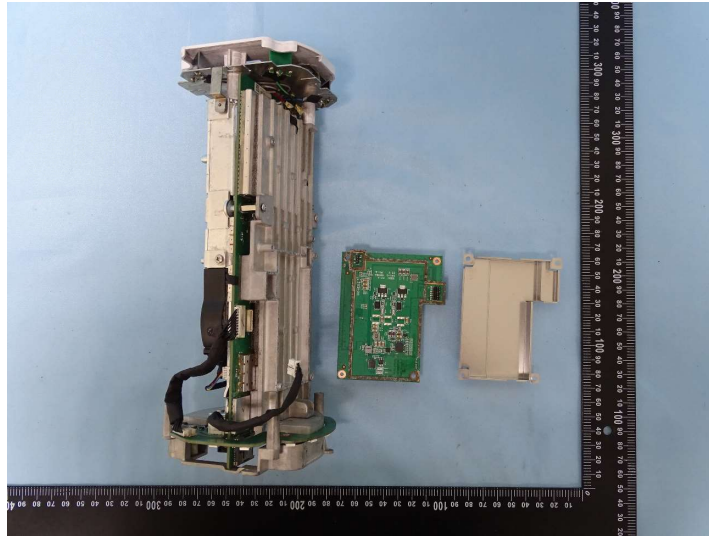
Photograph 7: Power Supply Board Removed
