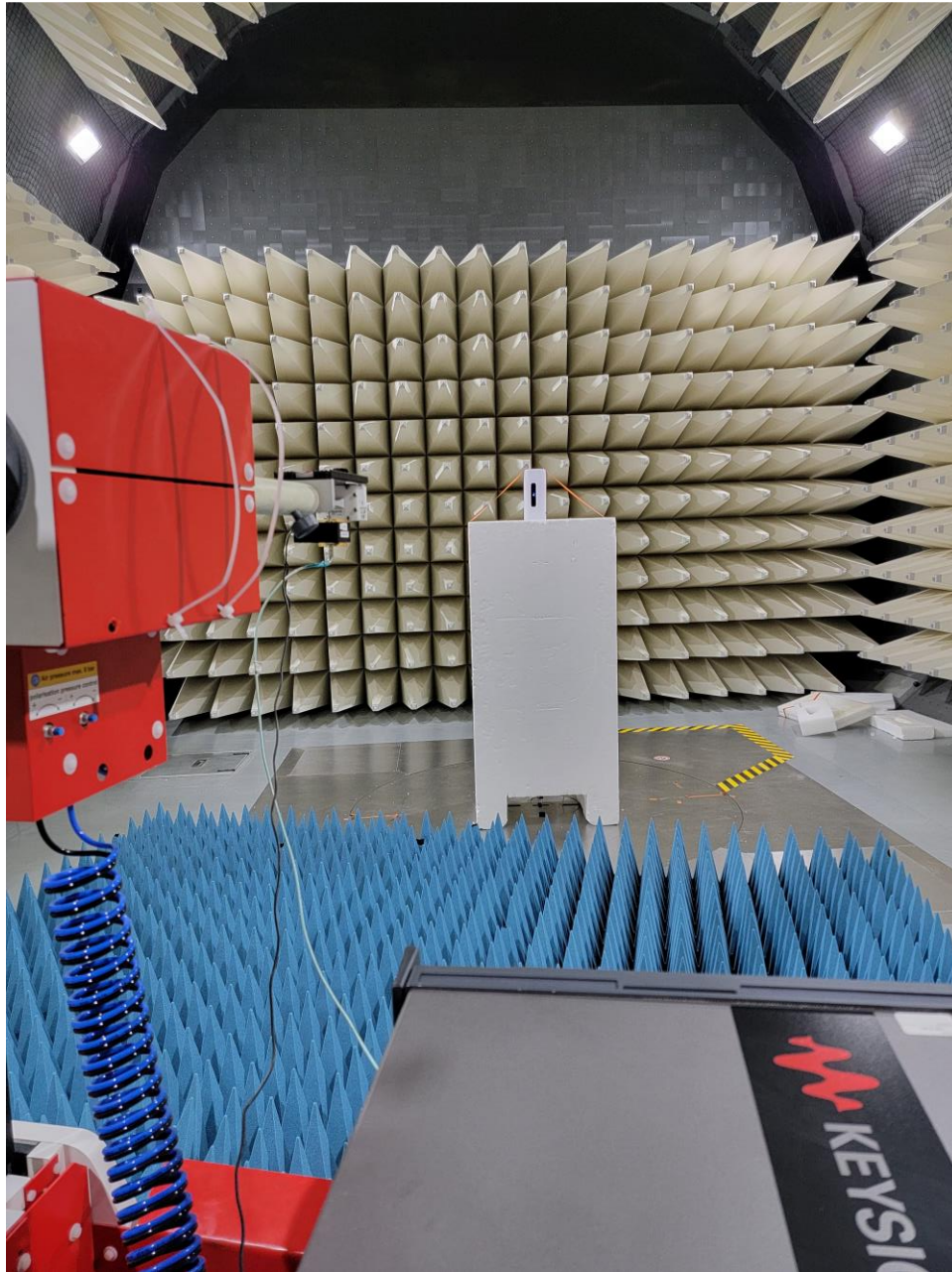
Photograph 3: View Test Set Up Radiated Emissions 17 – 40 GHz
