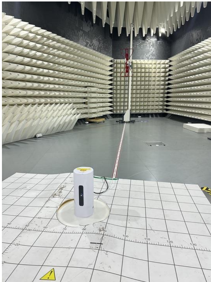
Photograph 1: View Test Set Up Radiated Emissions 30 – 1000 MHz
