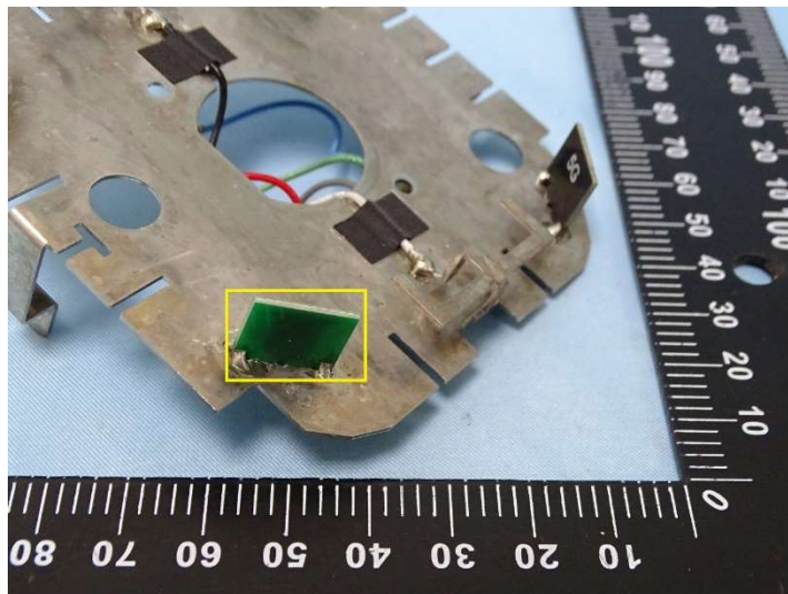
Photograph 9: 6 GHz WiFi 6G0 Antenna
