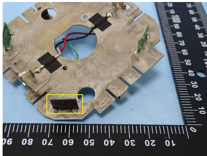
Photograph 8: 5 GHz WiFi 5G1 Antenna
