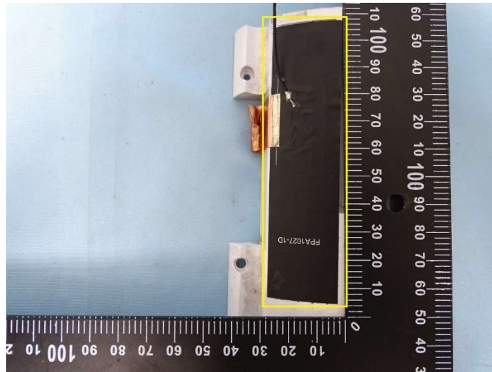
Photograph 11: WWAN Antenna 0
