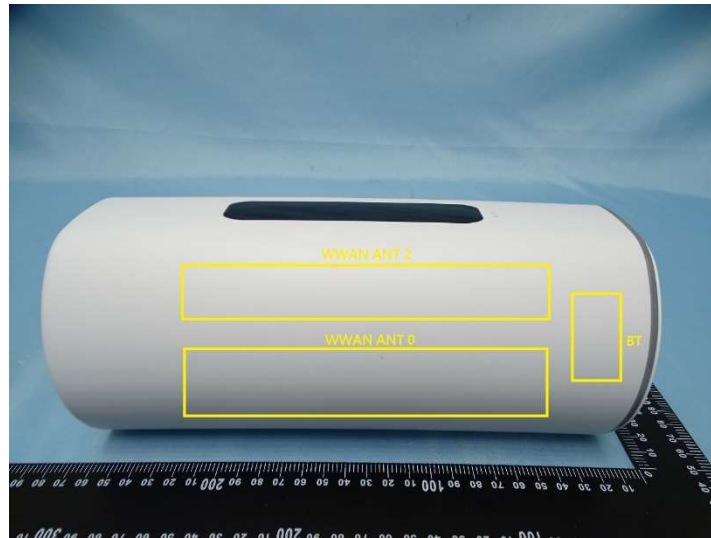
Photograph 3: Location of Antennas From the Outside
