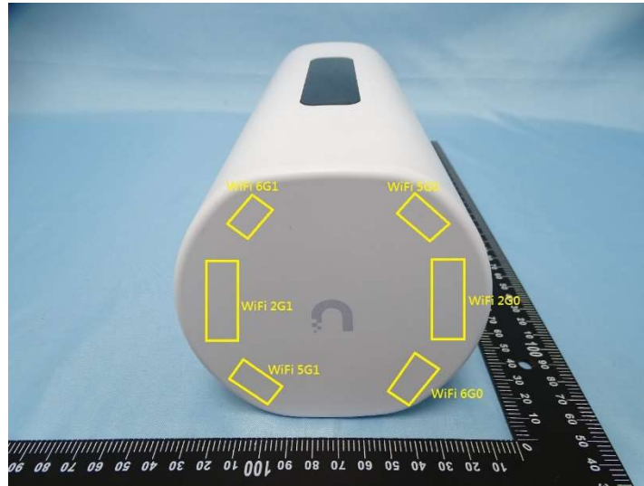
Photograph 1: Location of Antennas From the Outside
