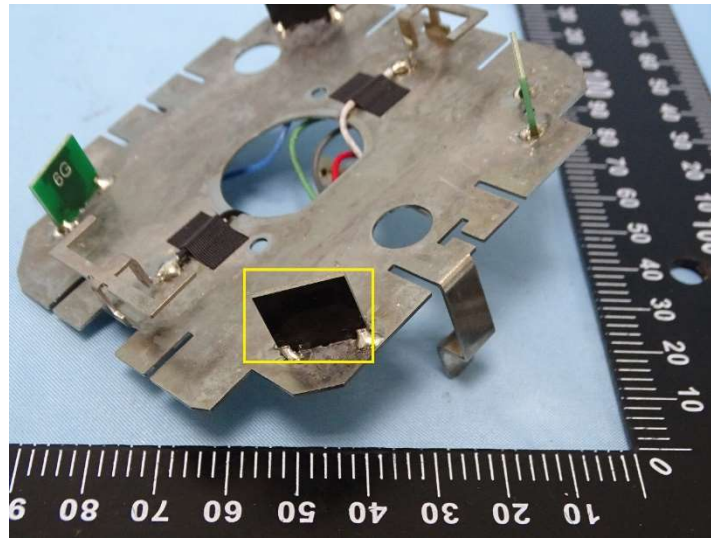
Photograph 7: 5 GHz WiFi 5G0 Antenna
