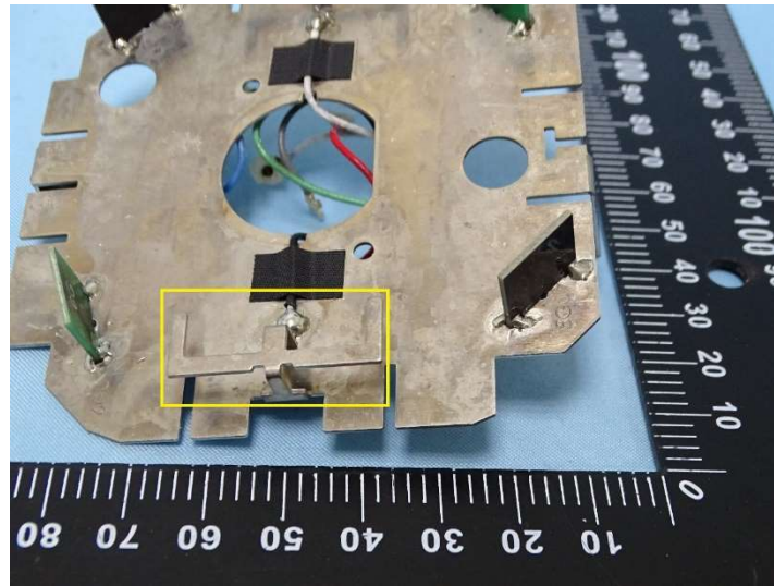
Photograph 5: 2.4 GHz WiFi 2G0 Antenna
