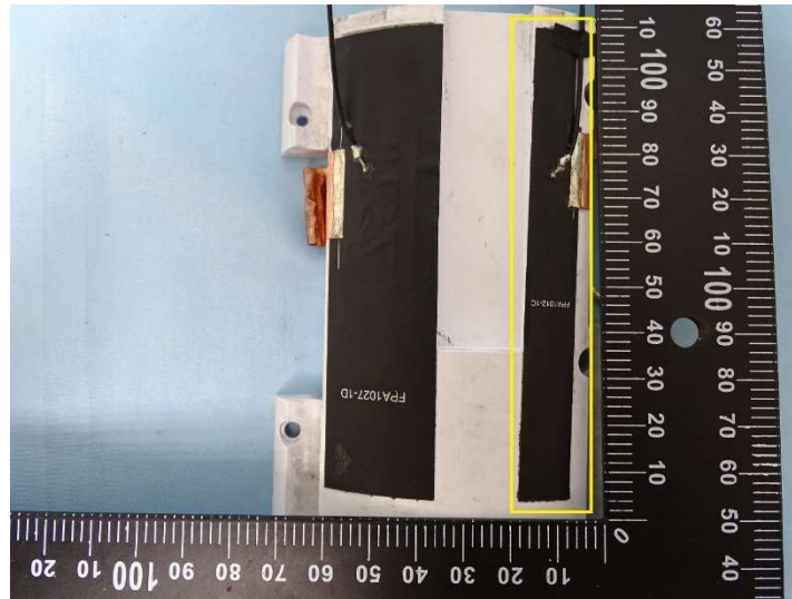
Photograph 13: WWAN Antenna 2
