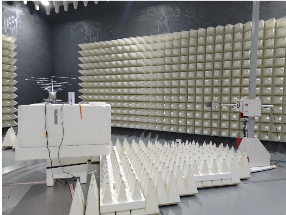
Photograph 4: Test Set Up Radiated Emissions 1 – 17 GHz (Colocation)
