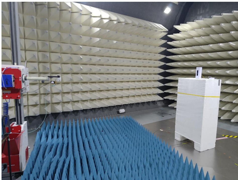
Photograph 5: Test Set Up Radiated Emissions 17 – 40 GHz (Colocation)
