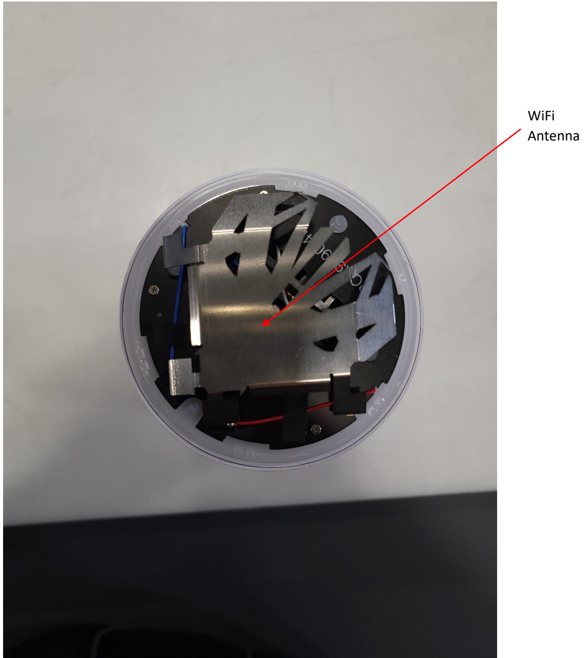
Photograph 1: Top of DUT w/Cover Off
