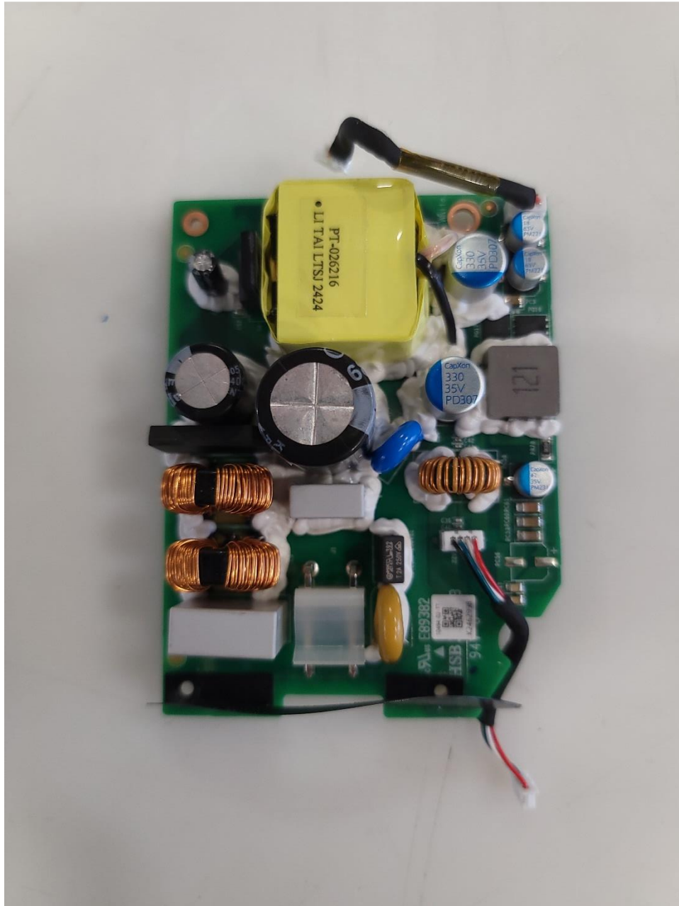
Photograph 14: Main Power Board Front
