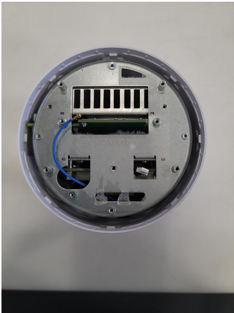
Photograph 5: Top of DUT w/ Antenna Board & Tape Off
