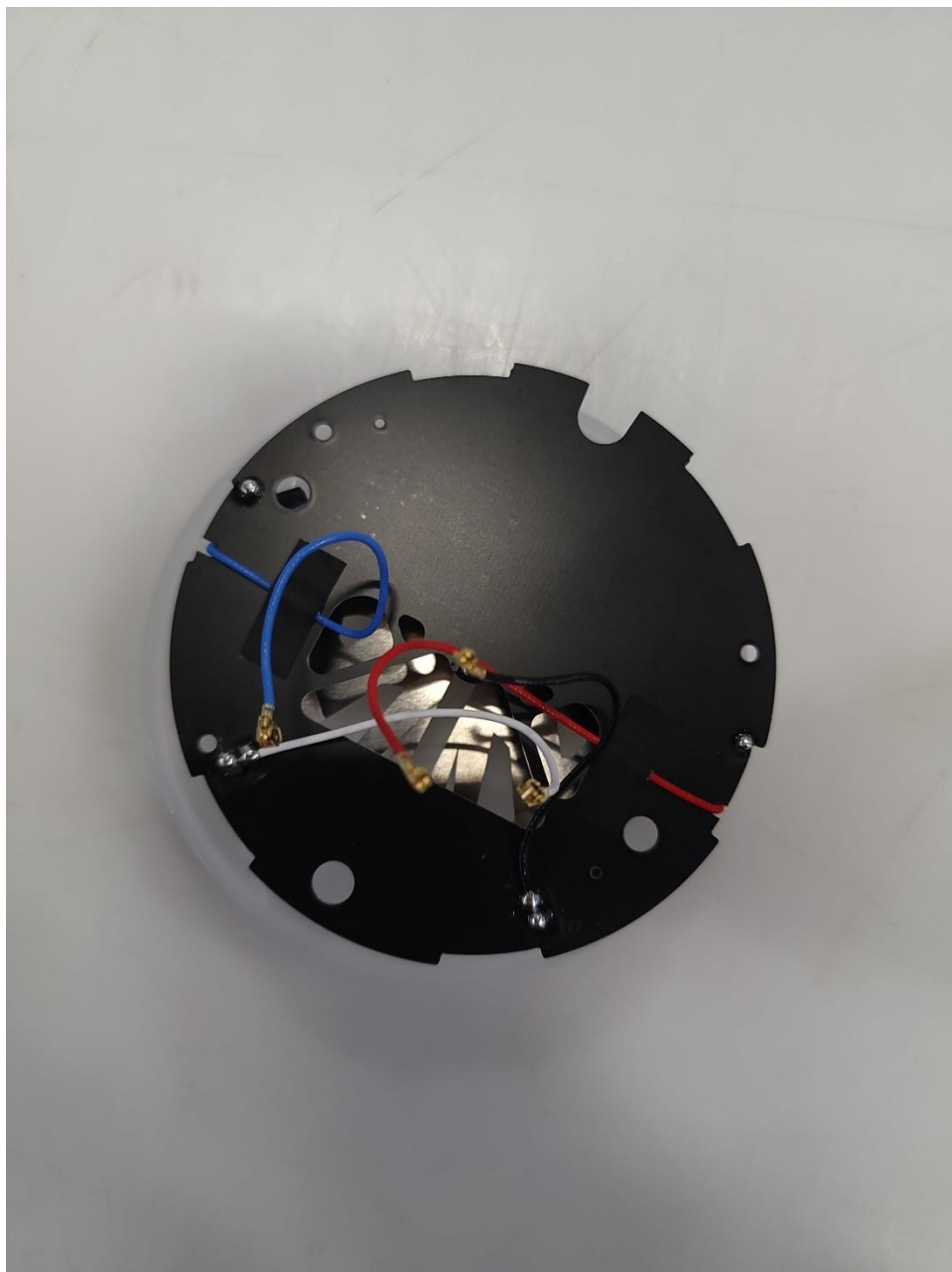
Photograph 3: Back of Antenna Board
