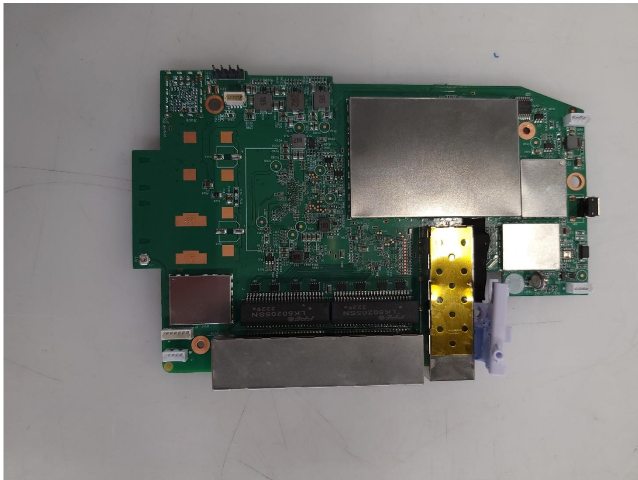
Photograph 16: Main PCB Front w/Cans
