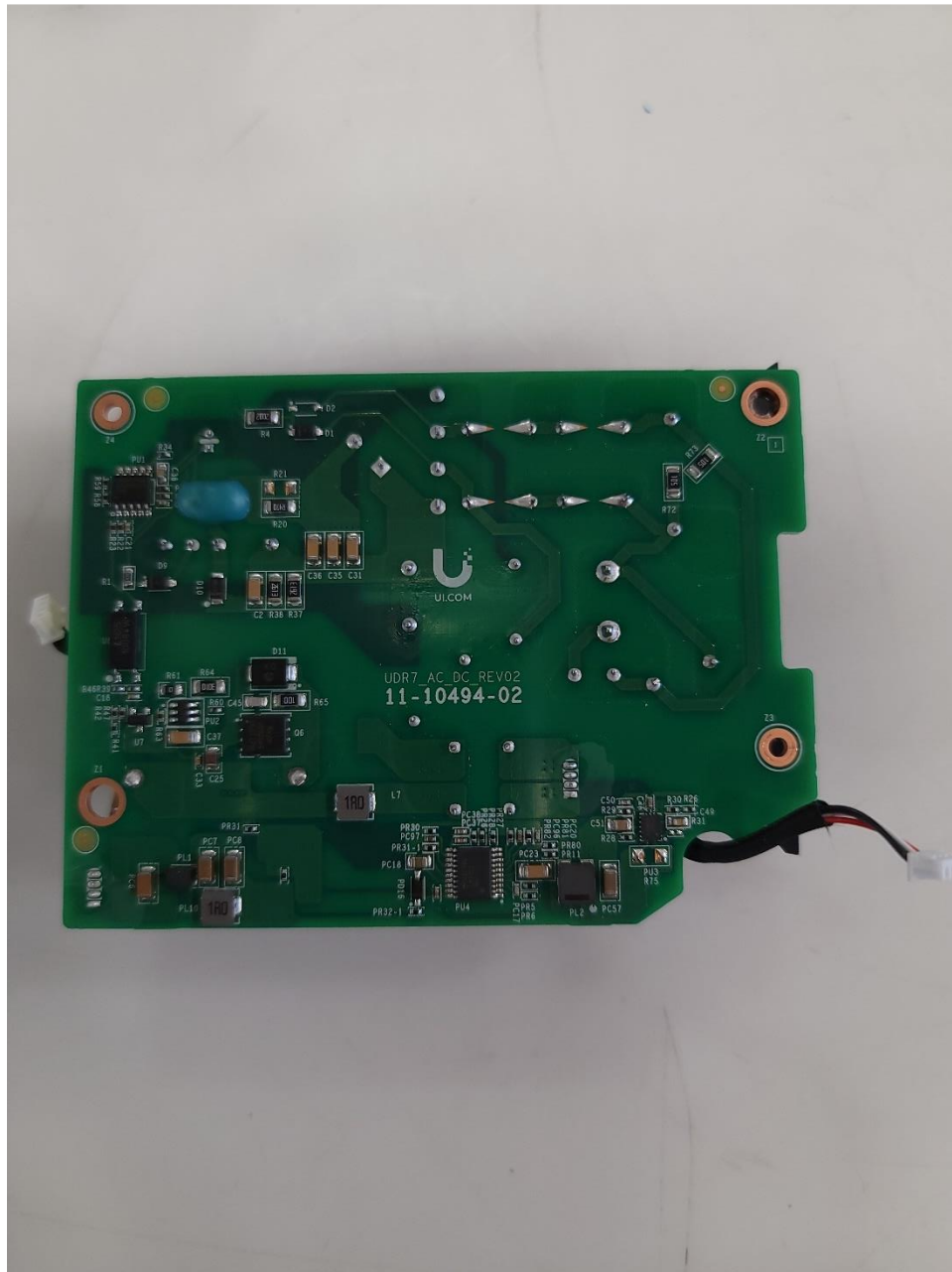
Photograph 15: Main Power Board Back
