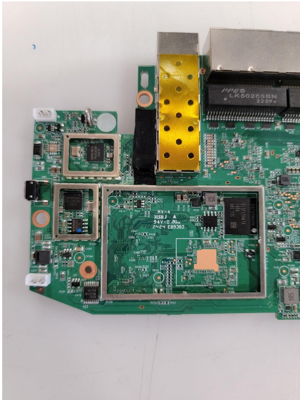
Photograph 19: Main PCB Front Close Up
