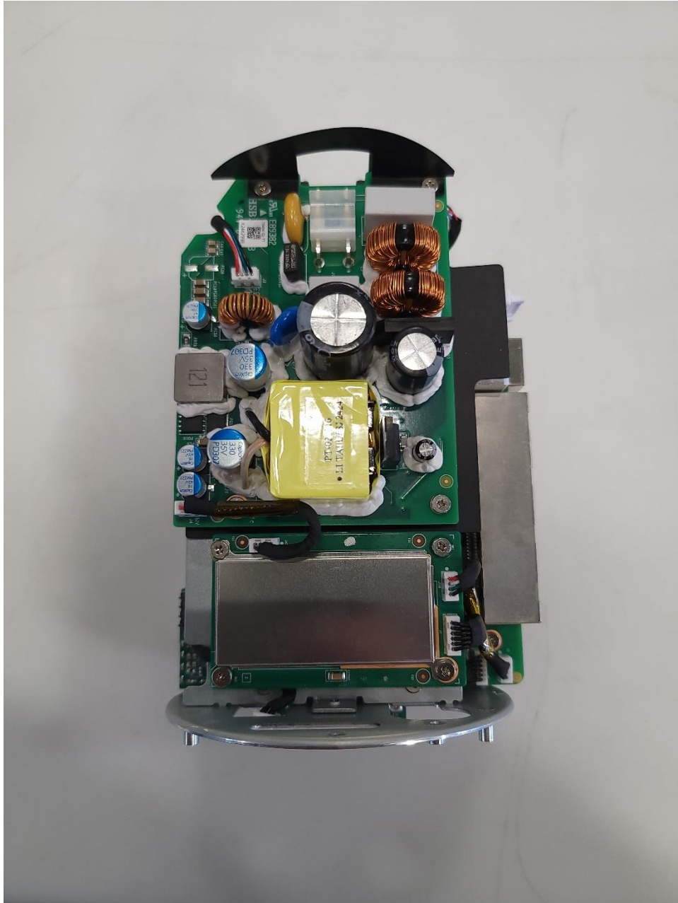
Photograph 9: DUT Front Side
