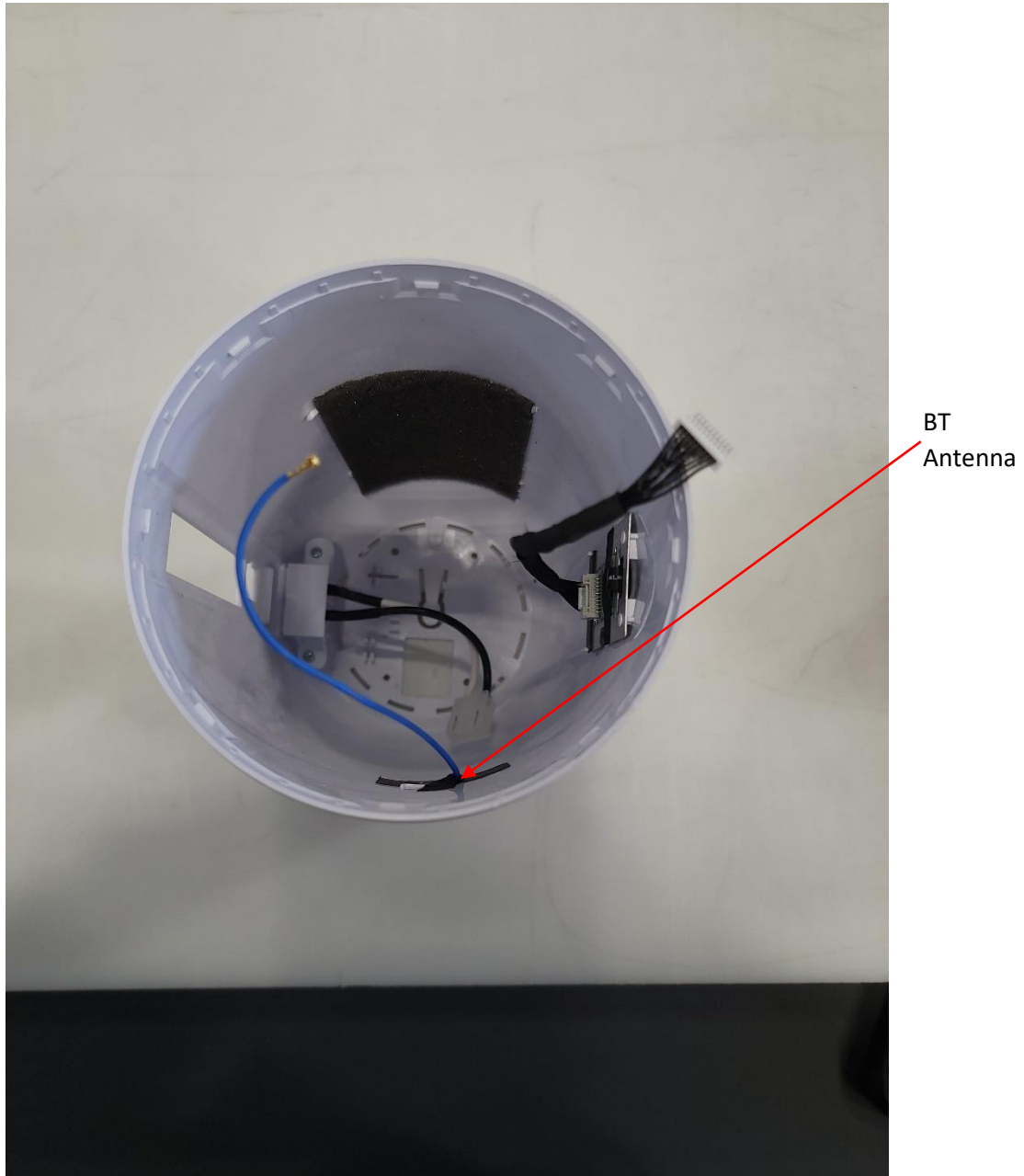
Photograph 6: Inside of DUT Outer Shell
