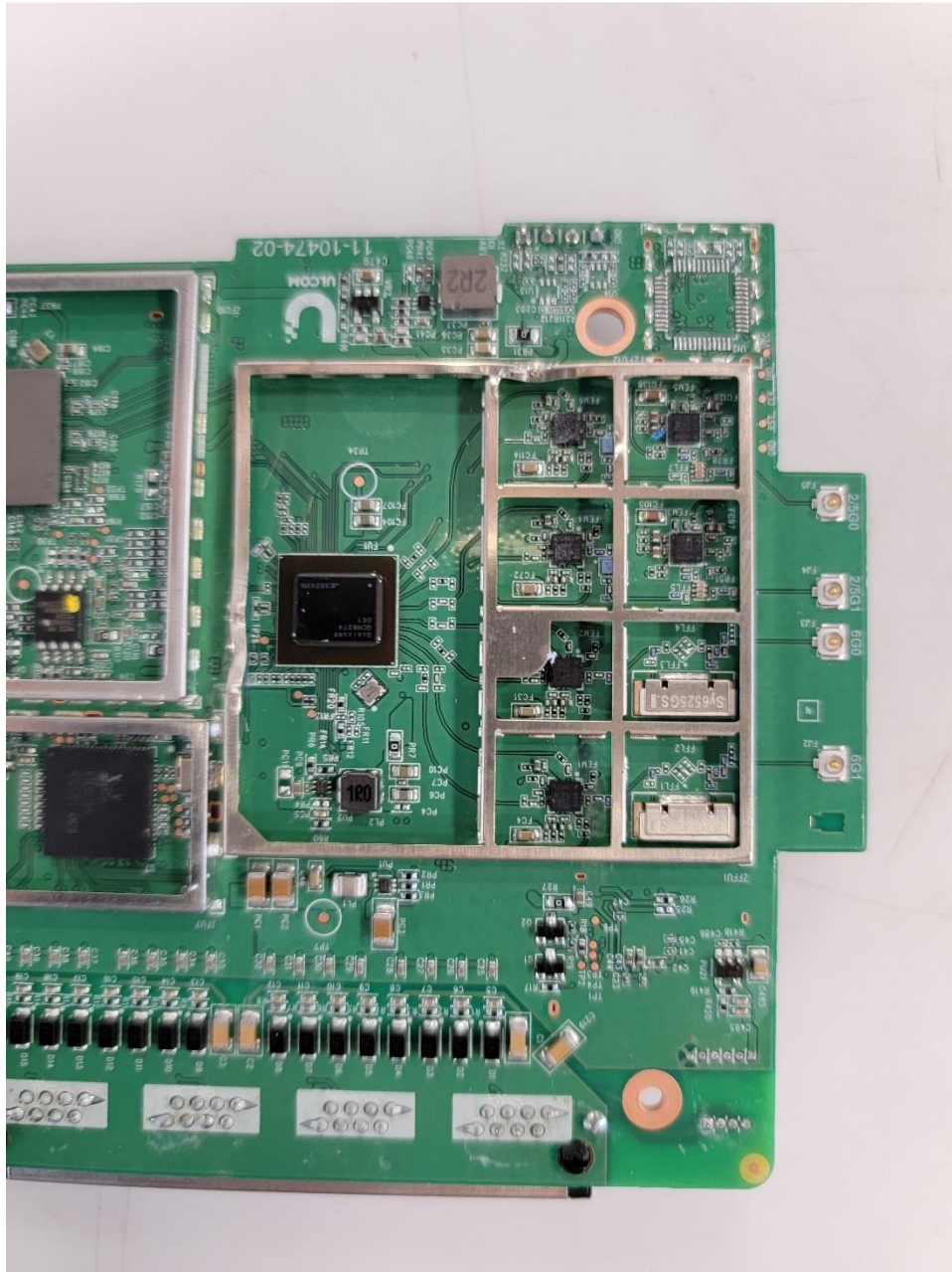
Photograph 22: Main PCB Back Close Up
