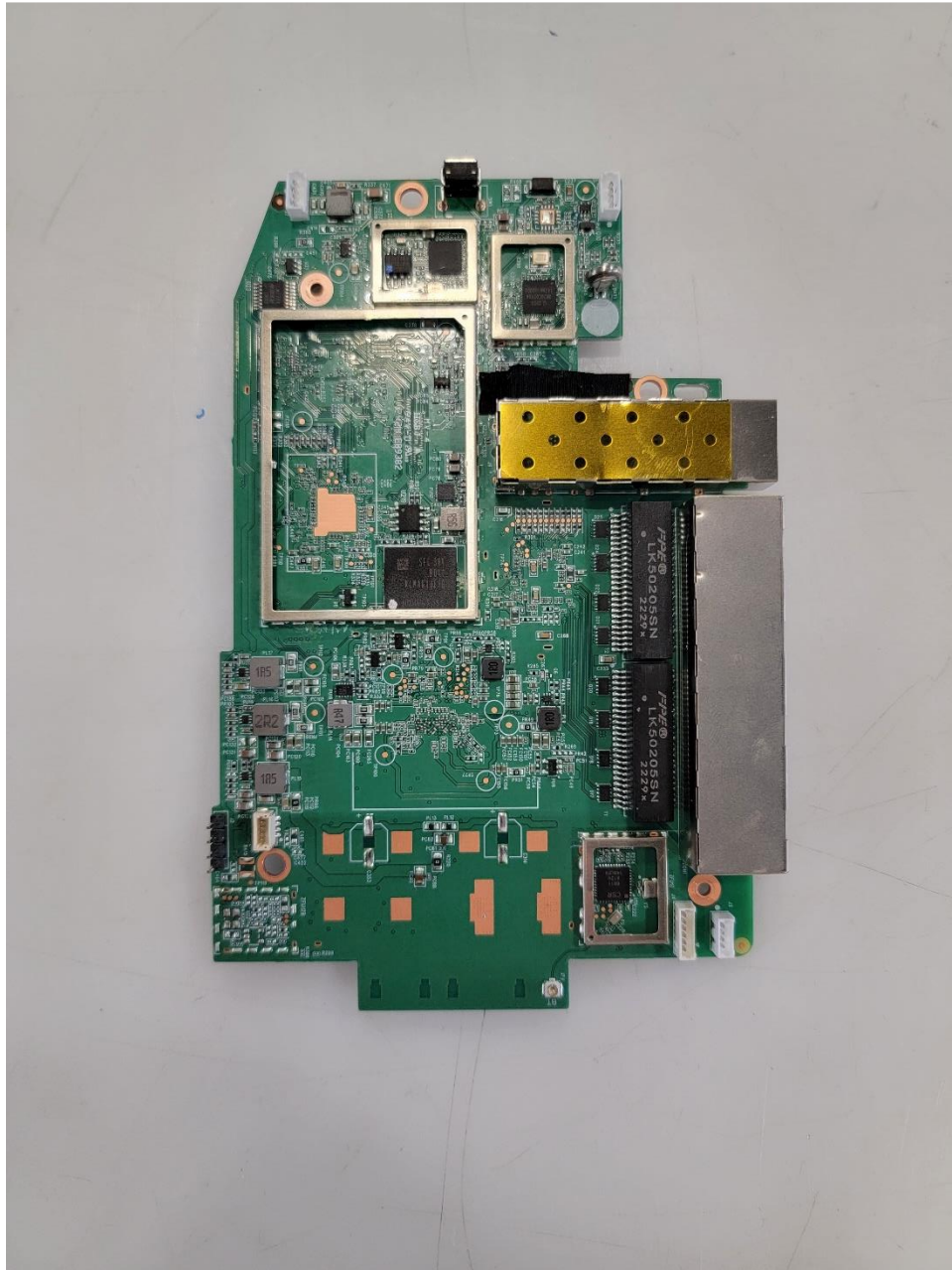
Photograph 17: Main PCB Front w/Cans Off
