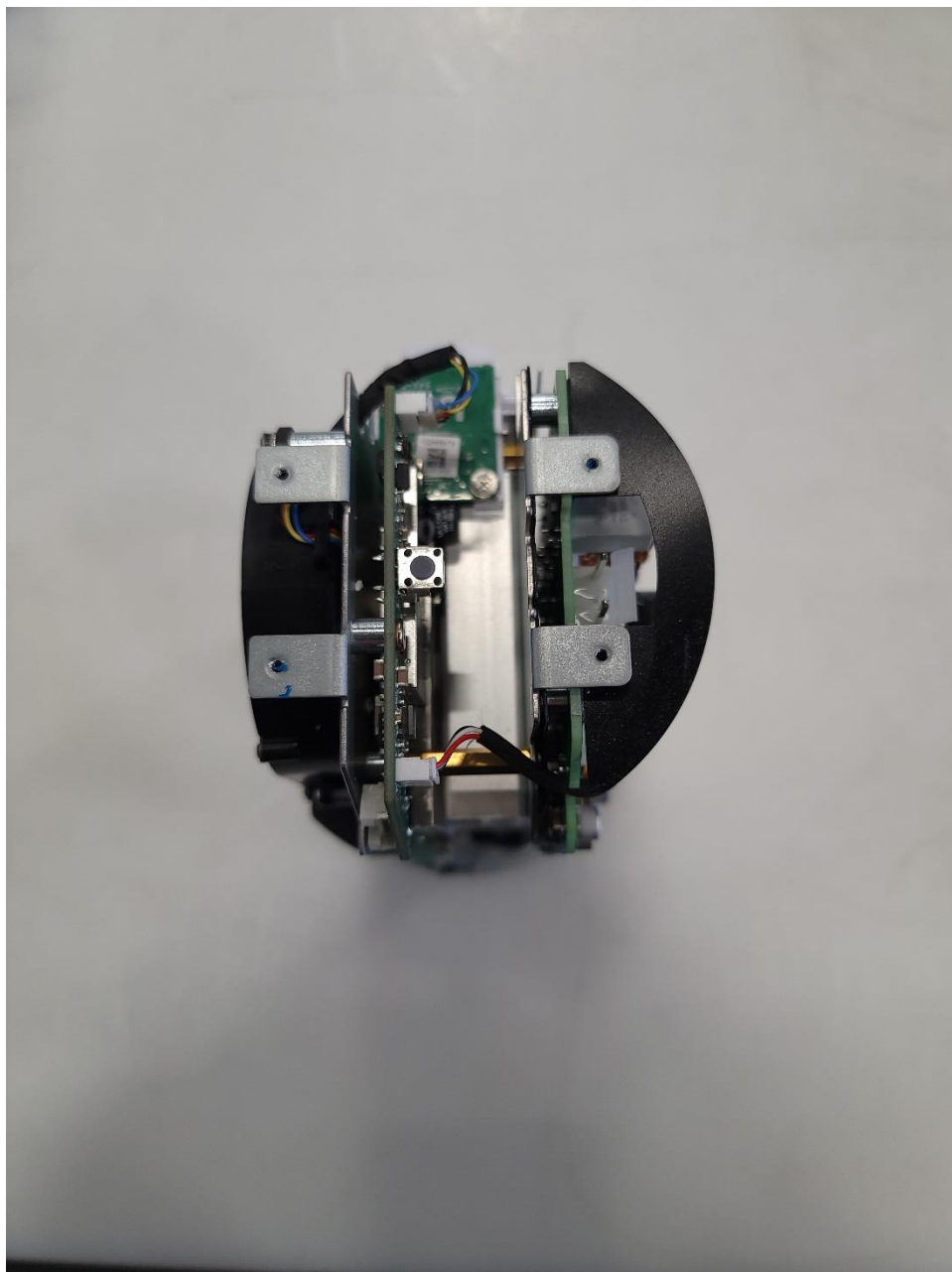
Photograph 7: Top of DUT Outside Cover Off
