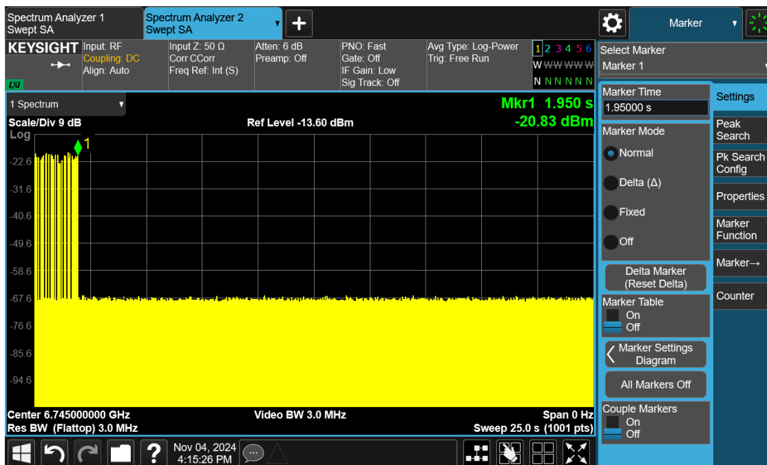
Plot 9: AWGN Signal Detection 320MHz
