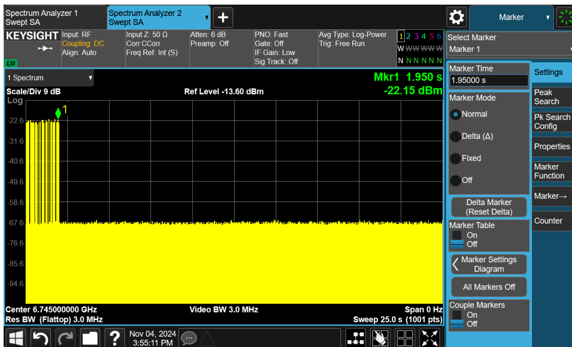
Plot 11: AWGN Signal Detection 320MHz
