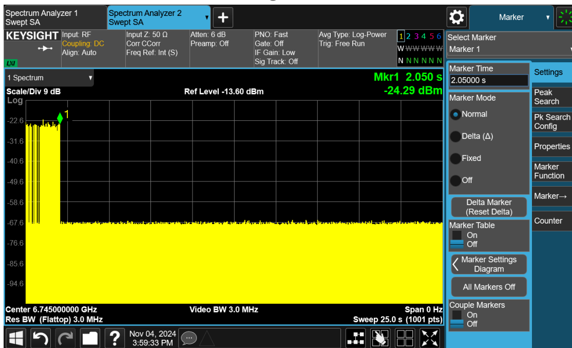
Plot 10: AWGN Signal Detection 320MHz
