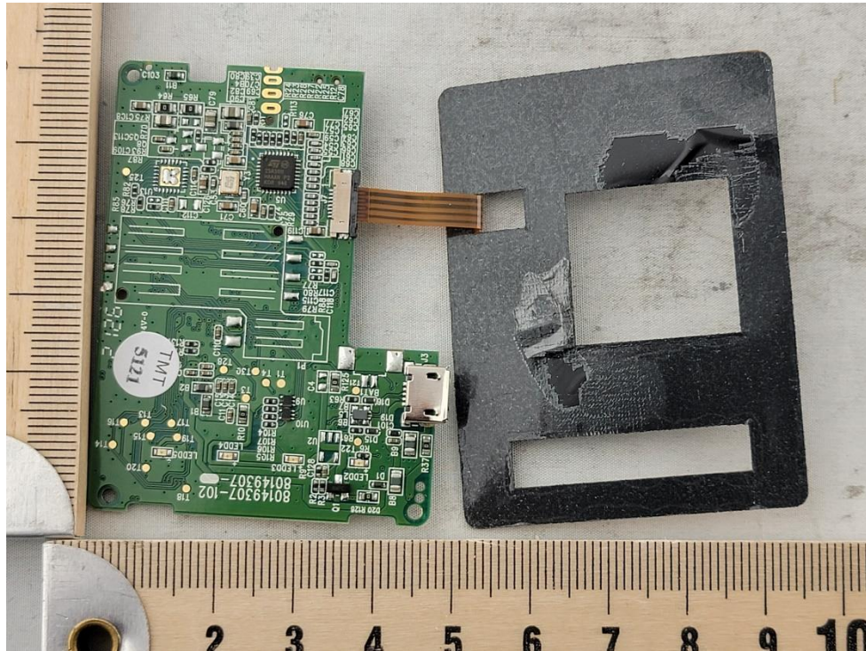
Photograph 3: Internal View of DUT
