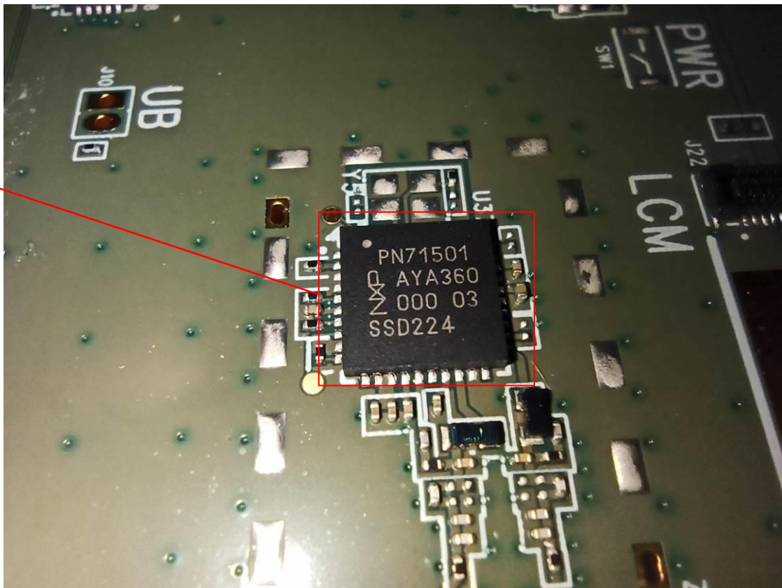
RF Chip A (For NFC)
