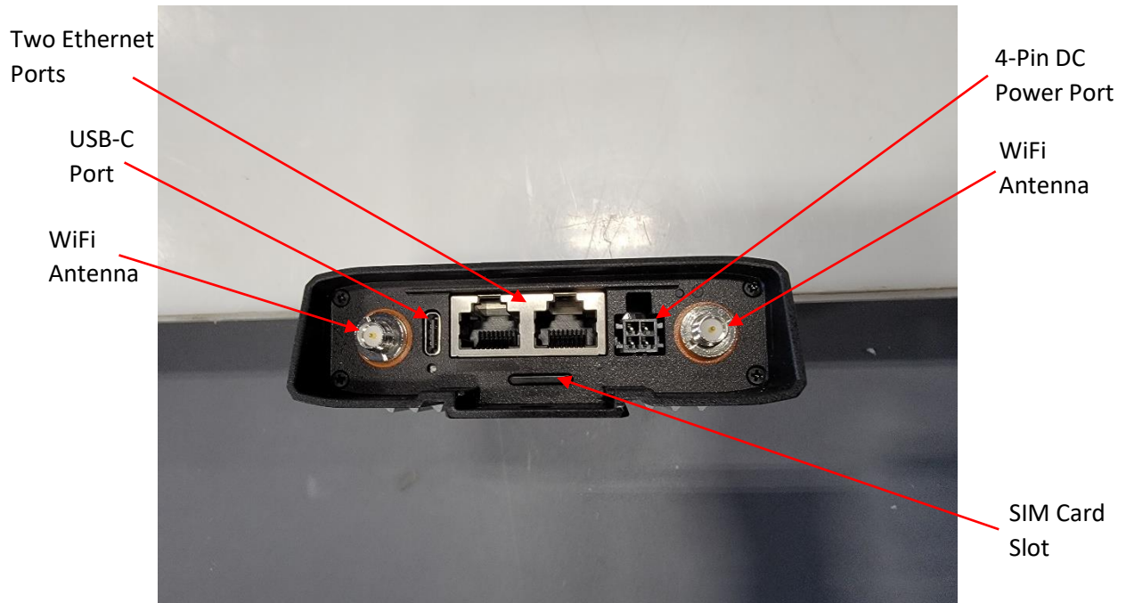
Photograph 9: Bottom View of DUT Close Up Showing Ports
