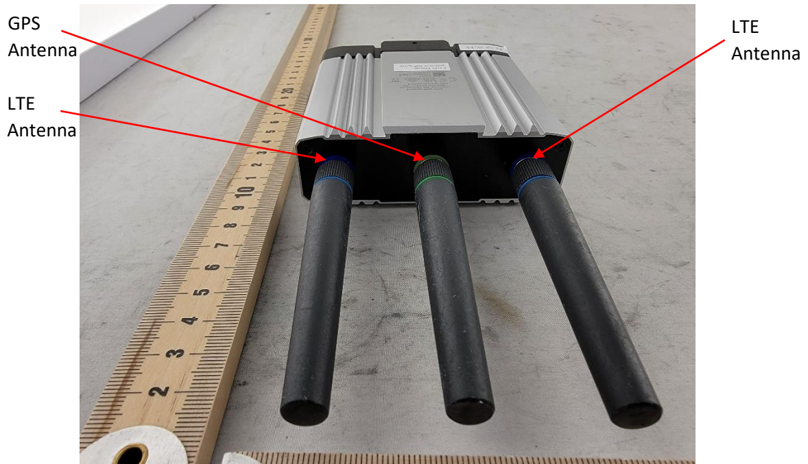
Photograph 7: Top View of DUT
