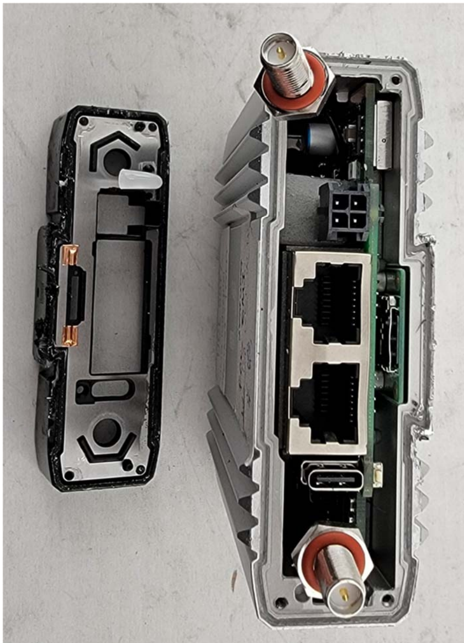
Photograph 1: Cover Off of Bottom of DUT
