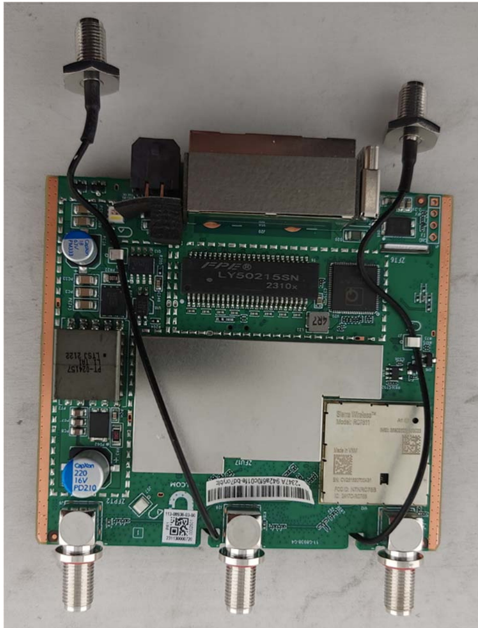
Photograph 2: Internal View of DUT – Top of PCB With Can On
