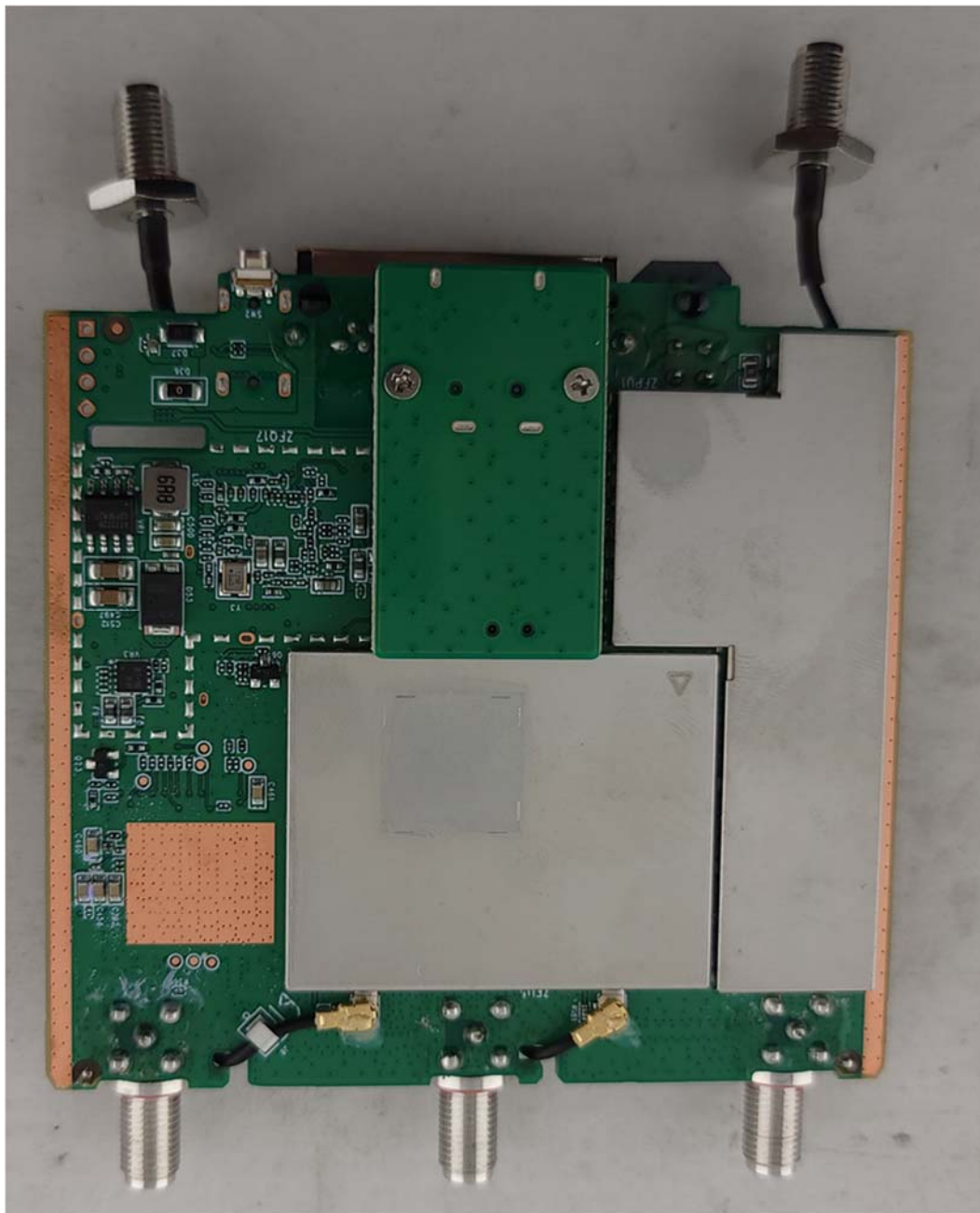
Photograph 2: Internal View of DUT – Bottom of PCB With Metal Removed and Cans On
