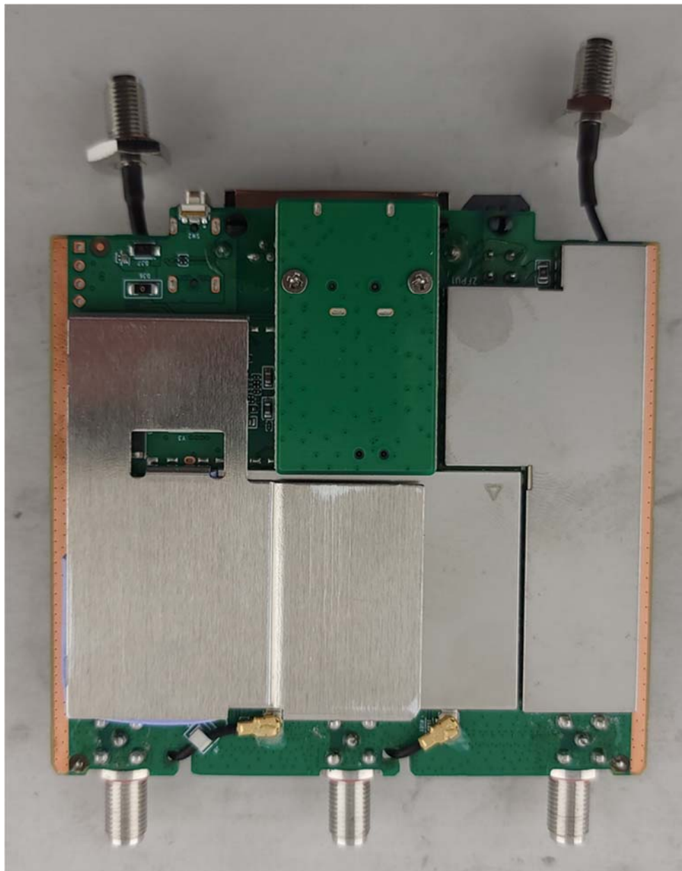
Photograph 1: Internal View of DUT – Bottom of PCB With Metal and Cans On
