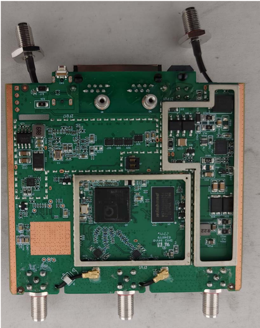
Photograph 3: Internal View of DUT – Bottom of PCB With Metal and Cans Off
