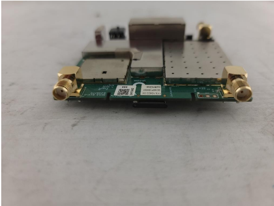
Photograph 1: Cover Off of Top of DUT
