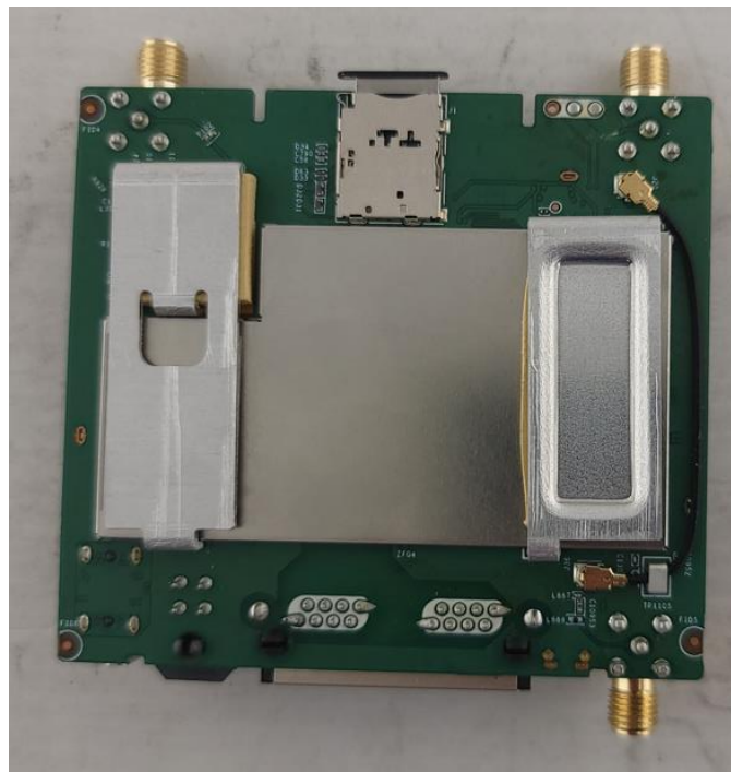
Photograph 4: Internal View of DUT – Bottom of PCB With Metal and Cans On
