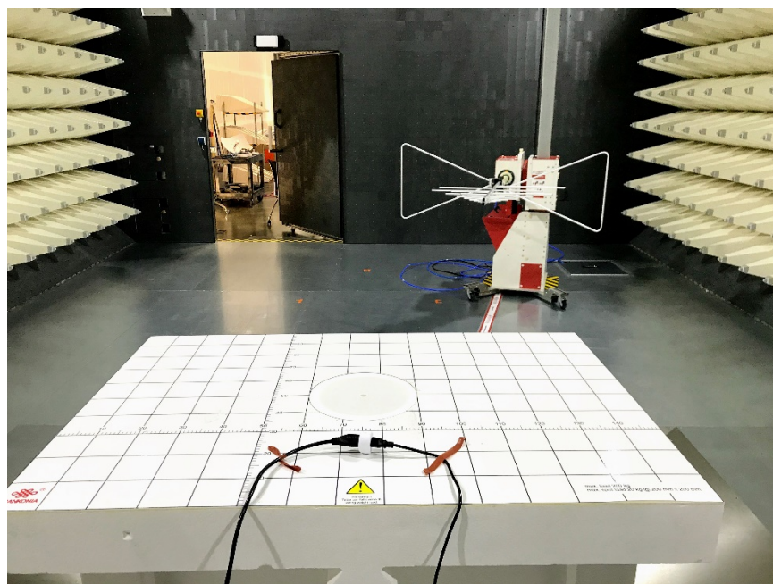
Radiated Below 1 Ghz
