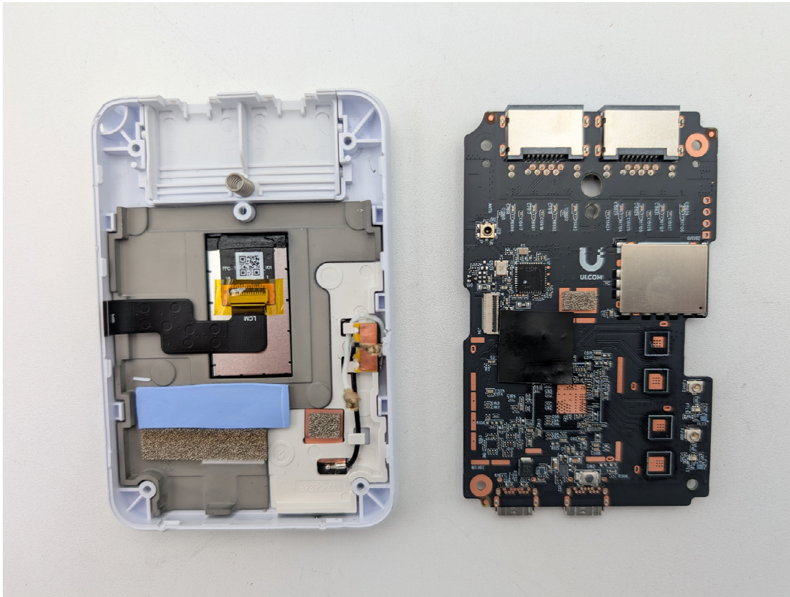
Photograph 1: PCB Out of Front Housing
