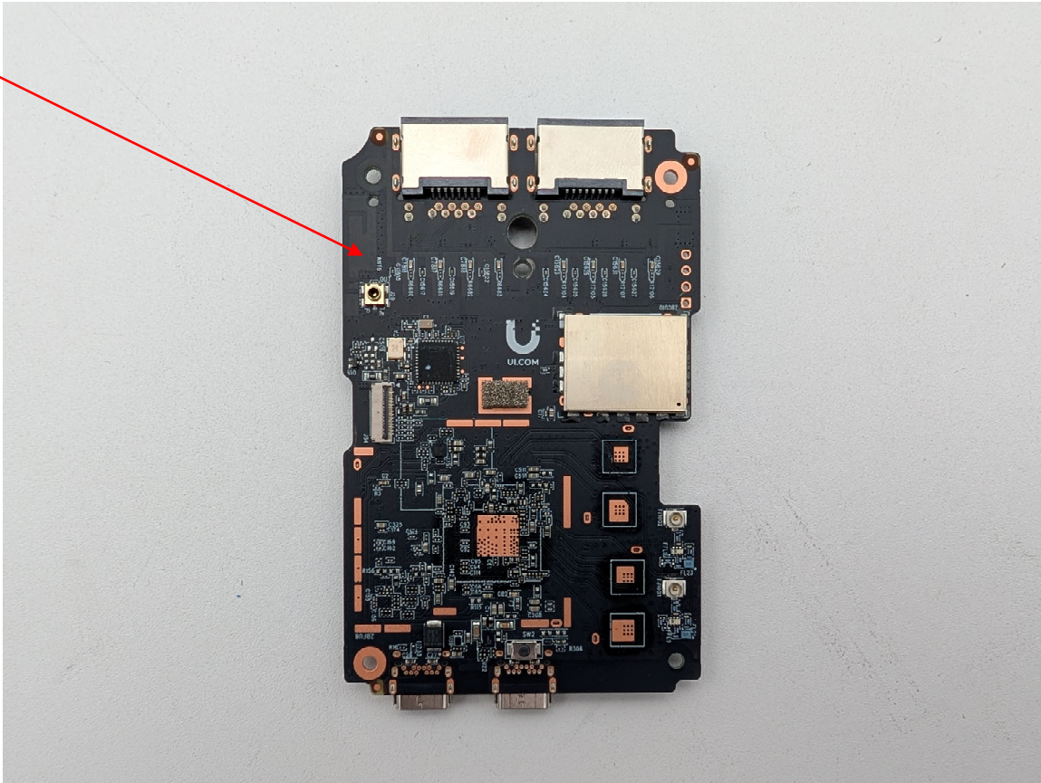
Photograph 1: Back of PCB w/Cans On
