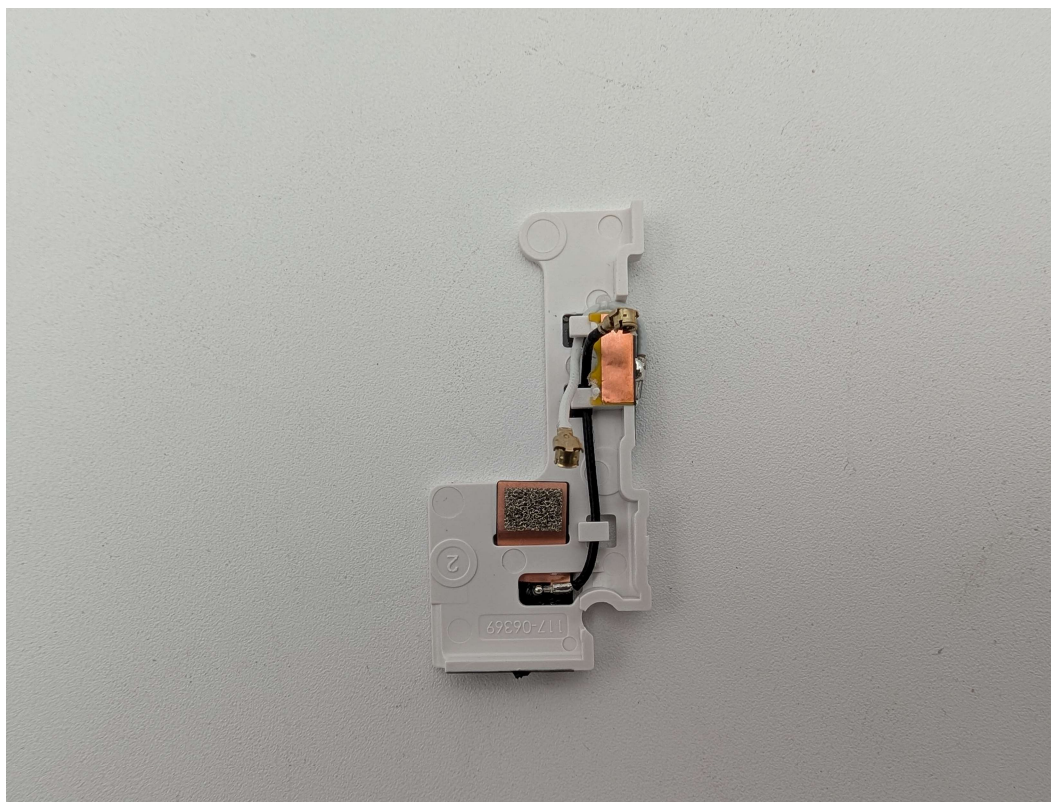
Photograph 1: Back Side of Antenna Board
