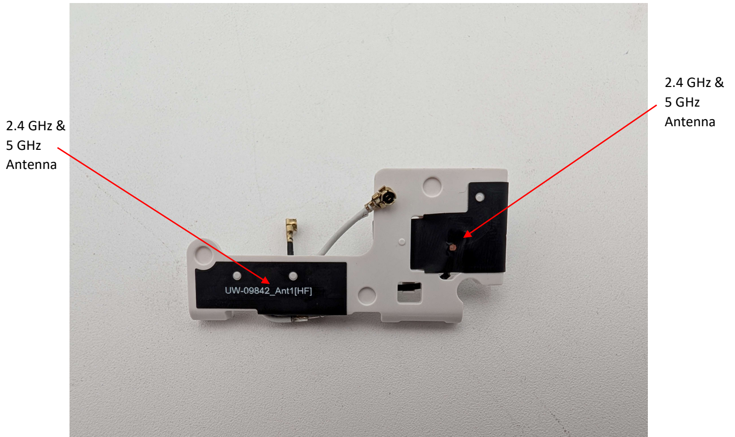
Photograph 2: Front Side of Antenna Board
