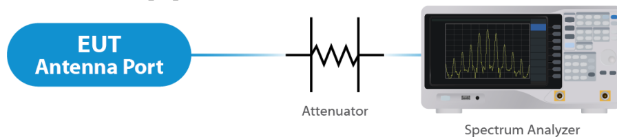
Figure 2: Direct Connect at the Antenna Port Test
