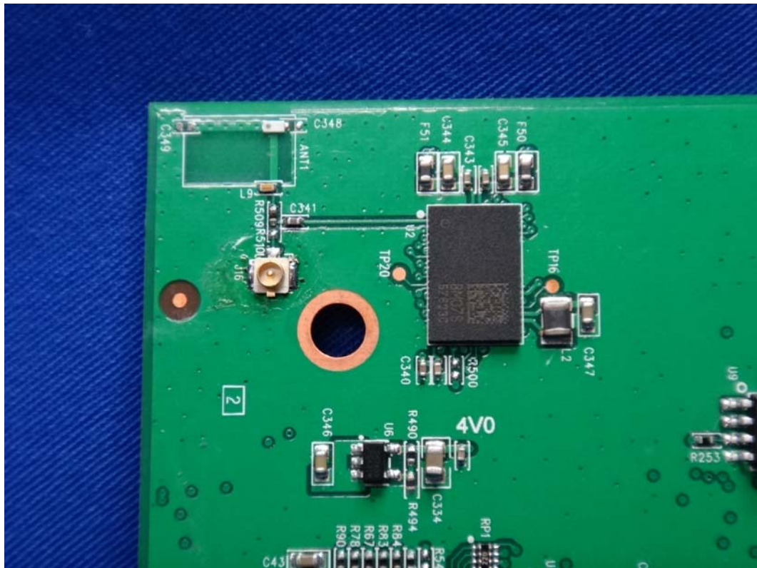
(22) EUT Photo-RF Chip &amp; Chip Antenna
