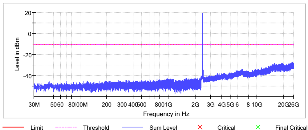
Graph 2: B- Mode 20MHz Middle Conducted Spurious Plot
