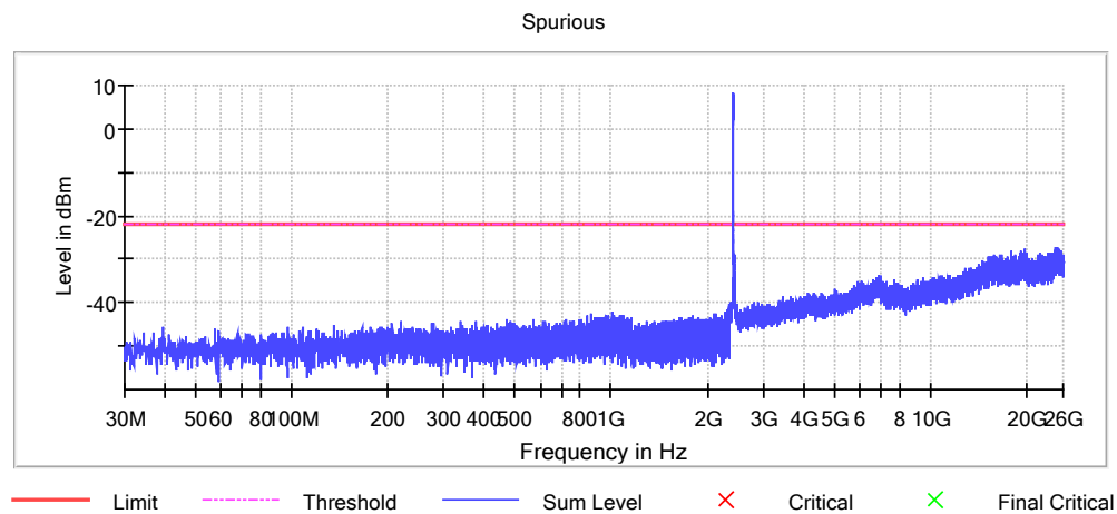
Graph 13: AX- z Mode 20MHz Lower Conducted Spurious Plot
