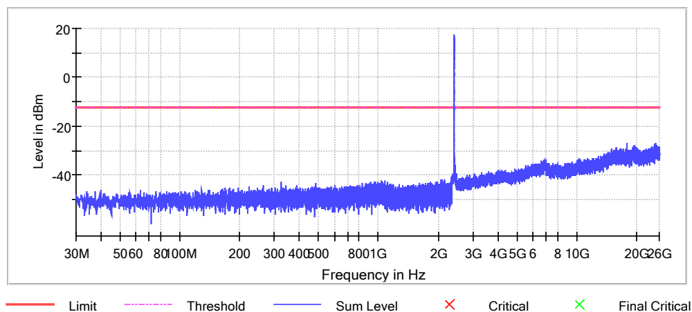
Graph 1: B- Mode 20MHz Lower Conducted Spurious Plot
