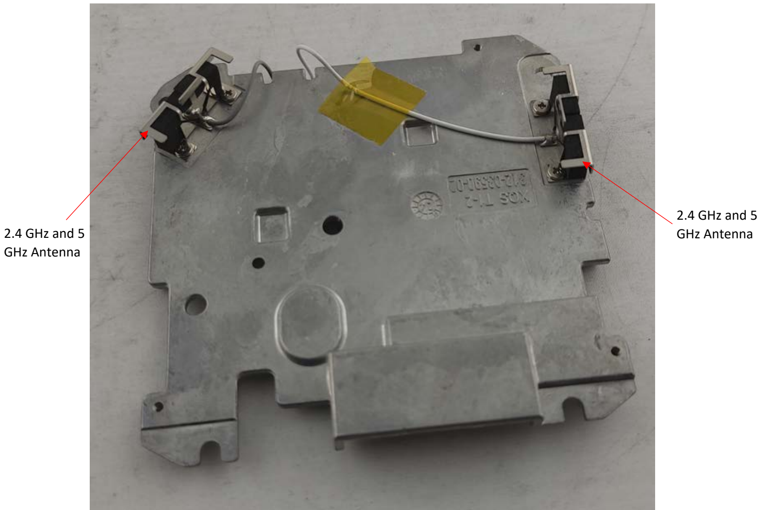
Photograph 8: Top Side of Heat Sink/Antenna Mount Showing 2.4/5 GHz Antennas
