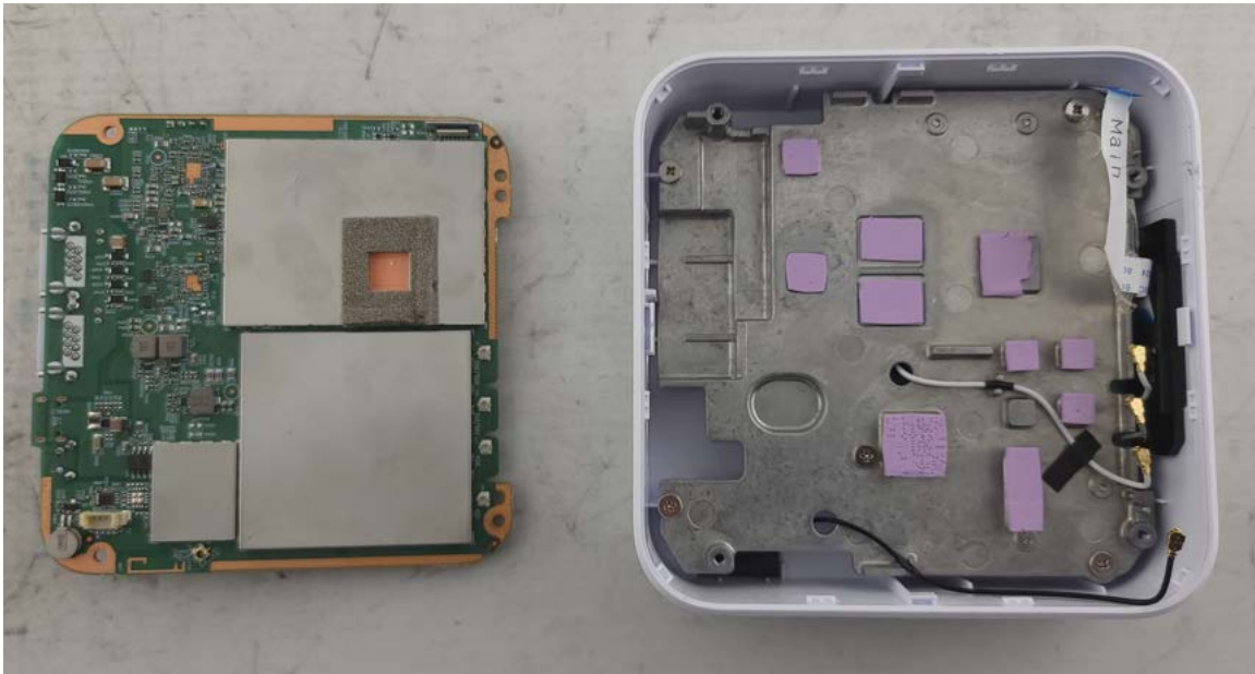
Photograph 4: Top of DUT with Main PCB Removed
