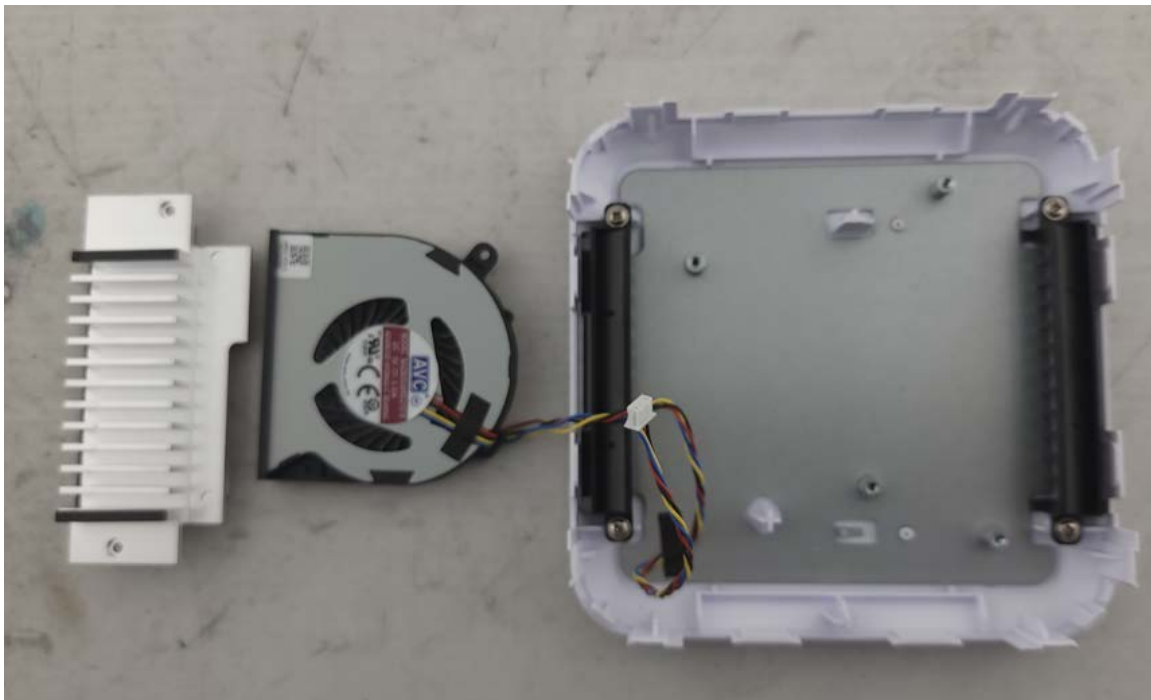
Photograph 2: Internal View Bottom of DUT with Fan and Heat Sink Removed
