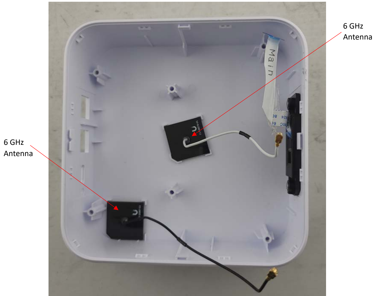
Photograph 6: Top Inside View of DUT Showing 6 GHz Antennas
