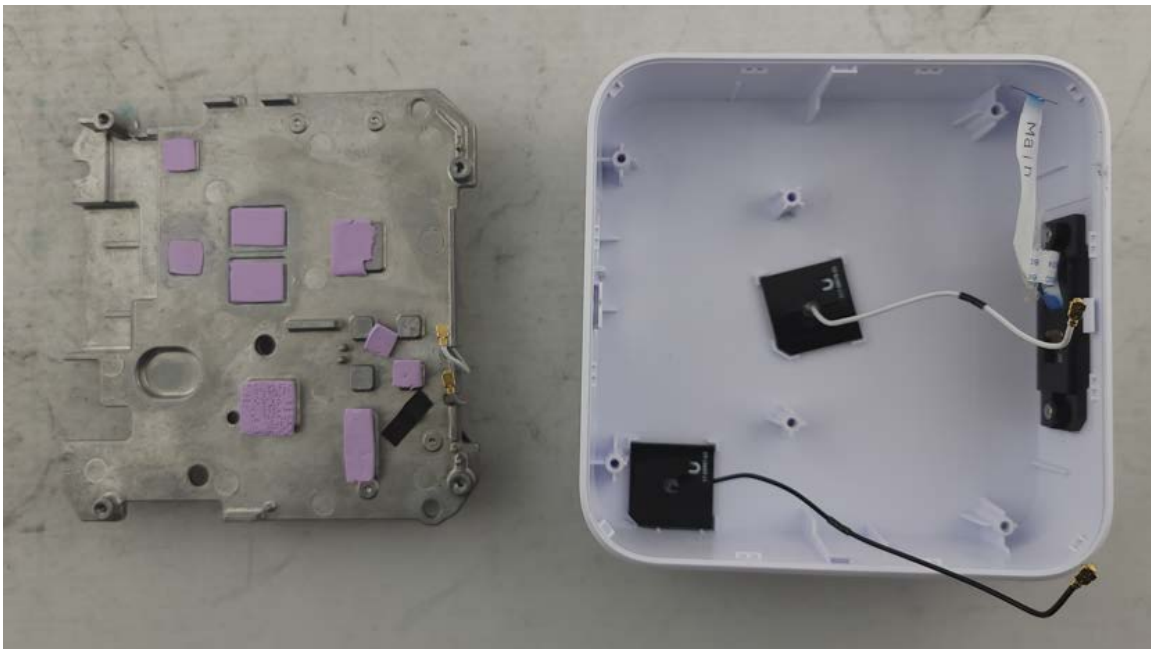
Photograph 5: Top of DUT with Heat Sink/Antenna Mount Removed
