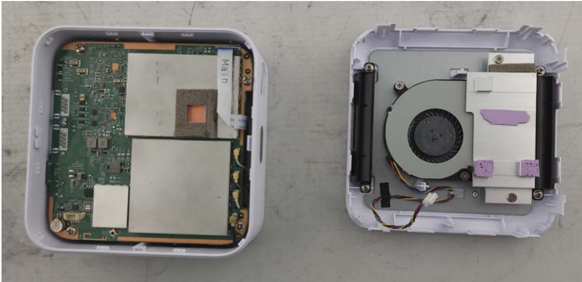
Photograph 1: Internal View with Bottom Piece Removed
