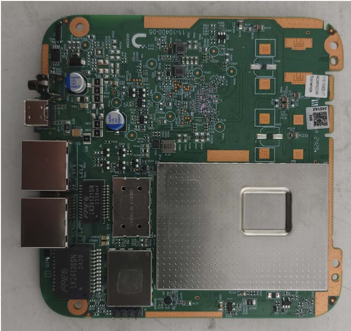
Photograph 2: Top Side Of Main PCB with Cans On
