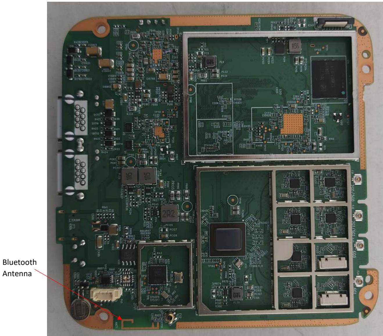
Photograph 3: Bottom Side of Main PCB with Cans Off
