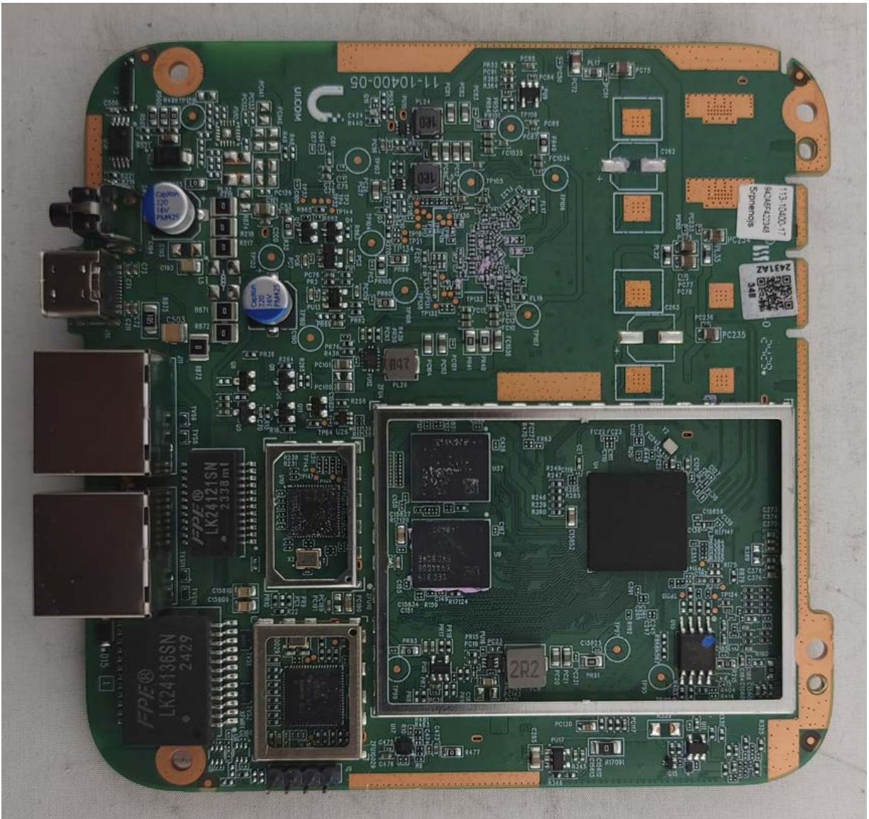
Photograph 4: Top Side Of Main PCB with Cans Off
