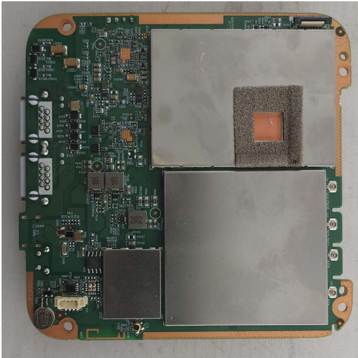
Photograph 1: Bottom Side of Main PCB with Cans On
