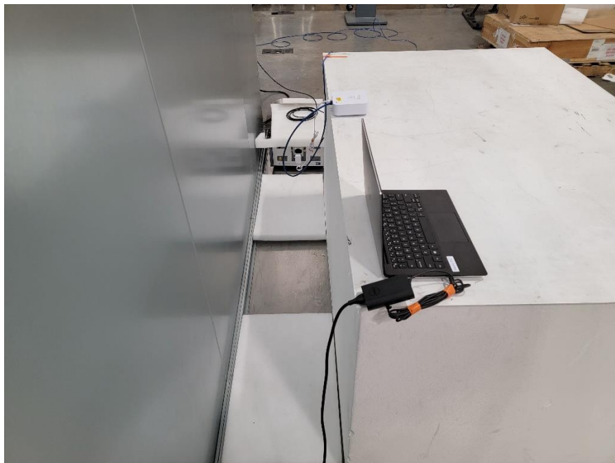
Photograph 7: View Test Set Up Back Conducted Emissions
