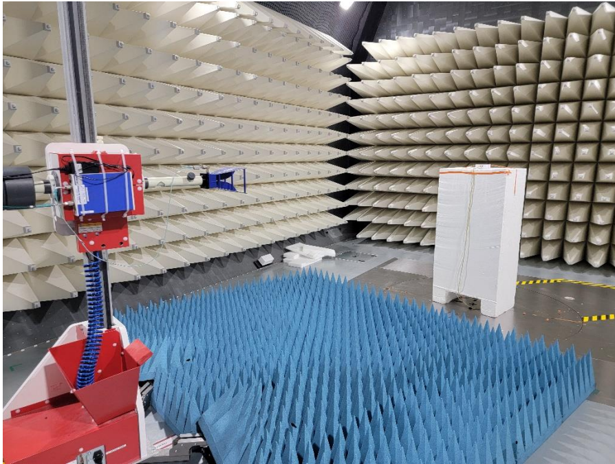
Photograph 3: View Test Set Up Radiated Emissions 17 – 40 GHz
