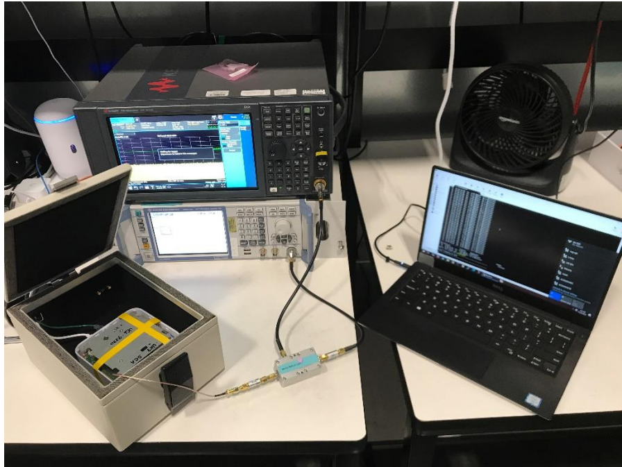
Photograph 5: View Test Set Up DFS
